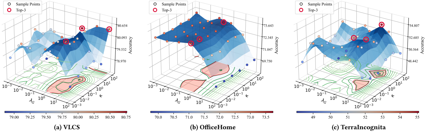
Figure 5: Additional performance comparison results with respect to variations in \kappa and \lambda_G .
