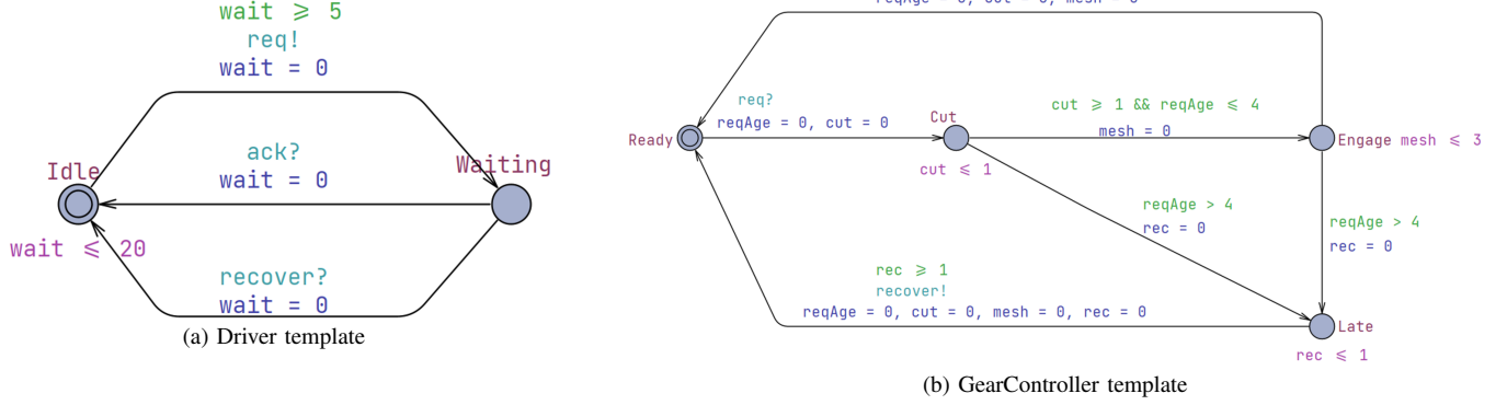
Fig. 1. A simplified network timed automaton for a cyclic automotive gear-shift controller. The faulty model uses cut \leq 1 , cut \geq 1 , mesh \leq 3 , and mesh \geq 3 . A repair that changes only the cut bounds blocks the early-engagement trace but can violate the response-deadline property; a multi-property repair also changes the mesh bounds.
