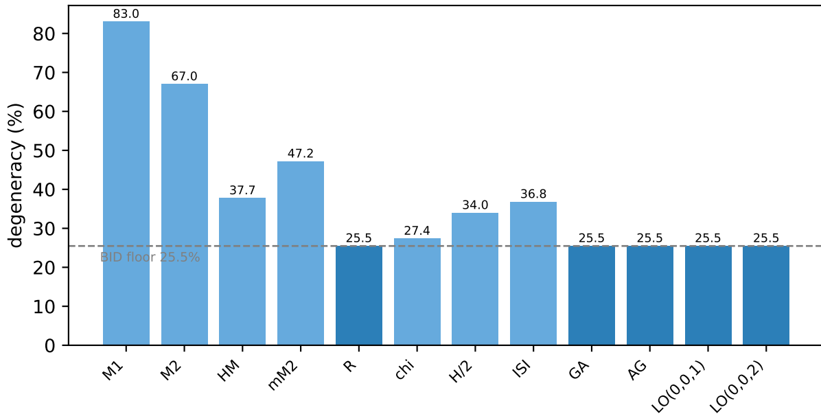
Degeneracy on the 106 trees of order 10
