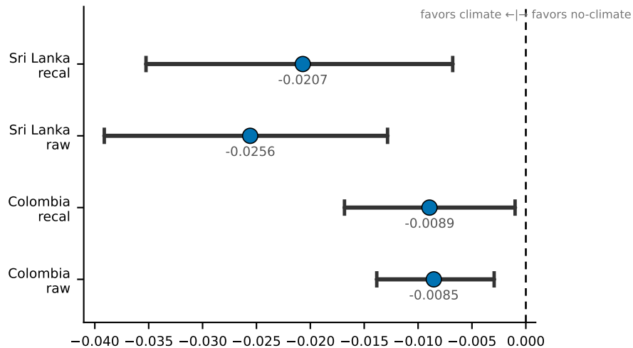
(A1) \Delta\text{NLL} (nats)
