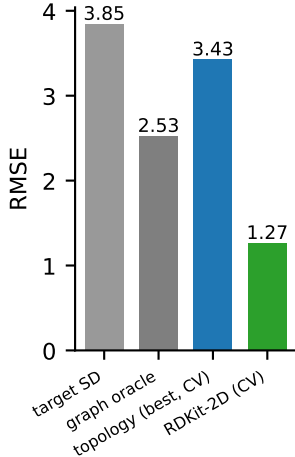
FreeSolv
