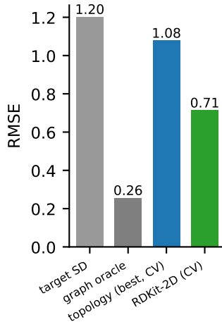
Lipophilicity
