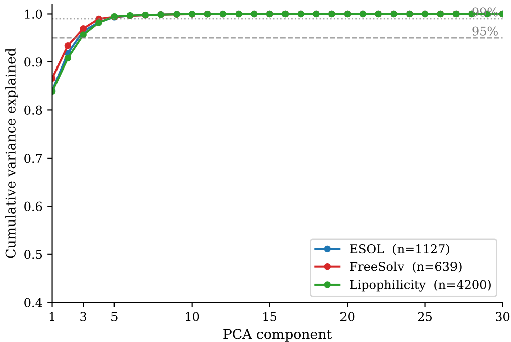
Effective rank of the 30-index baseline (3 components capture 95% of variance on all three datasets)
