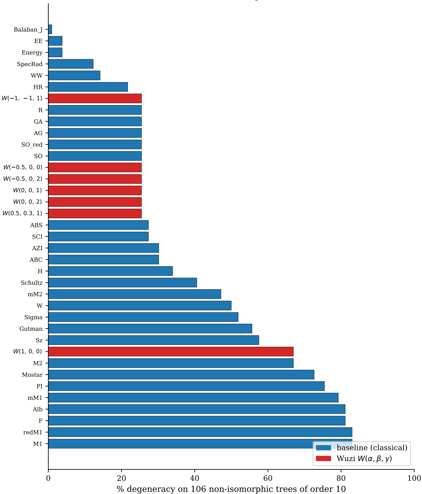
Index degeneracy on trees of order 10 (lower = better discrimination among 106 distinct structures)
