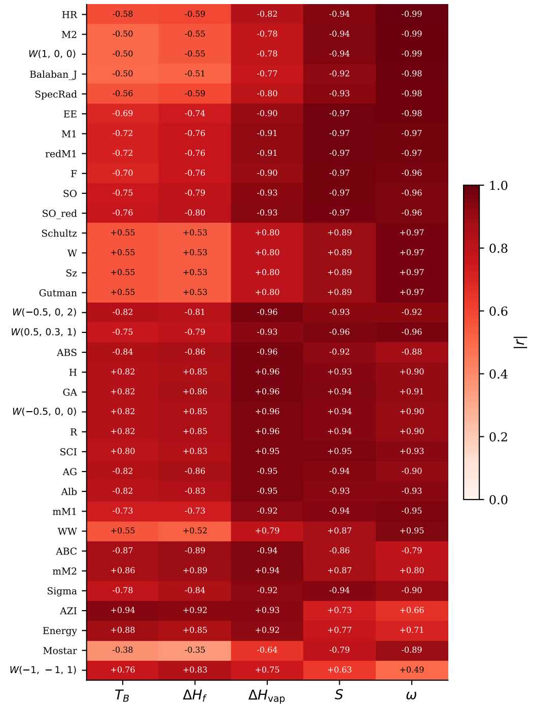
Octane property-correlation benchmark: signed Pearson r (color encodes |r| ) — n = 18 Degenerate (constant on the 18 octanes, |r| undefined): PI.
