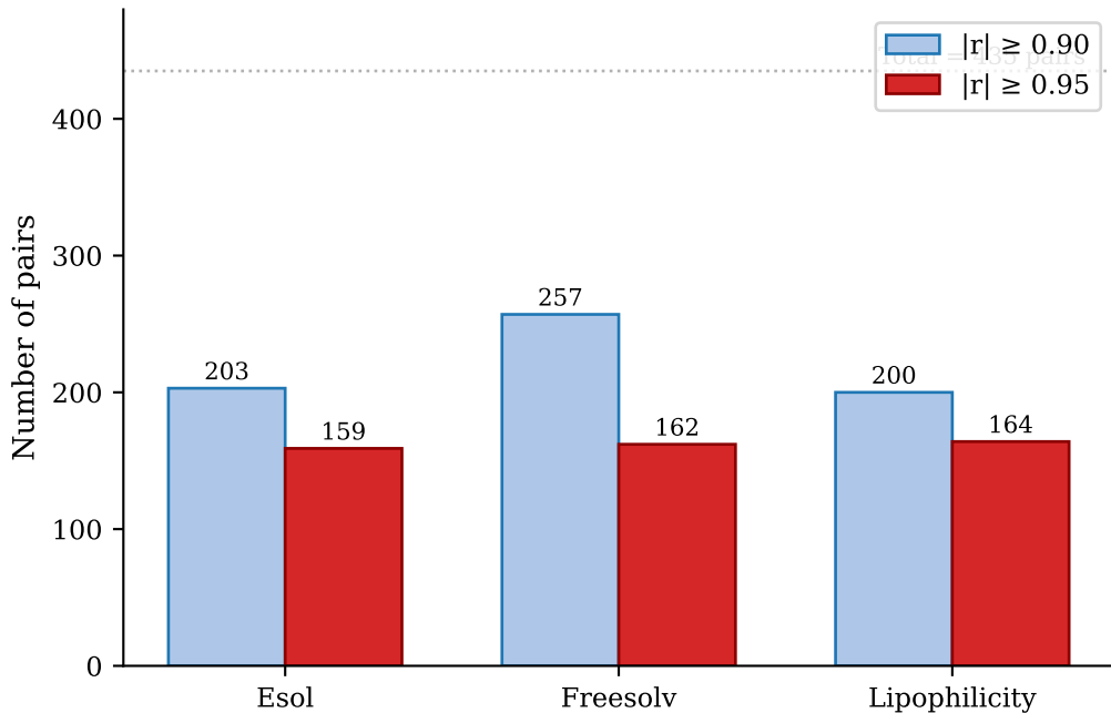
Redundant pairs out of C(30, 2) = 435 baseline index pairs
