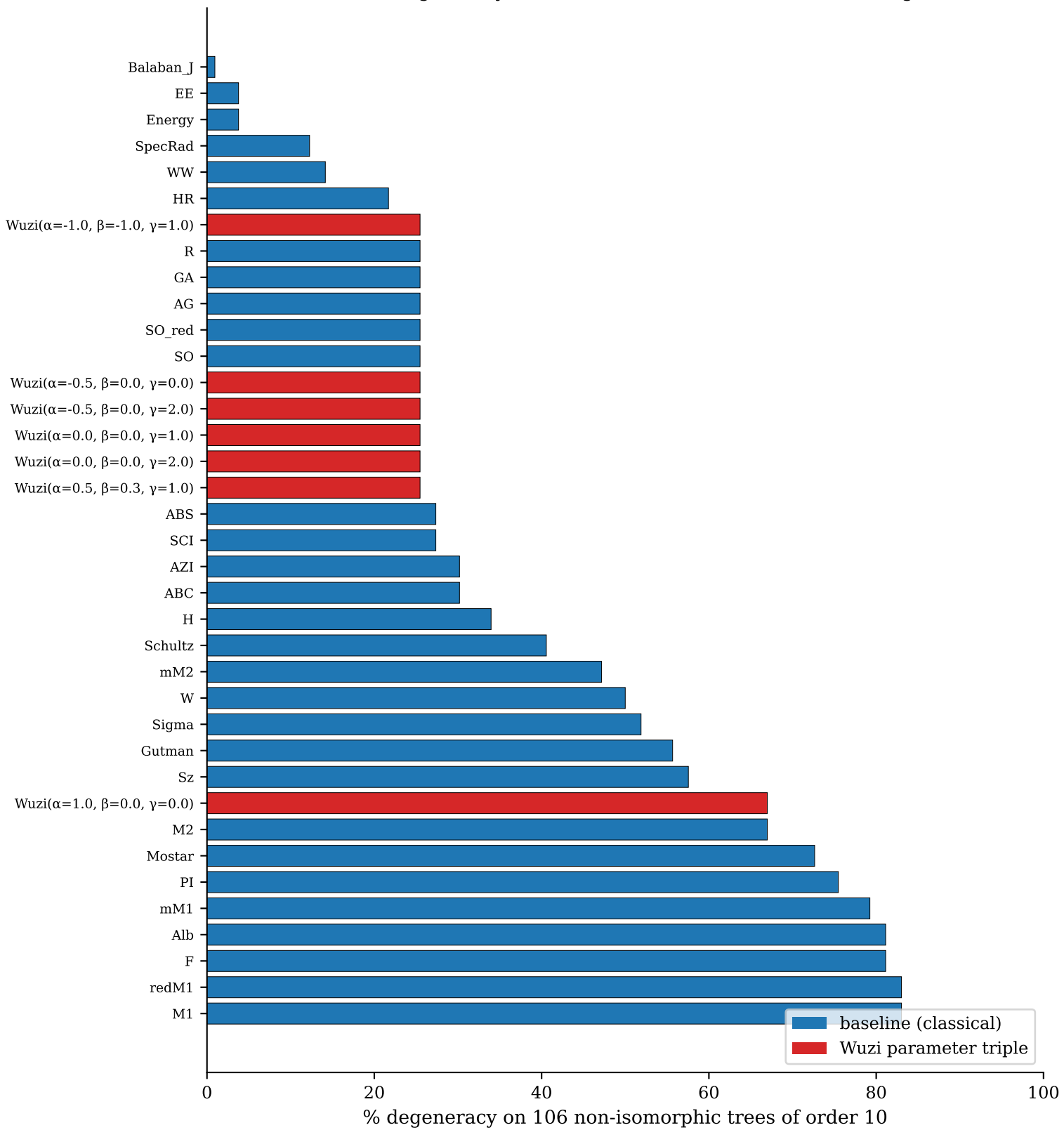
Index degeneracy on trees(10): lower is more discriminating
