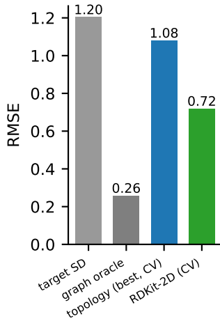
Lipophilicity
