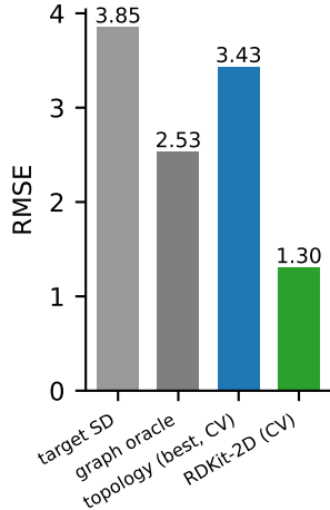
FreeSolv
