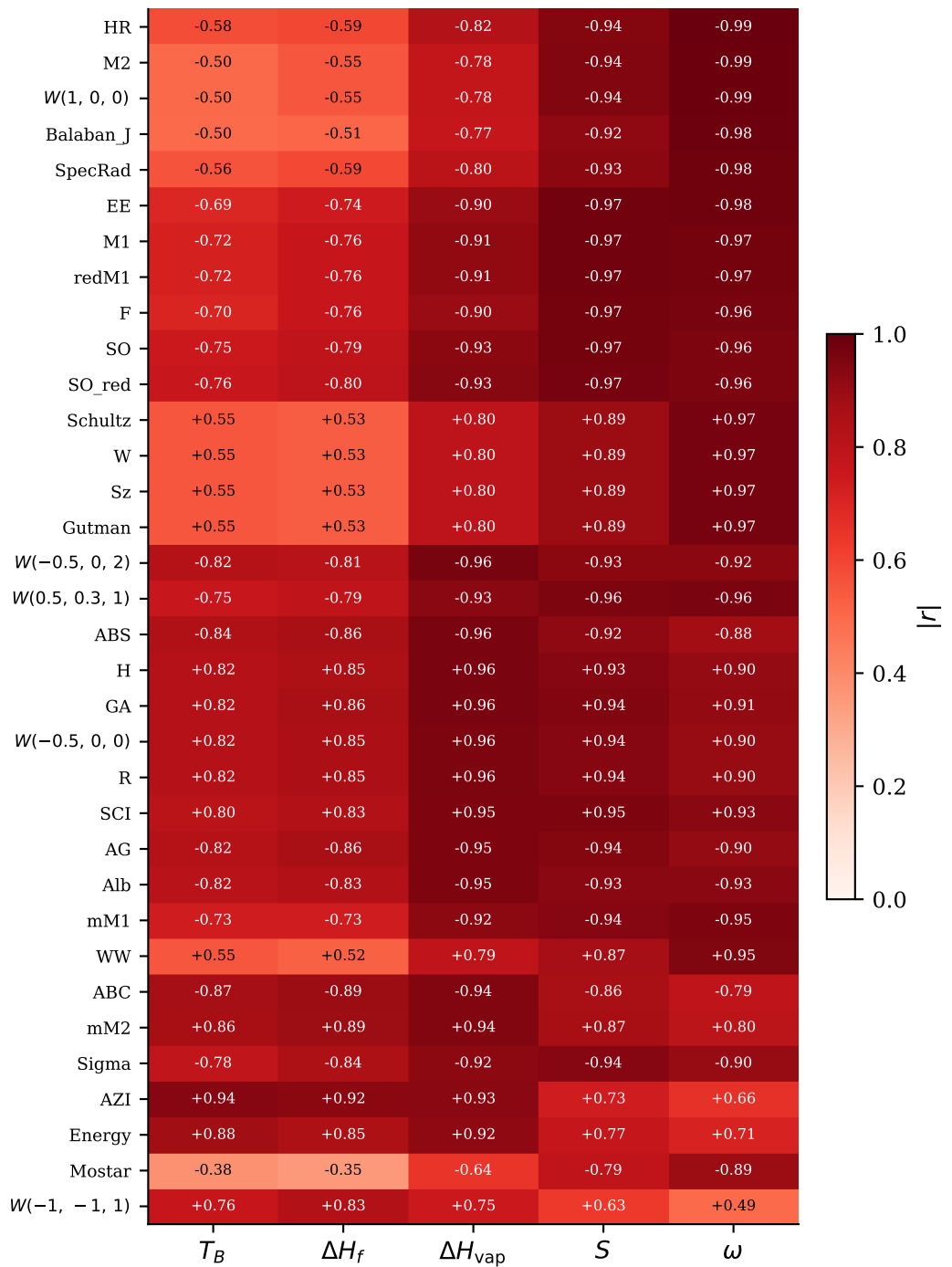
Octane prediction: signed Pearson r (color encodes |r| ) — n = 18 Degenerate (constant on the 18 octanes, |r| undefined): PI.
