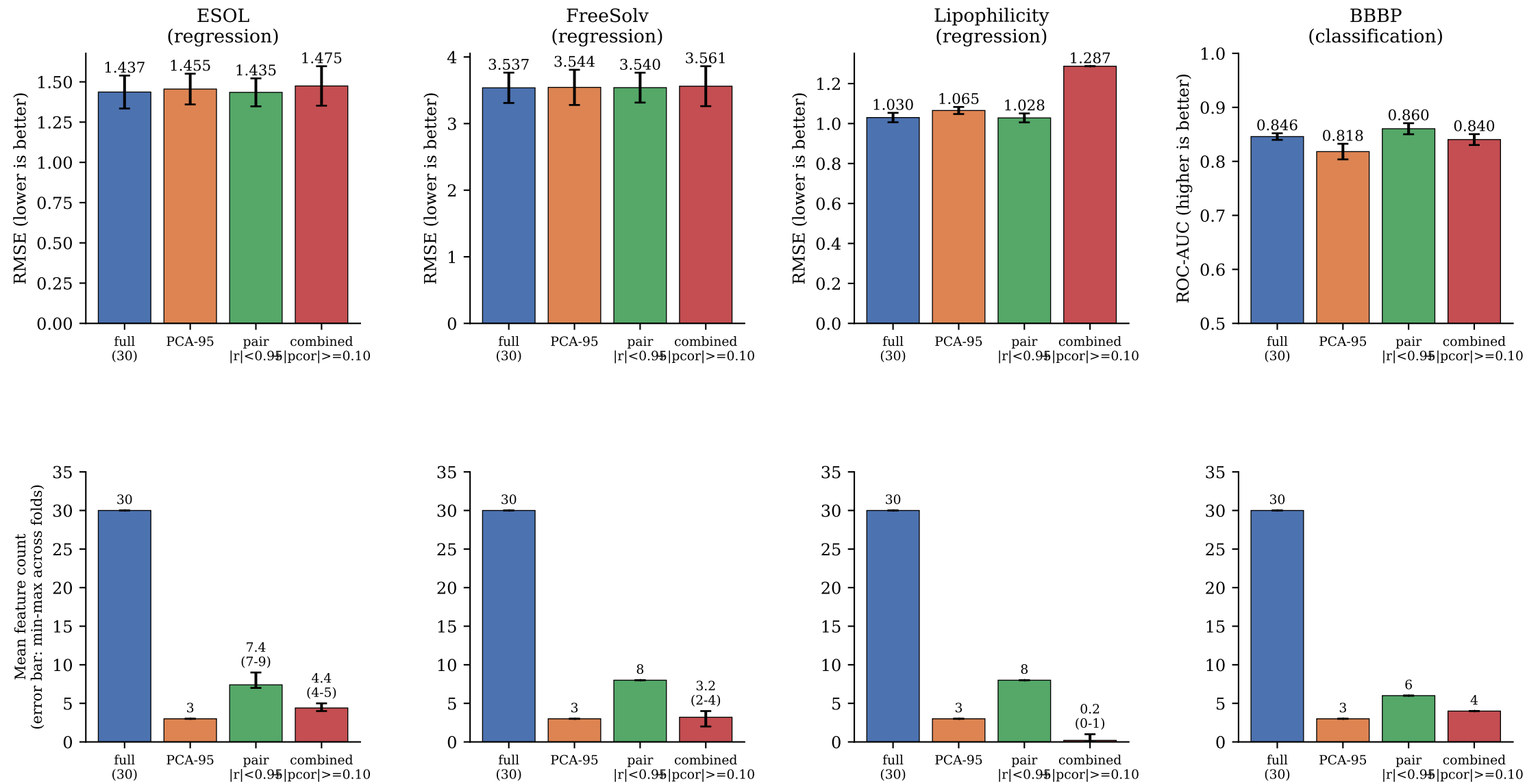
ML benchmark across 5-fold cross-validation: redundancy screening preserves RandomForest performance while reducing input dimension Top: primary metric mean \pm std across folds. Bottom: mean feature count, error bar = min-max range across folds.
