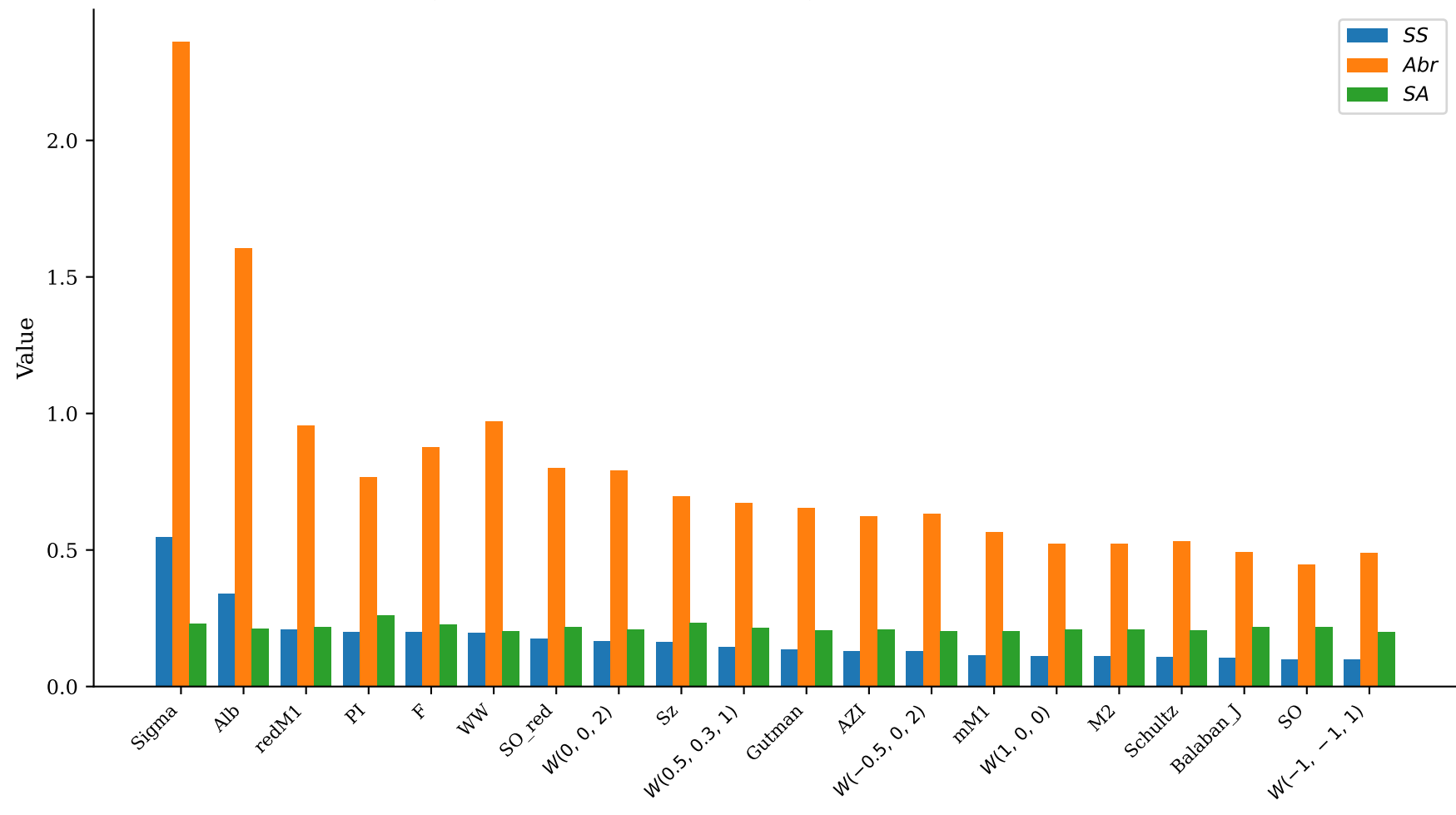
Structure sensitivity on 75 decane isomers — top 20 by SS ( SS = \sigma/\mu , Abr = (\max - \min)/\mu , SA = SS/Abr )
