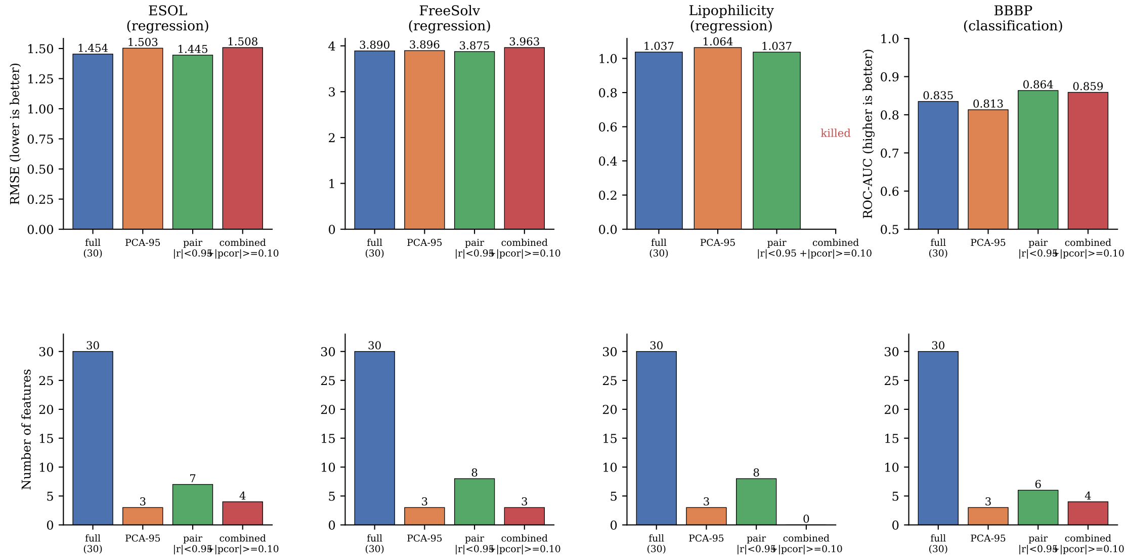
ML benchmark: redundancy screening preserves RandomForest performance while reducing input dimension Top: primary metric (RMSE for regression, ROC-AUC for classification). Bottom: feature count per configuration.
