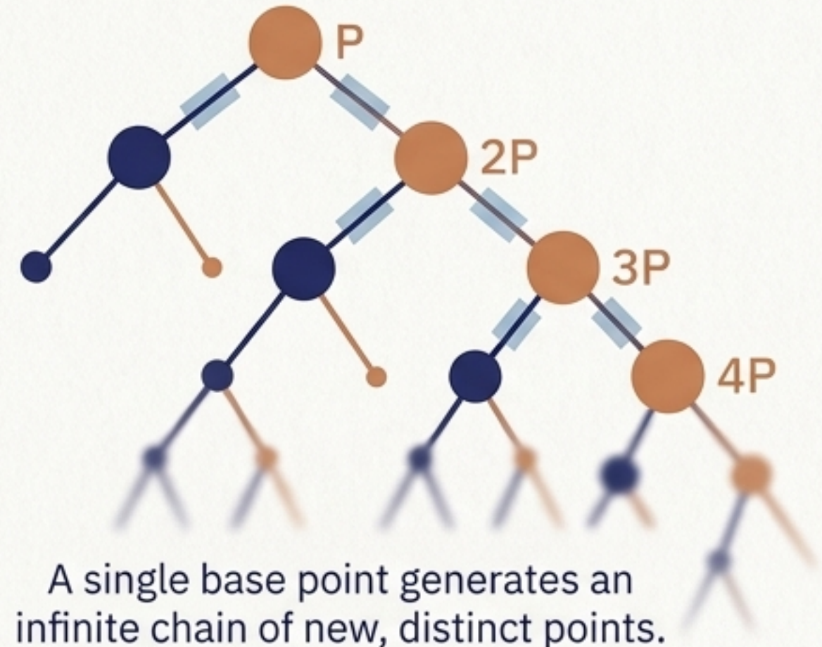
Rank > 0
