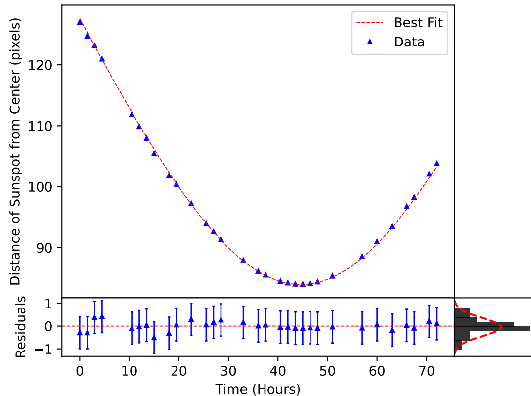
\delta_m(\omega, t) Plotted over the Motion of Sunspot 3556
