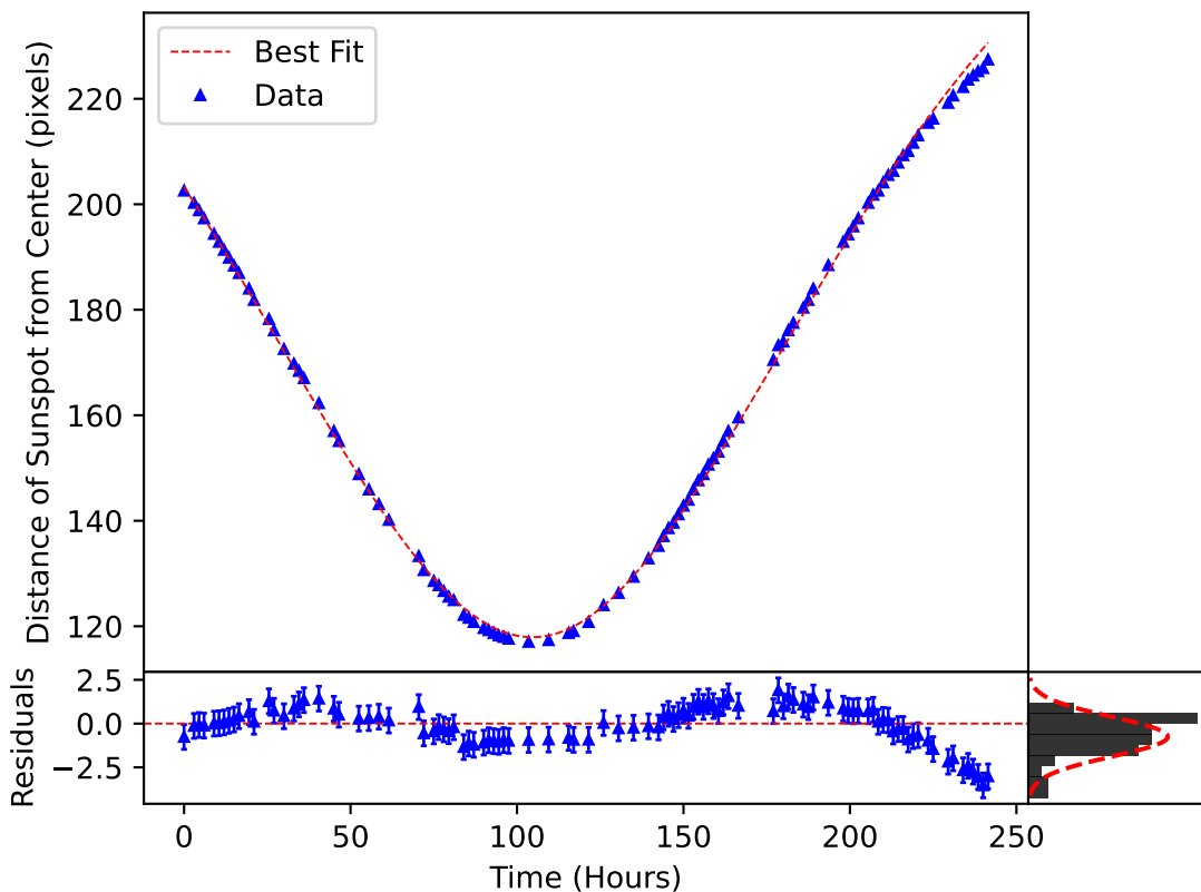
\delta_m(\omega, t) Plotted over the Motion of Sunspot 3591
