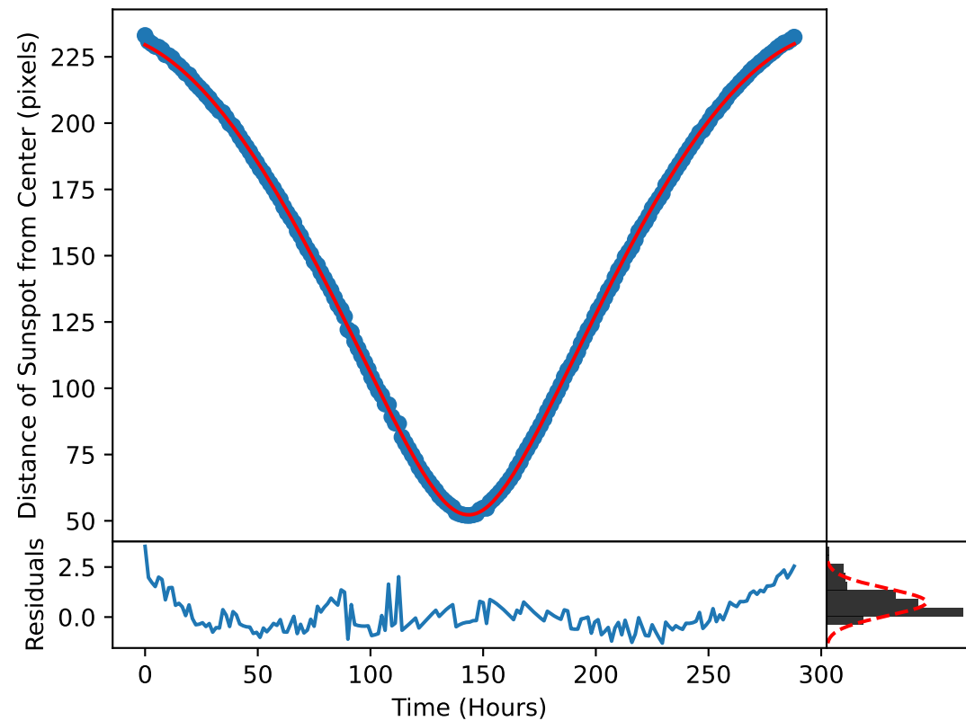
\delta_m(\omega, t) Plotted over the Motion of Sunspot 4018
