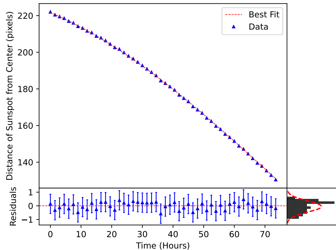
\delta_m(\omega, t) Plotted over the Motion of Sunspot 3670
