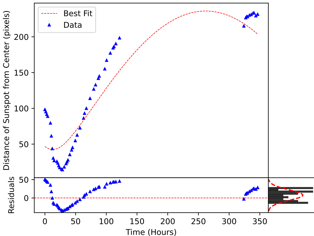
\delta_m(\omega, t) Plotted over the Motion of Sunspot 3638.5
