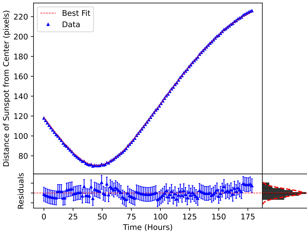
\delta_m(\omega, t) Plotted over the Motion of Sunspot 3724
