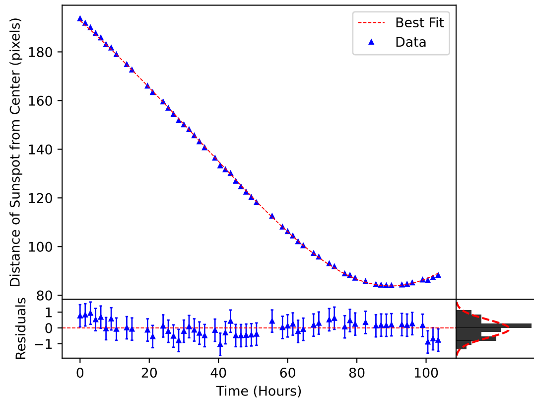
\delta_m(\omega, t) Plotted over the Motion of Sunspot 3603
