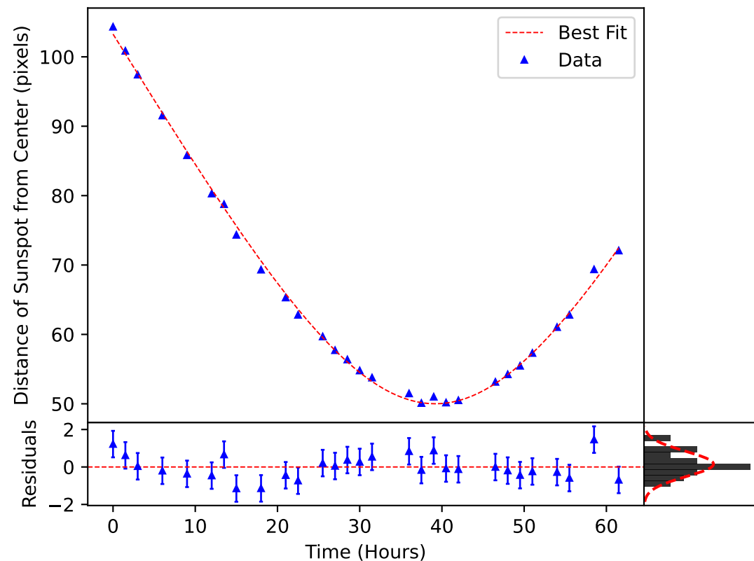
\delta_m(\omega, t) Plotted over the Motion of Sunspot 3638
