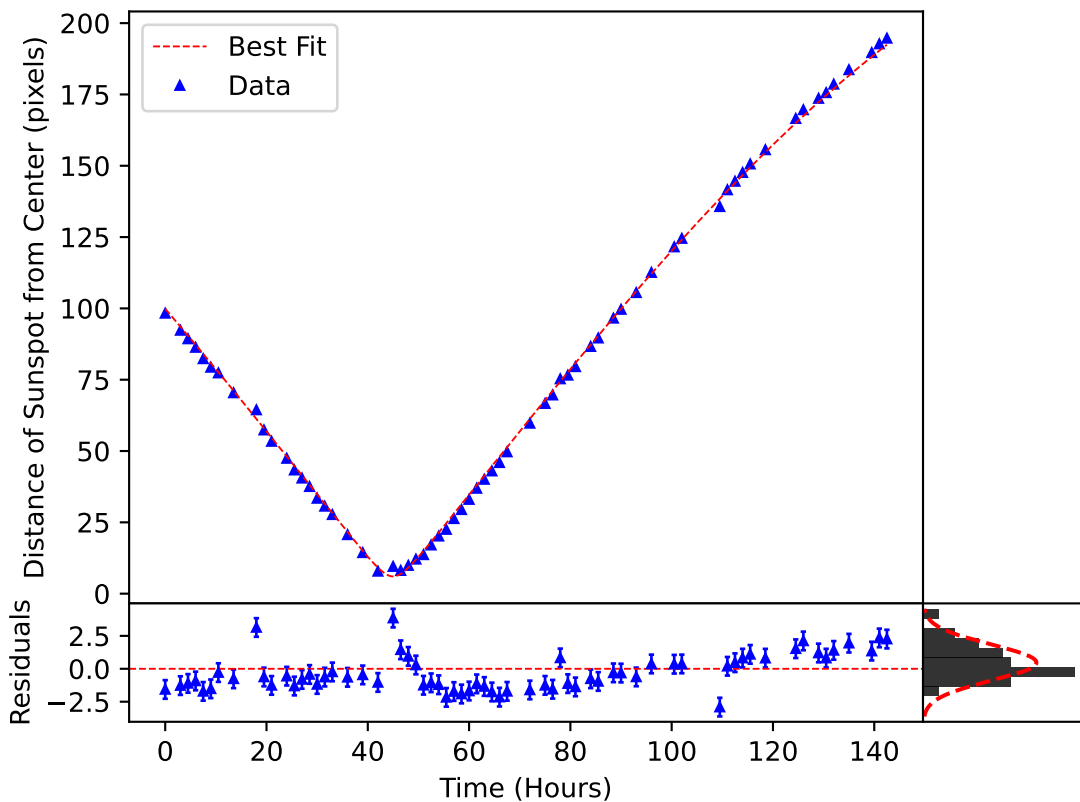
\delta_m(\omega, t) Plotted over the Motion of Sunspot 3545
