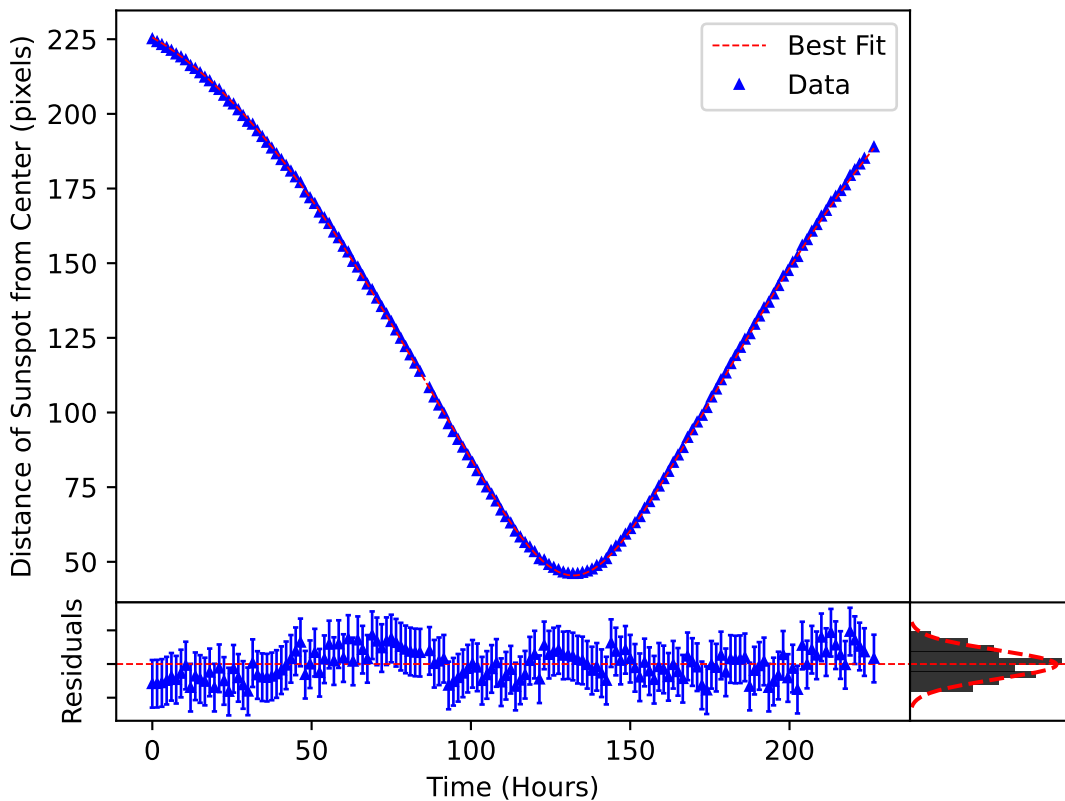
\delta_m(\omega, t) Plotted over the Motion of Sunspot 3674
