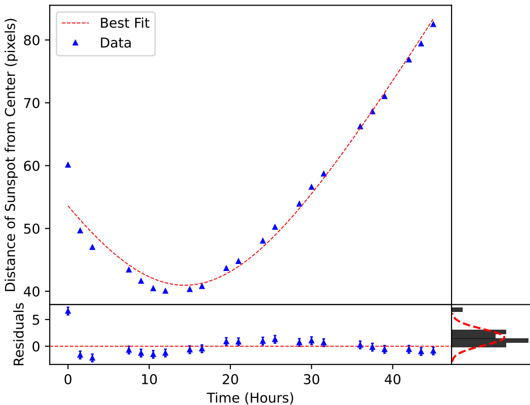
\delta_m(\omega, t) Plotted over the Motion of Sunspot 3545
