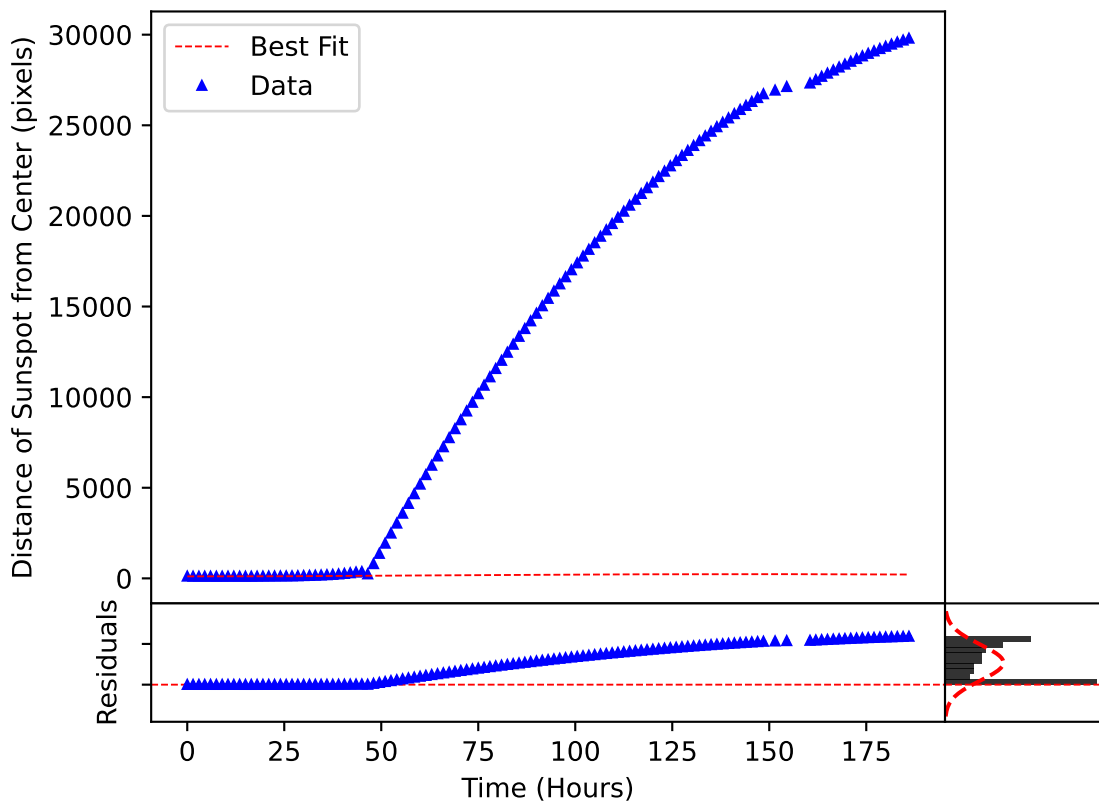
\delta_m(\omega, t) Plotted over the Motion of Sunspot 3712.1
