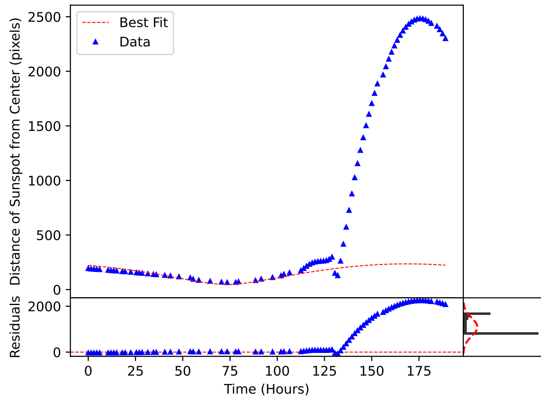
\delta_m(\omega, t) Plotted over the Motion of Sunspot 3644
