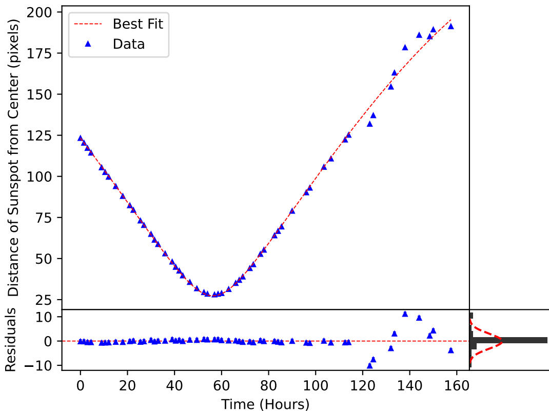
\delta_m(\omega, t) Plotted over the Motion of Sunspot 3617
