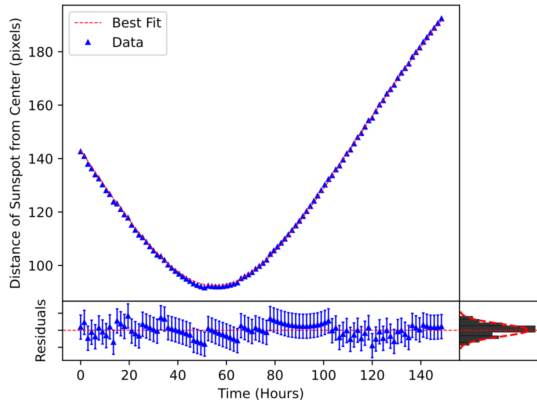
\delta_m(\omega, t) Plotted over the Motion of Sunspot 3736
