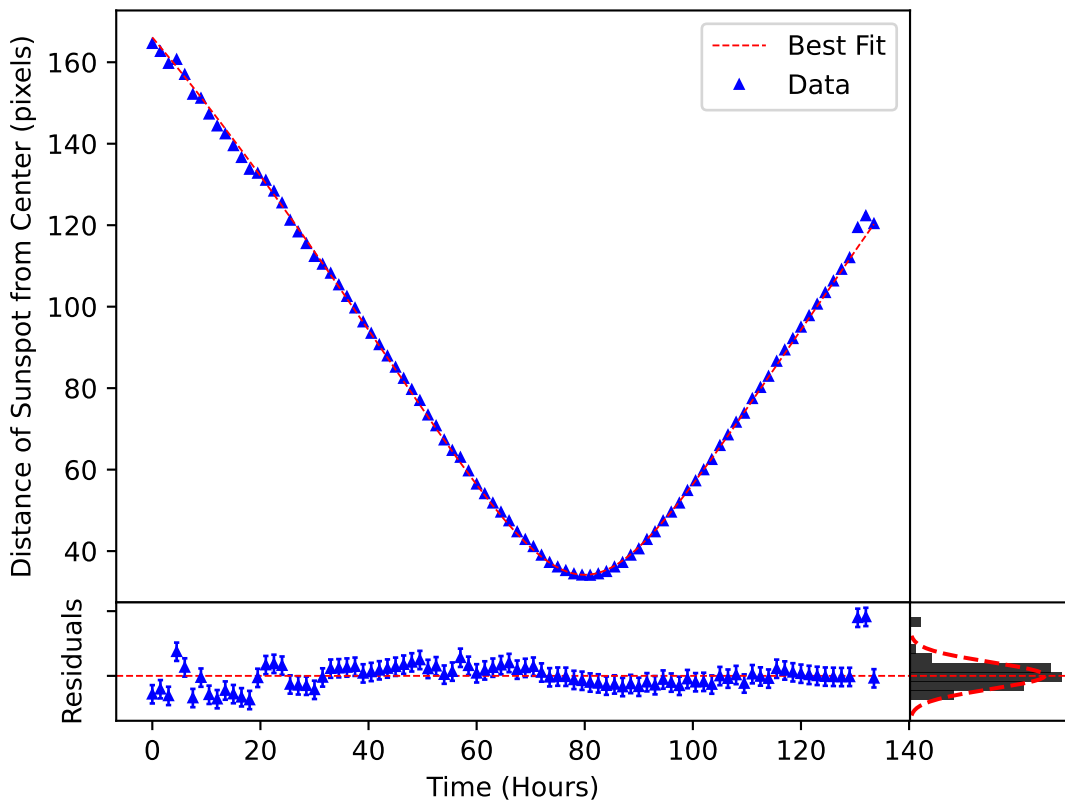
\delta_m(\omega, t) Plotted over the Motion of Sunspot 3720
