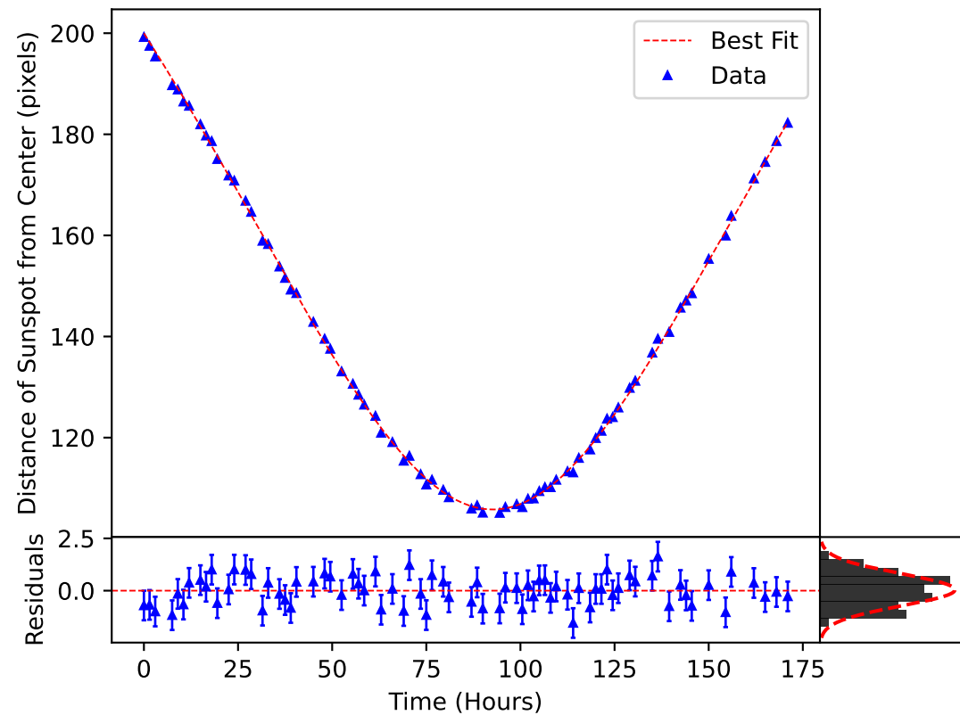
\delta_m(\omega, t) Plotted over the Motion of Sunspot 3590
