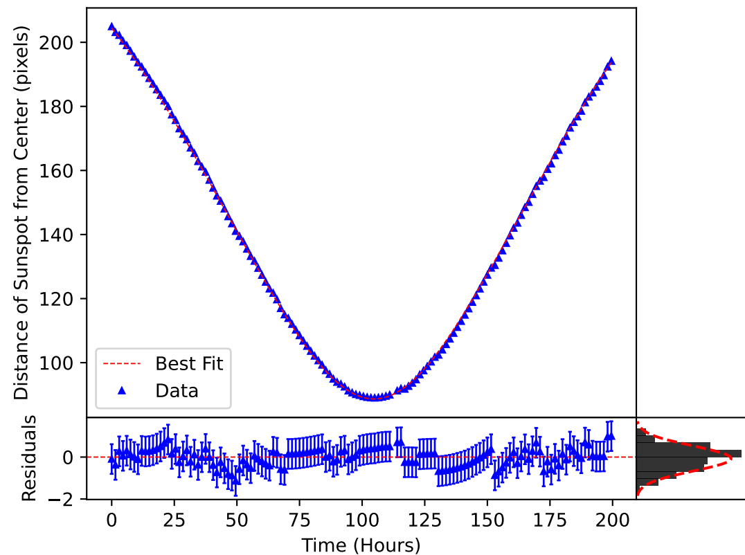
\delta_m(\omega, t) Plotted over the Motion of Sunspot 3672
