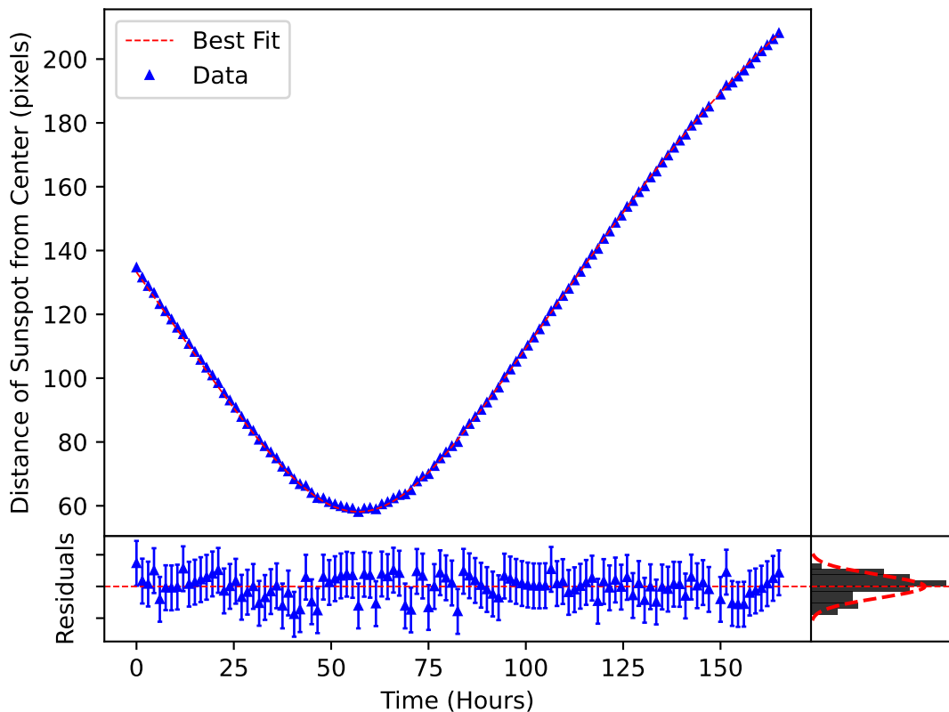
\delta_m(\omega, t) Plotted over the Motion of Sunspot 2794?
