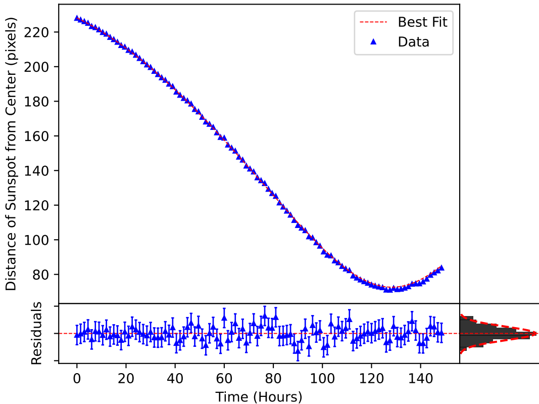
\delta_m(\omega, t) Plotted over the Motion of Sunspot 2785?
