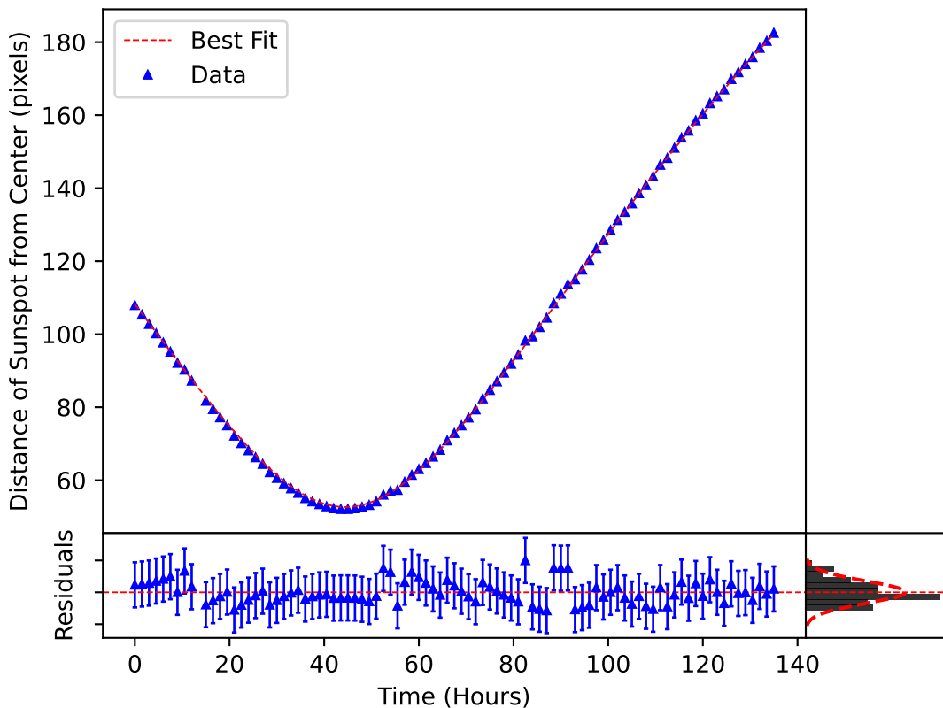
\delta_m(\omega, t) Plotted over the Motion of Sunspot 3685.3
