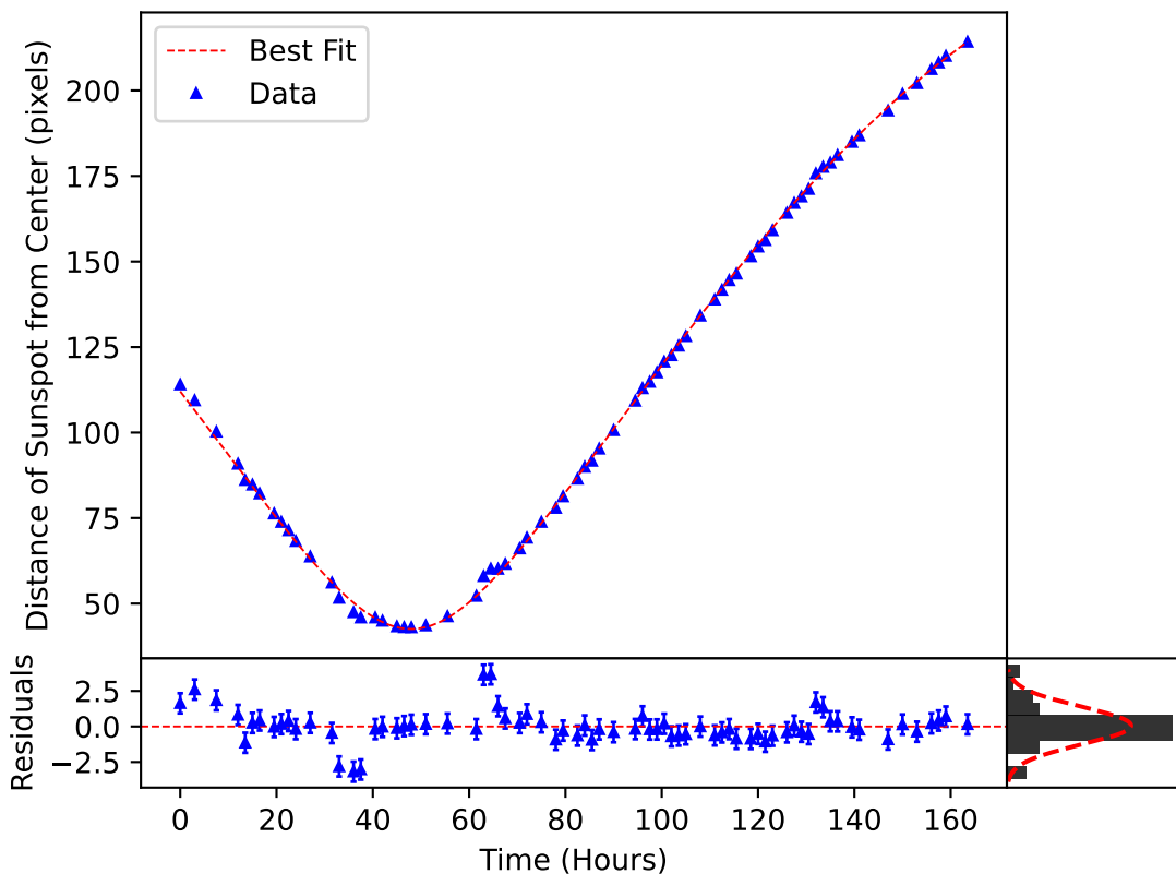
\delta_m(\omega, t) Plotted over the Motion of Sunspot 3576
