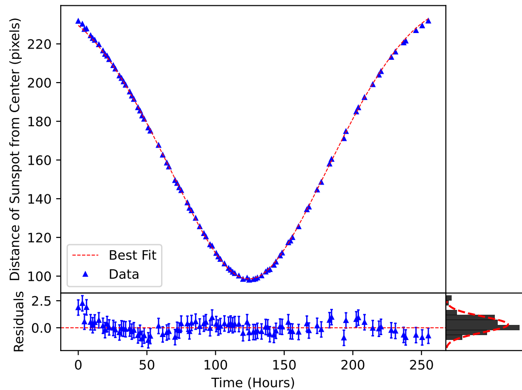
\delta_m(\omega, t) Plotted over the Motion of Sunspot 3614
