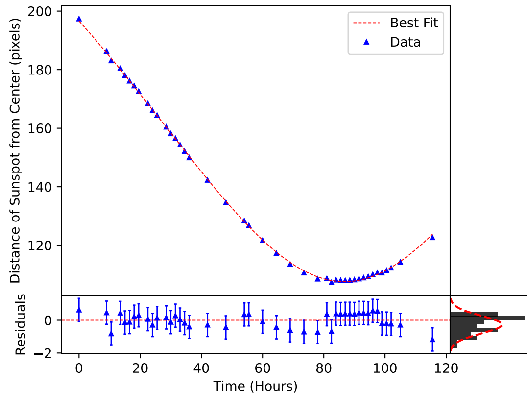
\delta_m(\omega, t) Plotted over the Motion of Sunspot 3596
