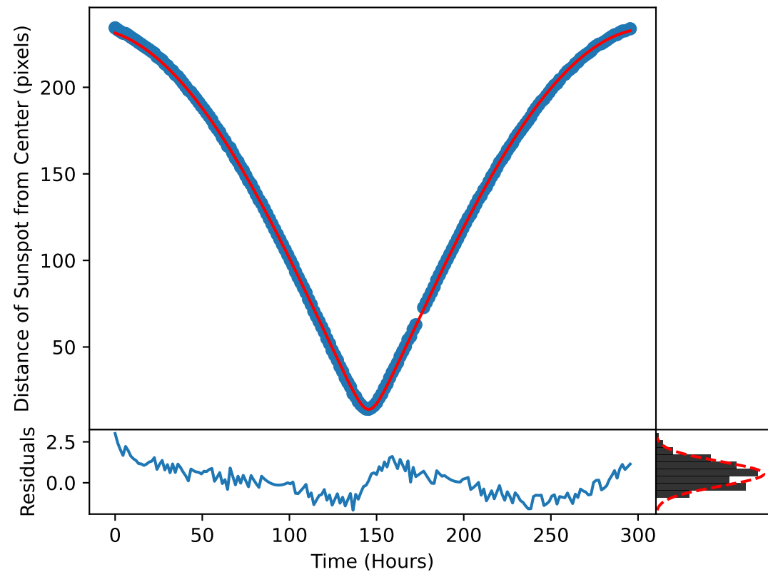
\delta_m(\omega, t) Plotted over the Motion of Sunspot 4216
