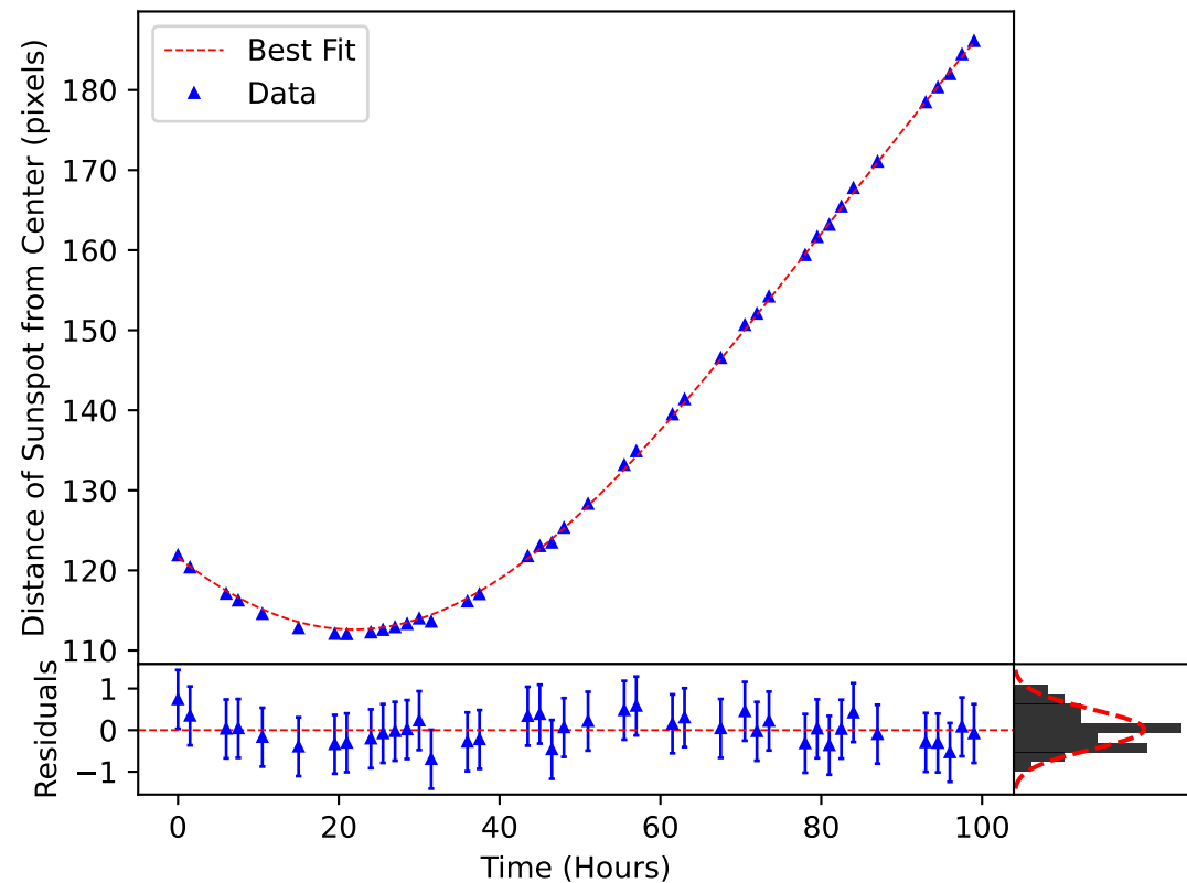
\delta_m(\omega, t) Plotted over the Motion of Sunspot 3573
