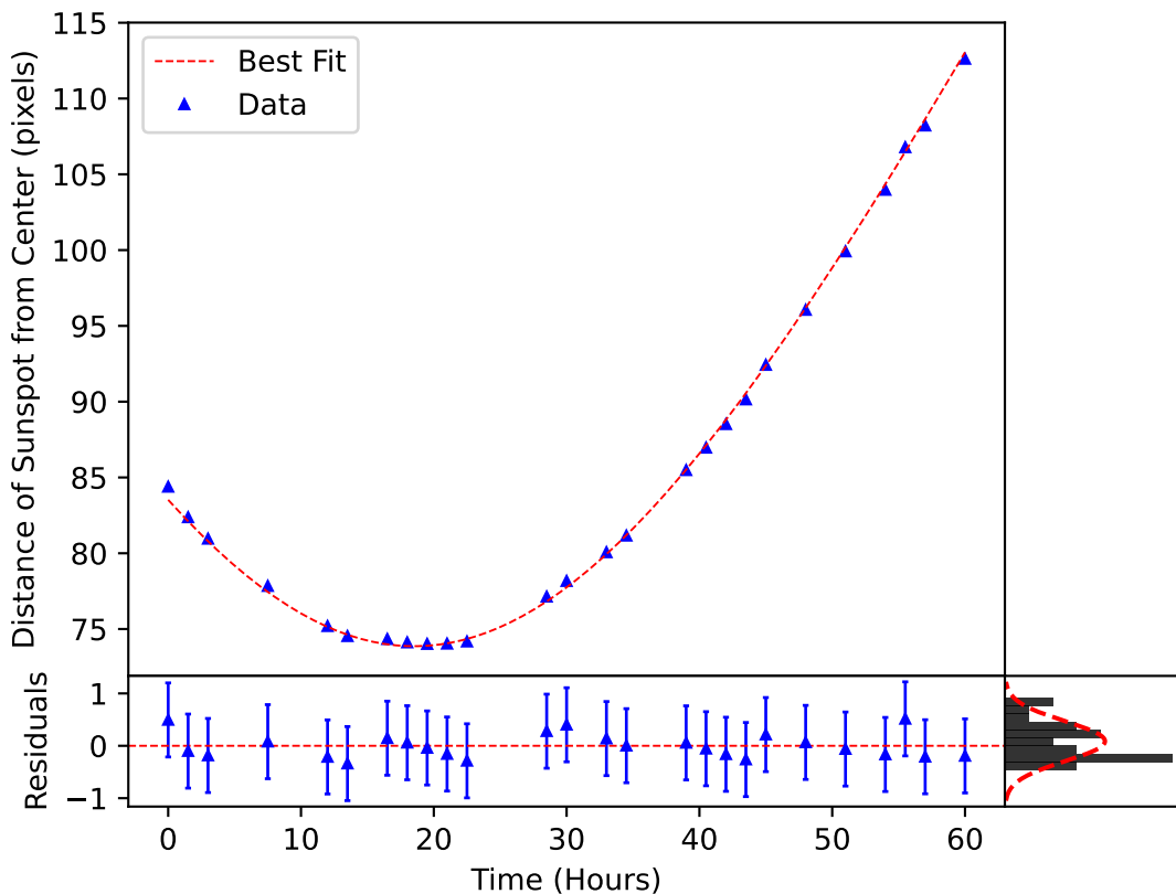
\delta_m(\omega, t) Plotted over the Motion of Sunspot 3641.5
