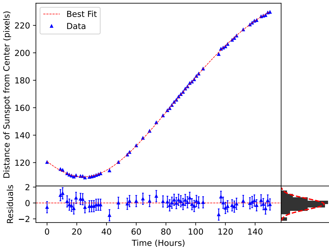
\delta_m(\omega, t) Plotted over the Motion of Sunspot 3595
