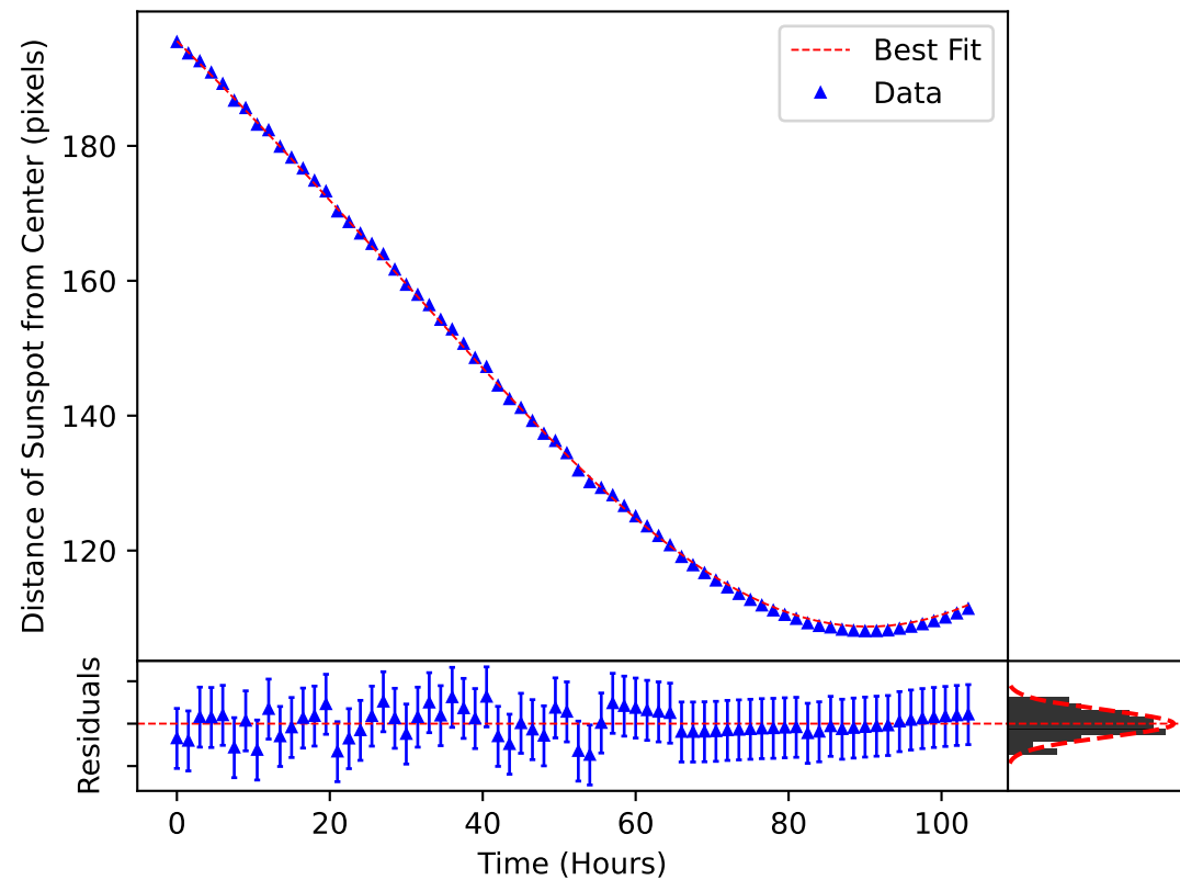
\delta_m(\omega, t) Plotted over the Motion of Sunspot 2781
