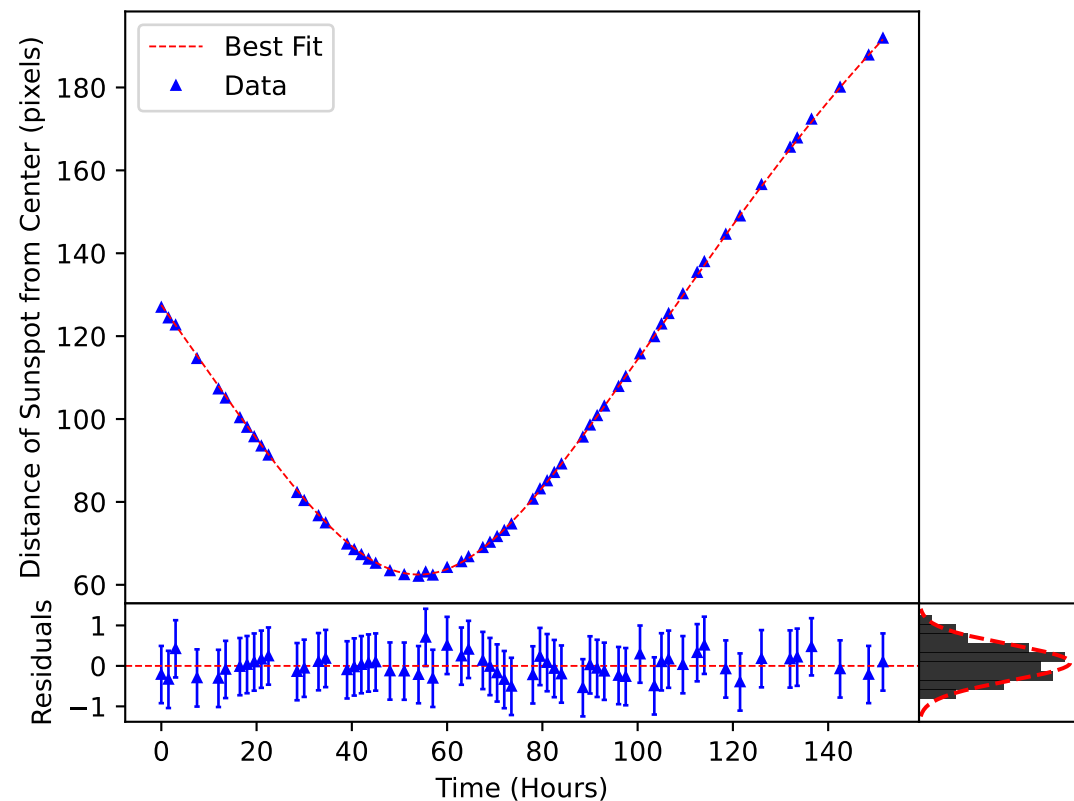
\delta_m(\omega, t) Plotted over the Motion of Sunspot 3636
