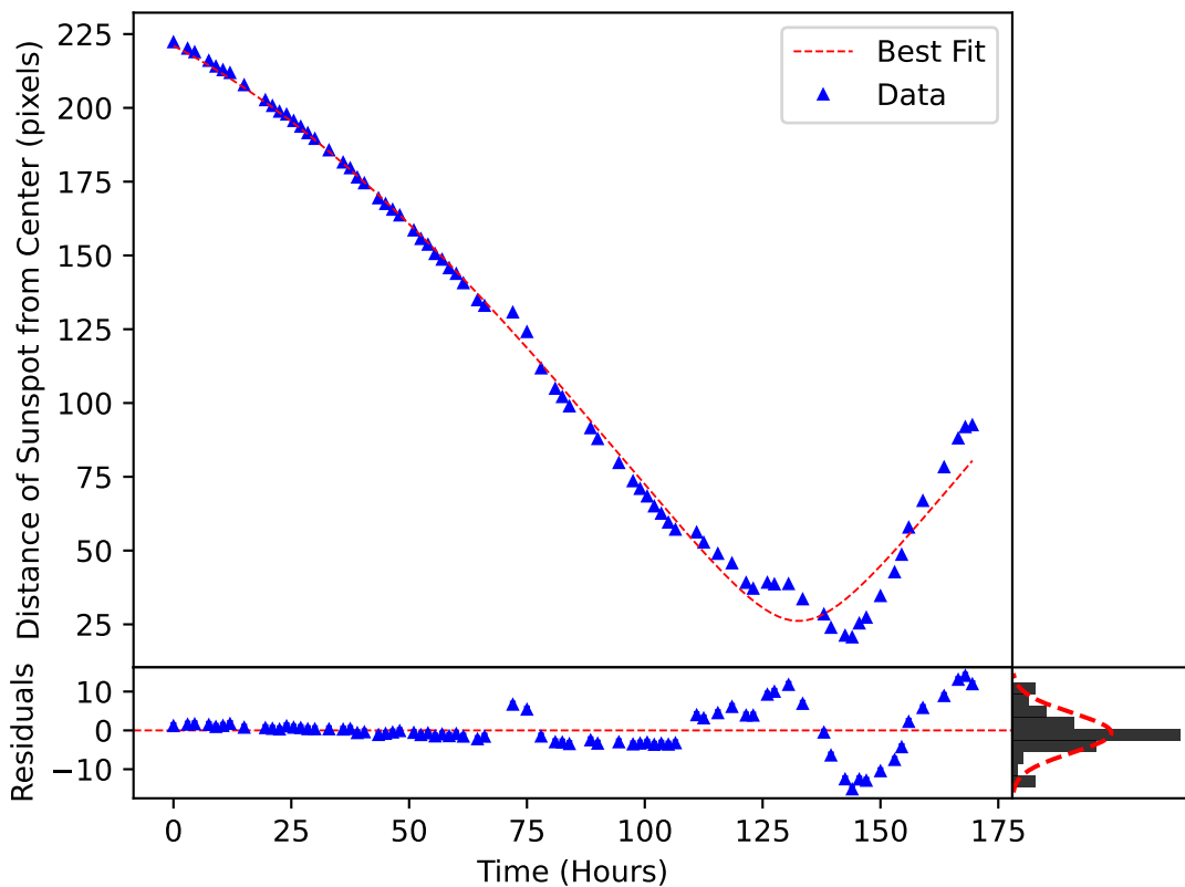
\delta_m(\omega, t) Plotted over the Motion of Sunspot 3584
