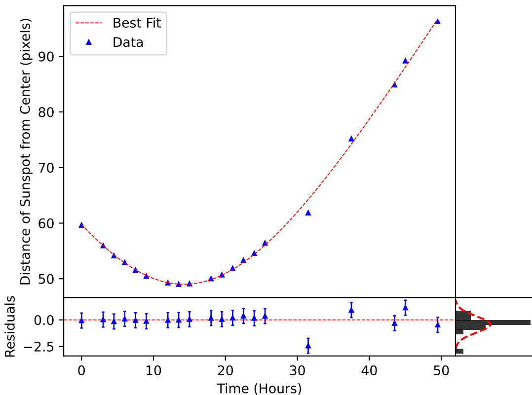
\delta_m(\omega, t) Plotted over the Motion of Sunspot 3594
