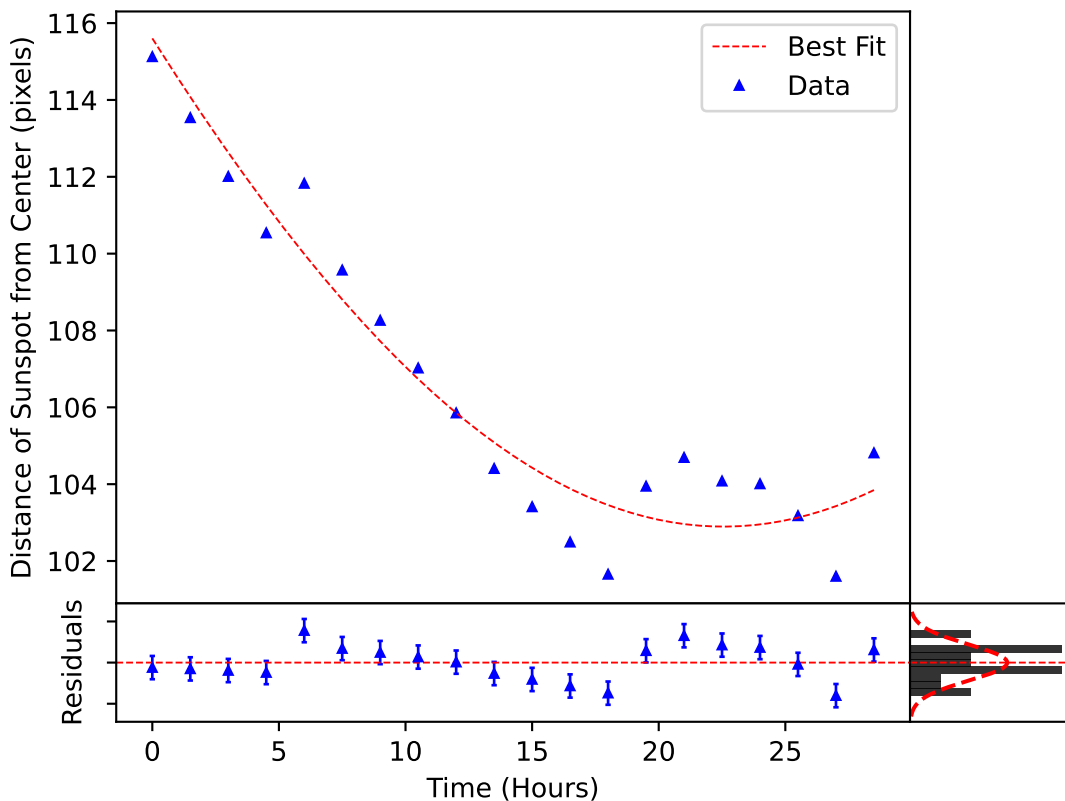
\delta_m(\omega, t) Plotted over the Motion of Sunspot 10232020
