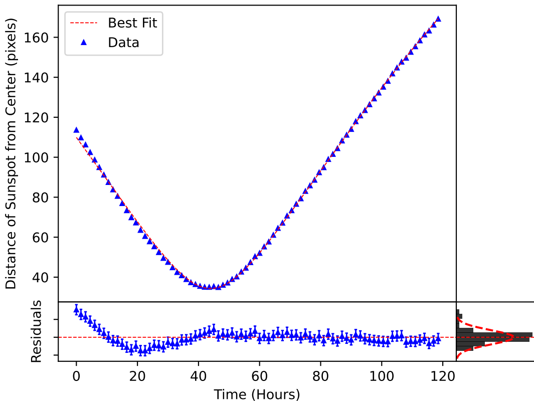
\delta_m(\omega, t) Plotted over the Motion of Sunspot 2757
