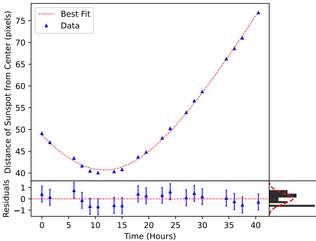
\delta_m(\omega, t) Plotted over the Motion of Sunspot 3607
