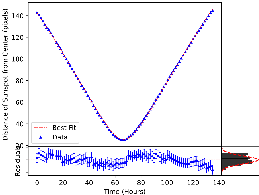
\delta_m(\omega, t) Plotted over the Motion of Sunspot 3686
