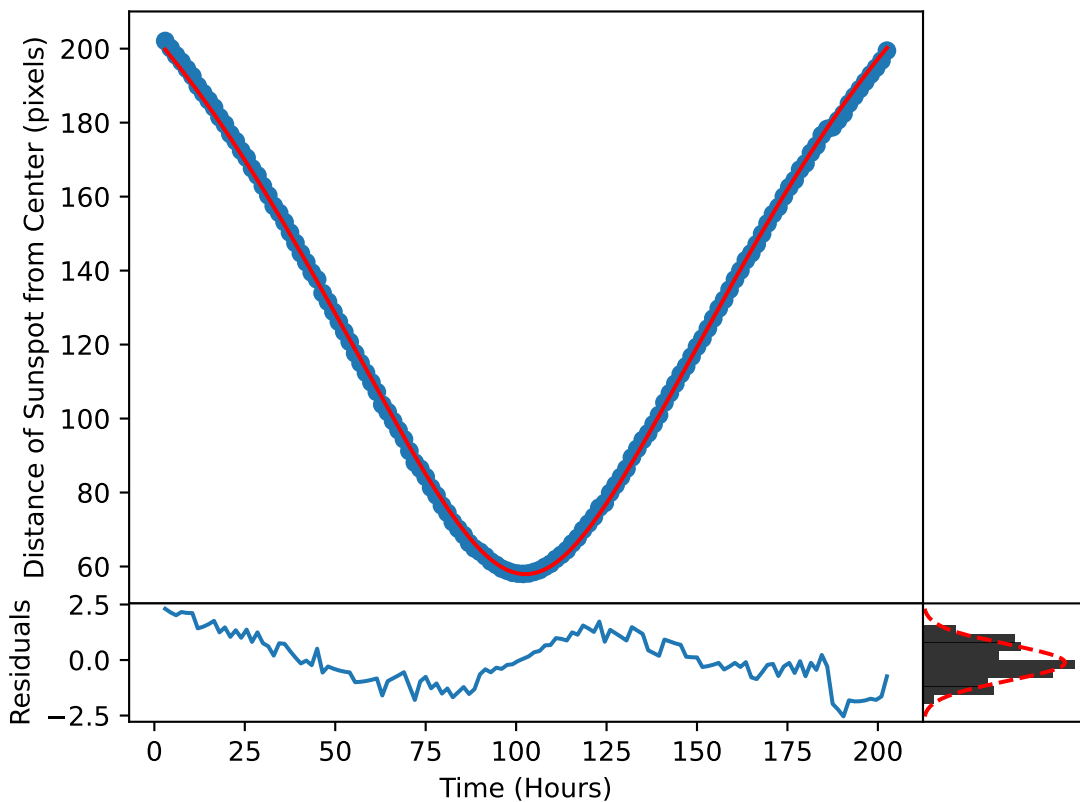
\delta_m(\omega, t) Plotted over the Motion of Sunspot 4019
