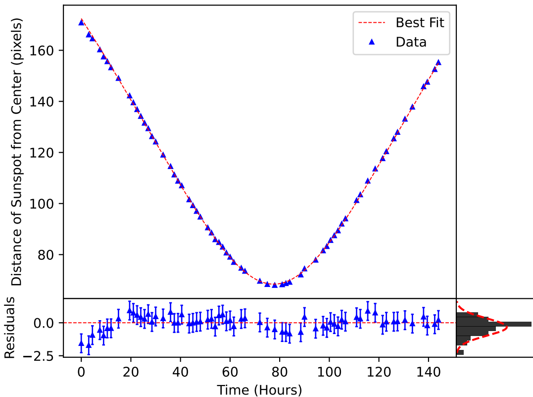
\delta_m(\omega, t) Plotted over the Motion of Sunspot 3583.5
