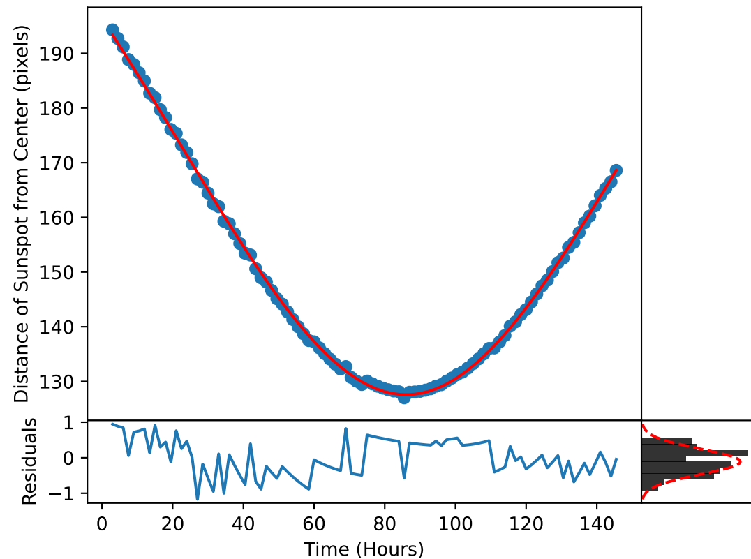
\delta_m(\omega, t) Plotted over the Motion of Sunspot 4023
