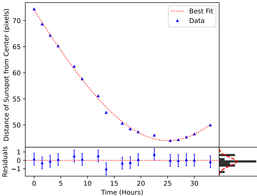
\delta_m(\omega, t) Plotted over the Motion of Sunspot 3600
