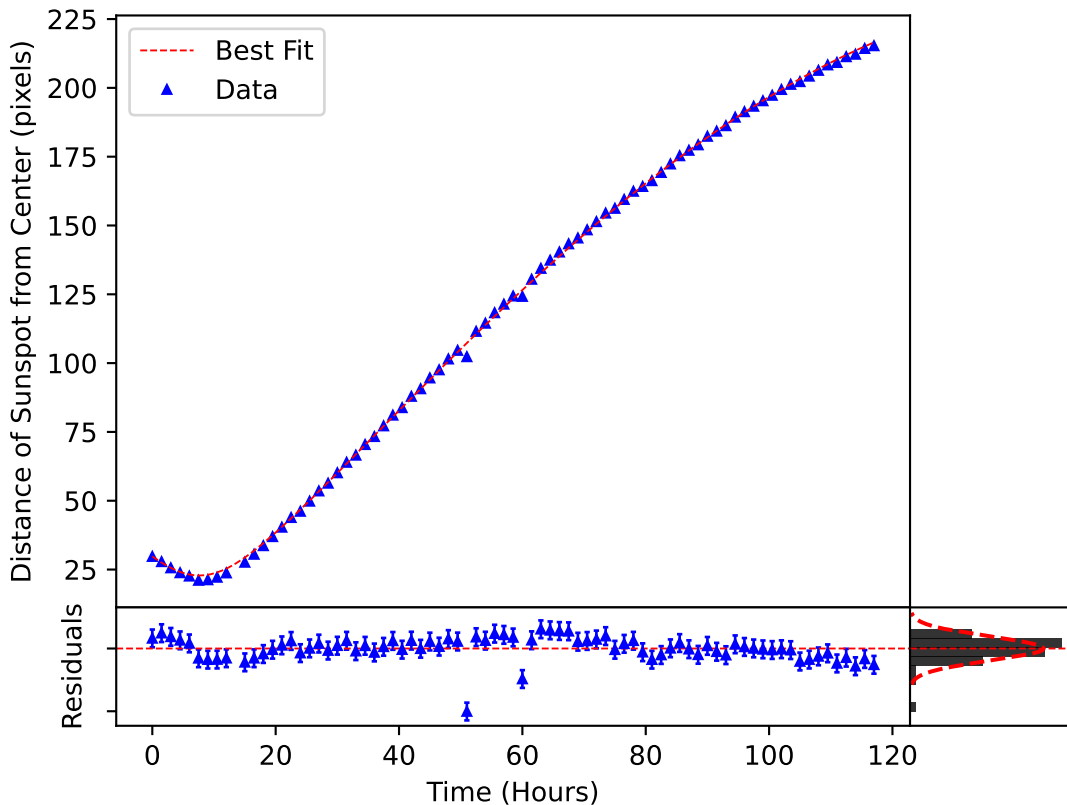
\delta_m(\omega, t) Plotted over the Motion of Sunspot 3684
