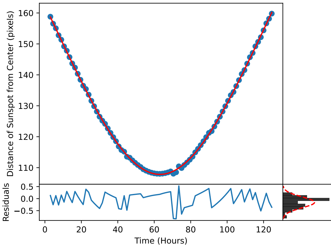
\delta_m(\omega, t) Plotted over the Motion of Sunspot 4020
