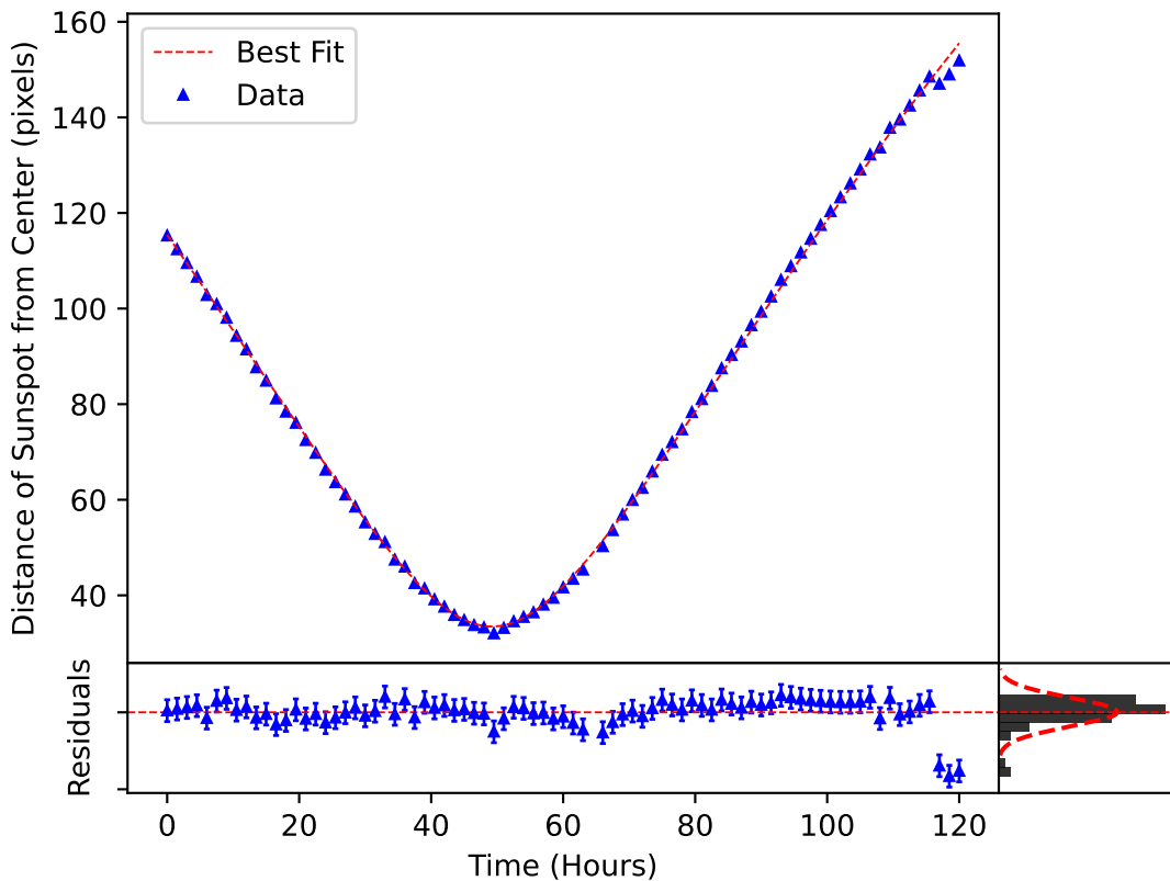
\delta_m(\omega, t) Plotted over the Motion of Sunspot 3703.1
