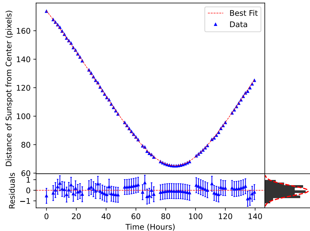
\delta_m(\omega, t) Plotted over the Motion of Sunspot 3769
