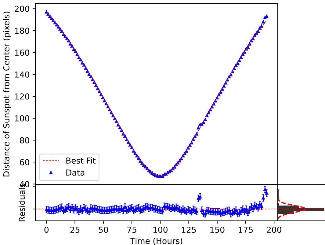
\delta_m(\omega, t) Plotted over the Motion of Sunspot 3711
