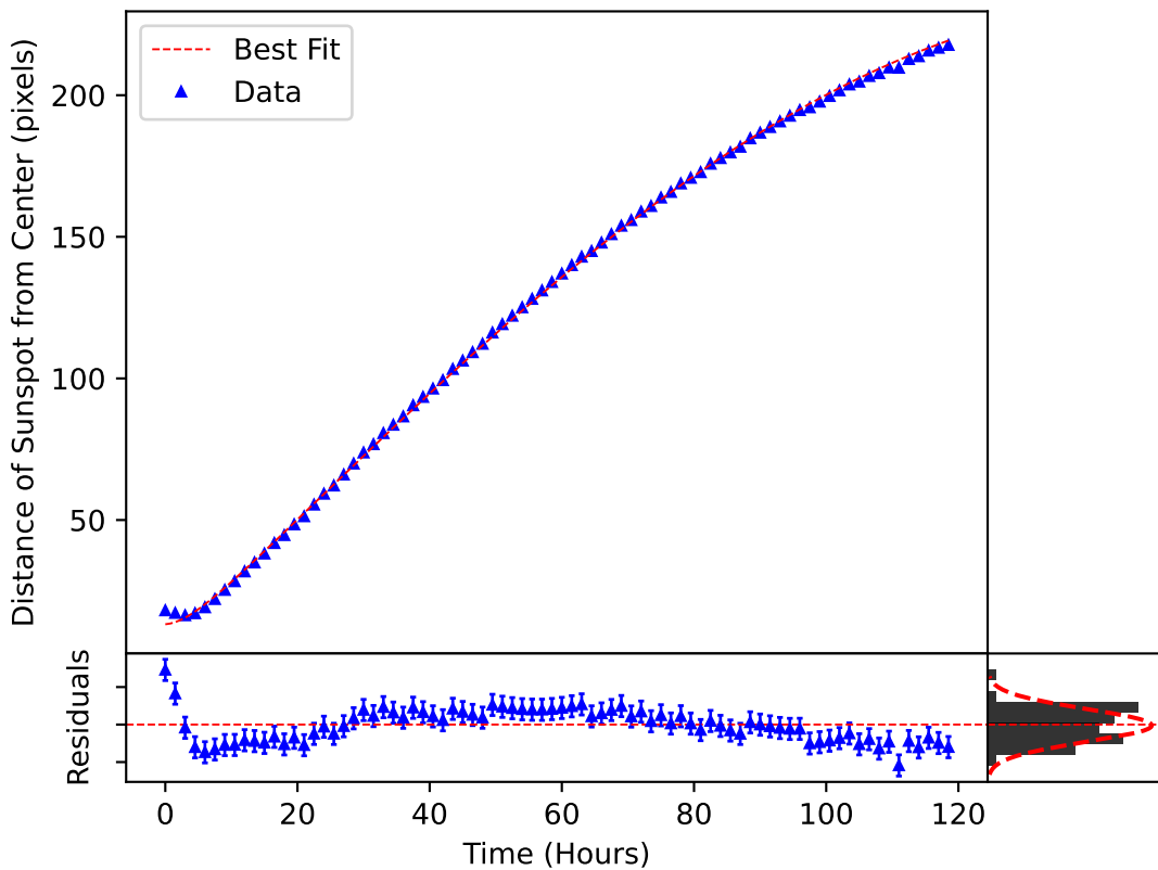
\delta_m(\omega, t) Plotted over the Motion of Sunspot 3699
