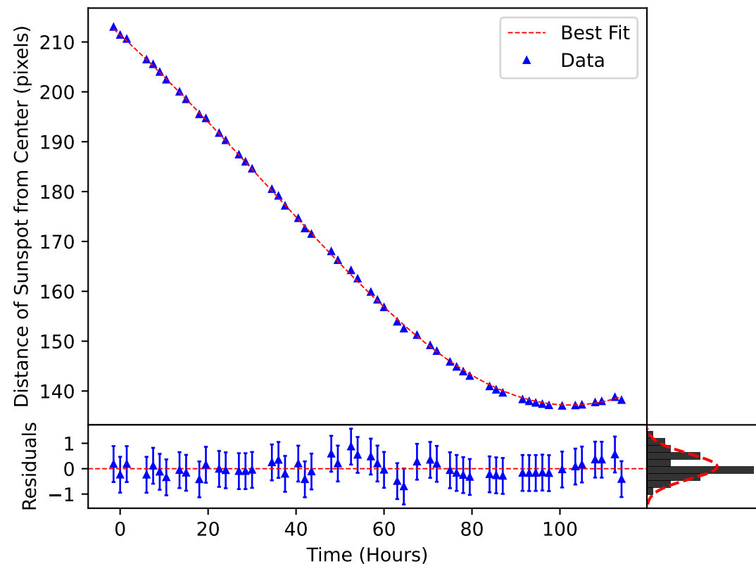
\delta_m(\omega, t) Plotted over the Motion of Sunspot 3611
