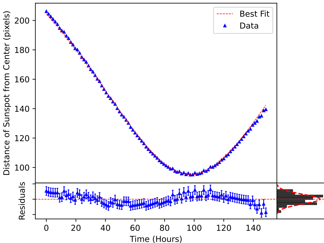
\delta_m(\omega, t) Plotted over the Motion of Sunspot 2784?
