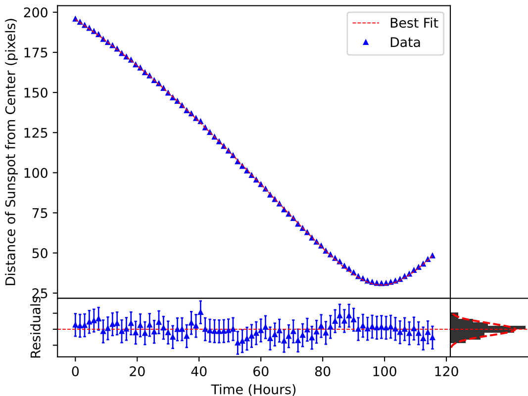
\delta_m(\omega, t) Plotted over the Motion of Sunspot 3689
