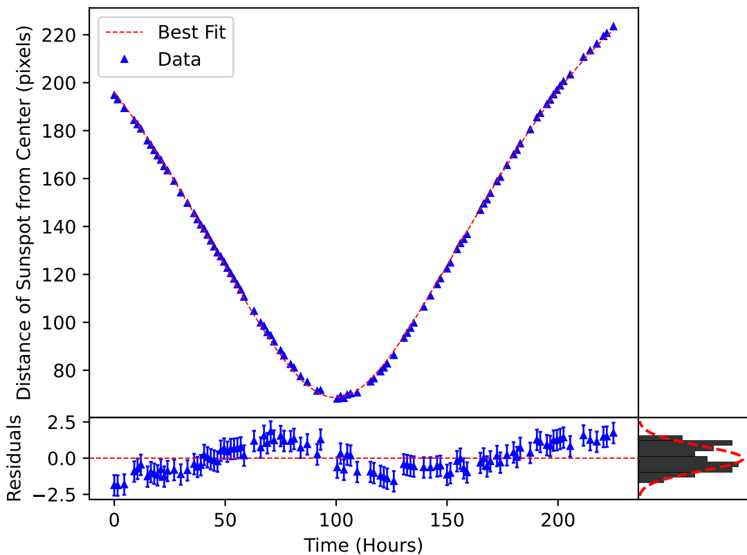
\delta_m(\omega, t) Plotted over the Motion of Sunspot 3549
