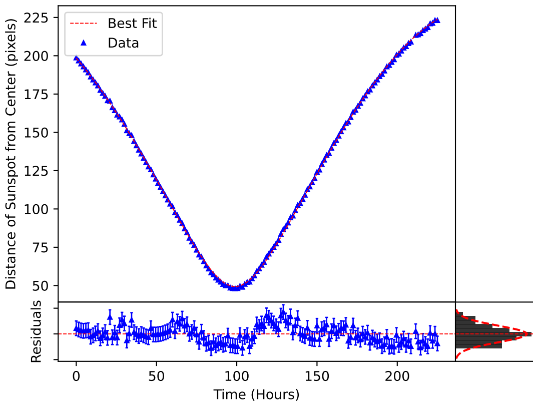
\delta_m(\omega, t) Plotted over the Motion of Sunspot 3738
