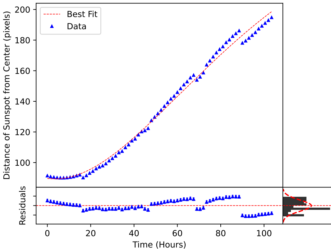
\delta_m(\omega, t) Plotted over the Motion of Sunspot 3740
