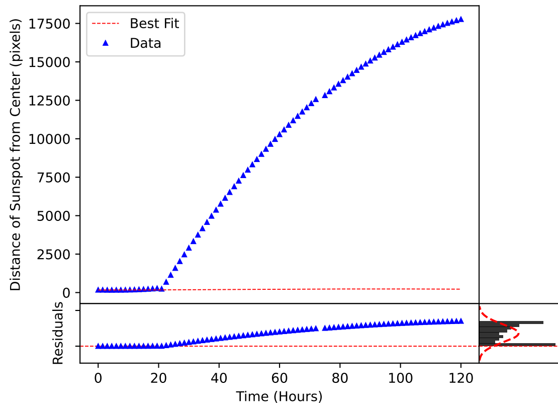
\delta_m(\omega, t) Plotted over the Motion of Sunspot 3693
