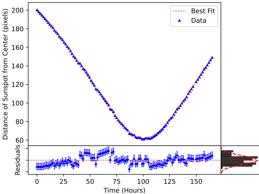
\delta_m(\omega, t) Plotted over the Motion of Sunspot 2795?
