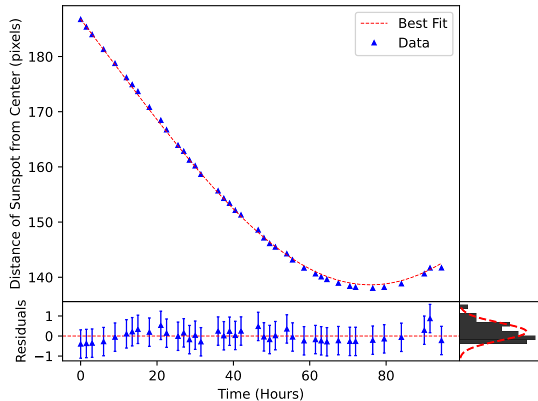
\delta_m(\omega, t) Plotted over the Motion of Sunspot 3639.5
