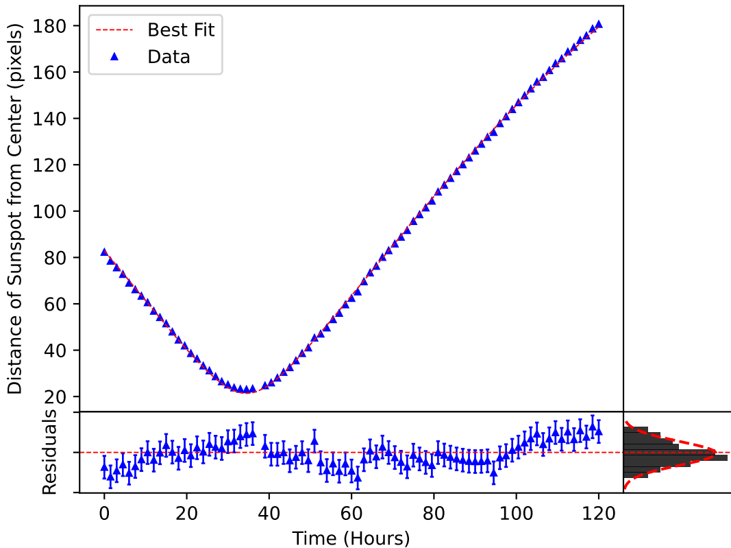
\delta_m(\omega, t) Plotted over the Motion of Sunspot 3693
