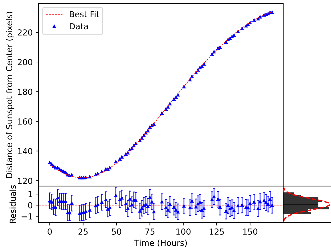
\delta_m(\omega, t) Plotted over the Motion of Sunspot 3634
