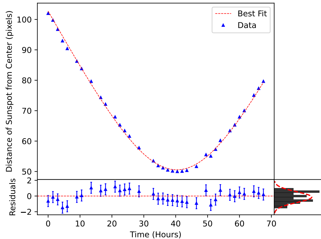
\delta_m(\omega, t) Plotted over the Motion of Sunspot 3582
