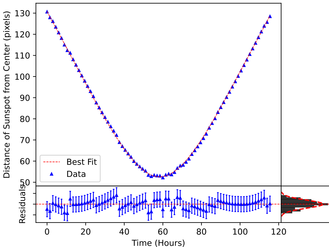
\delta_m(\omega, t) Plotted over the Motion of Sunspot 3735
