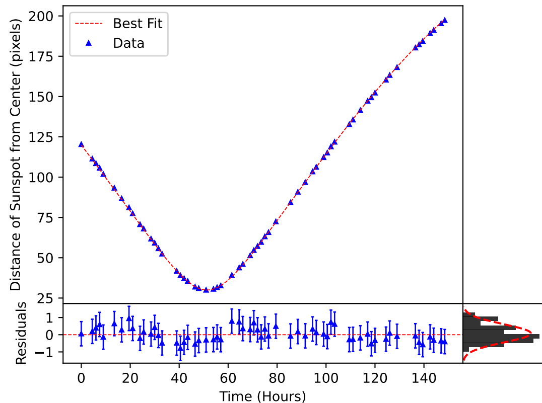
\delta_m(\omega, t) Plotted over the Motion of Sunspot 3555
