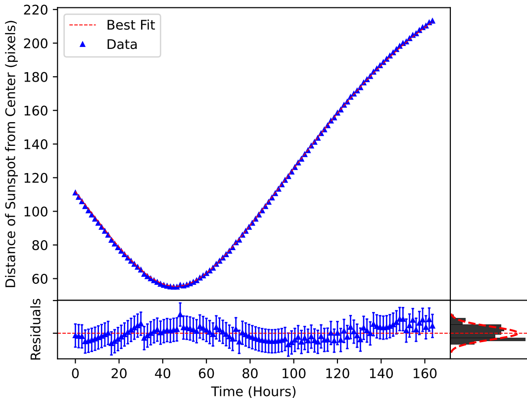
\delta_m(\omega, t) Plotted over the Motion of Sunspot 3722
