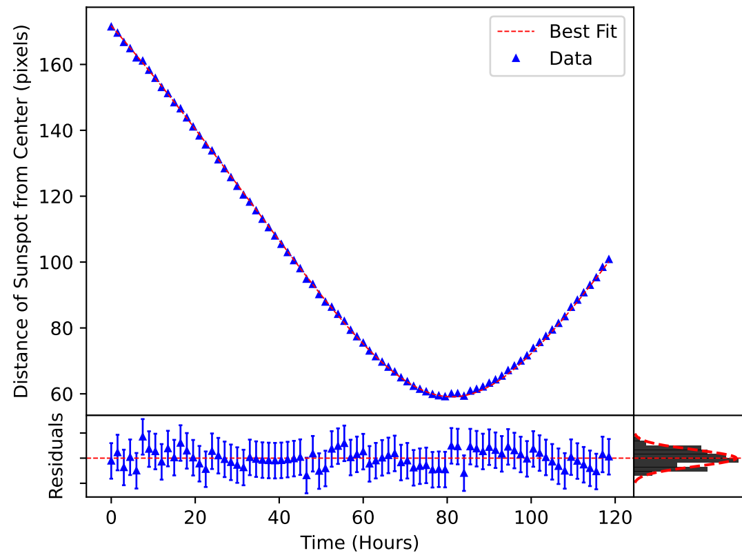
\delta_m(\omega, t) Plotted over the Motion of Sunspot 3713
