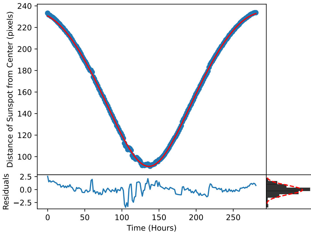
\delta_m(\omega, t) Plotted over the Motion of Sunspot 4217
