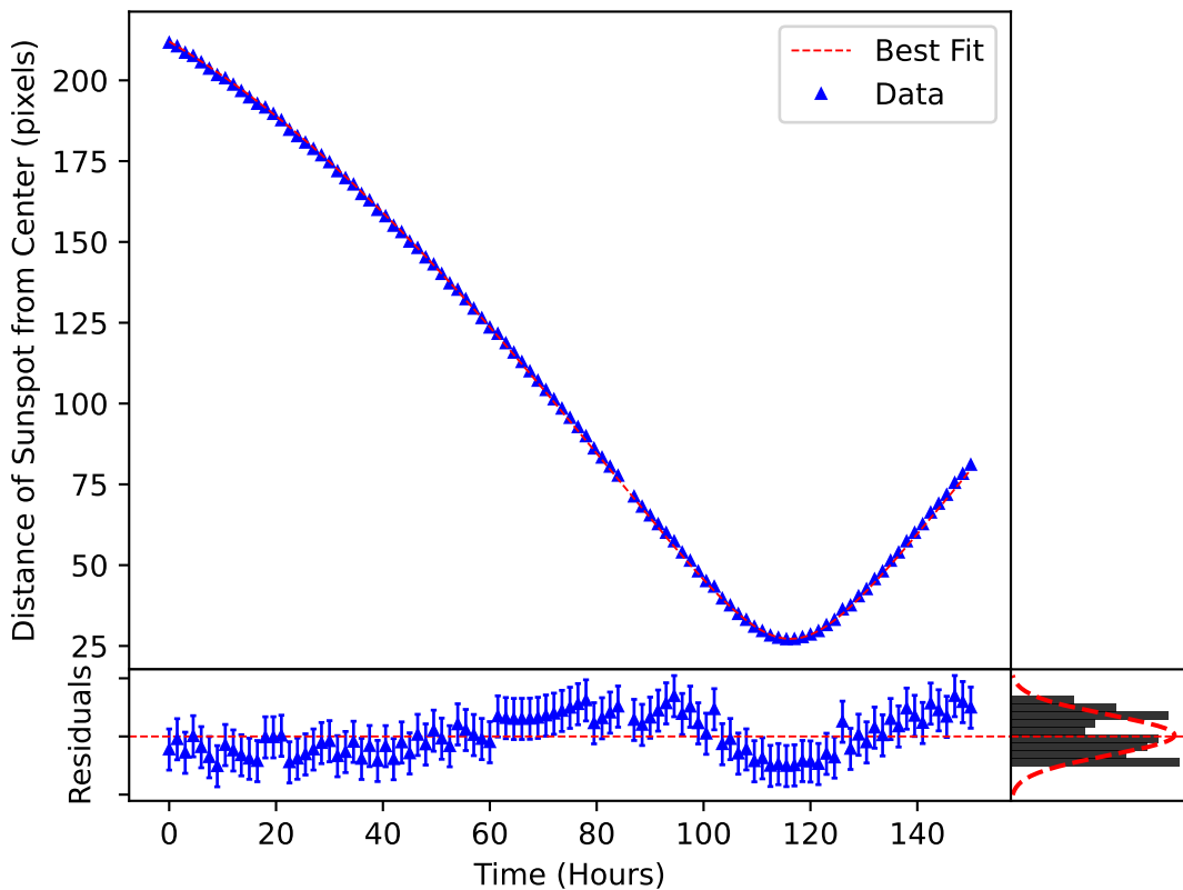
\delta_m(\omega, t) Plotted over the Motion of Sunspot 3673
