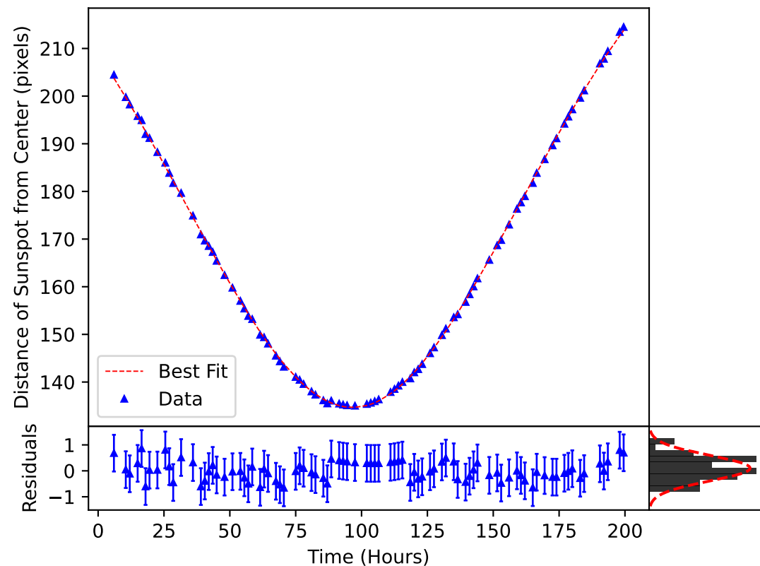
\delta_m(\omega, t) Plotted over the Motion of Sunspot 3586
