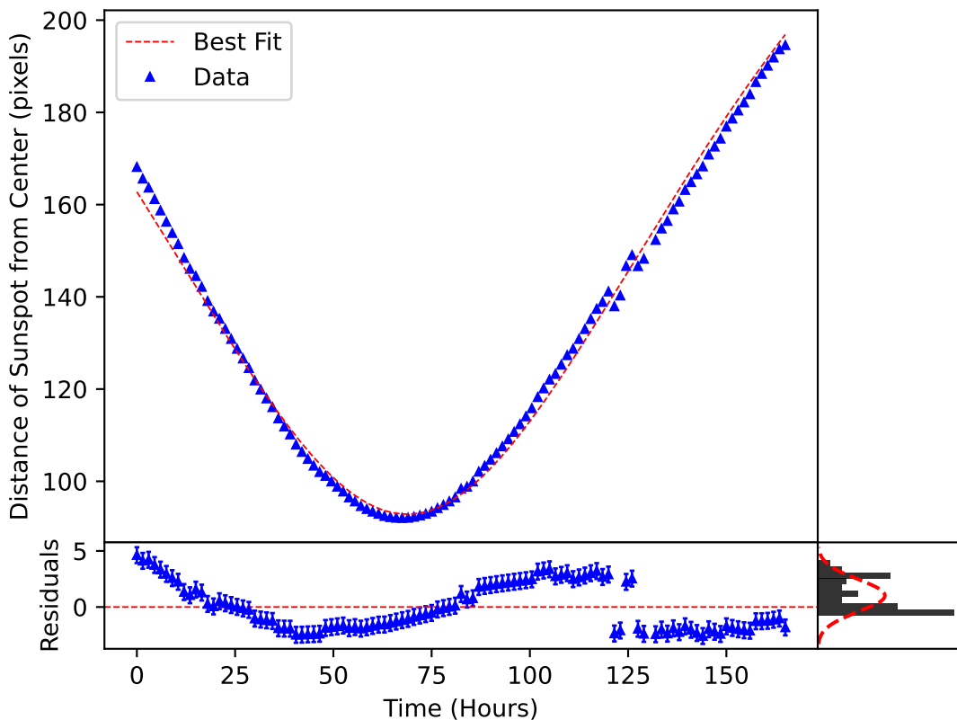
\delta_m(\omega, t) Plotted over the Motion of Sunspot 3671
