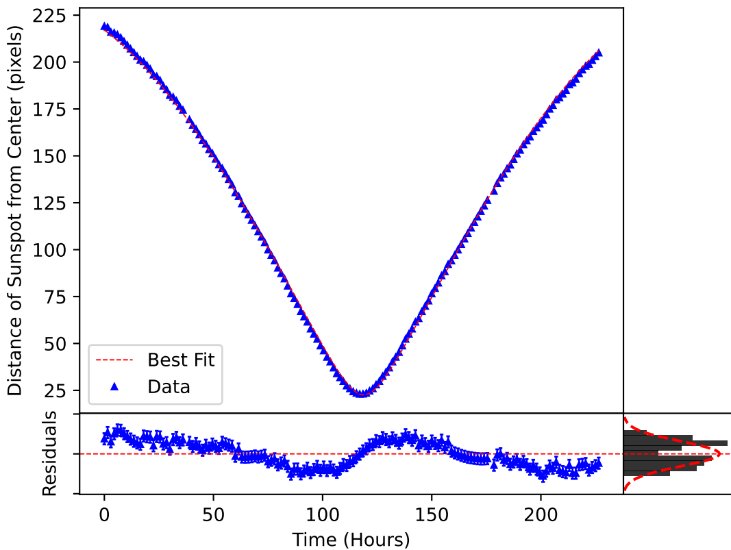
\delta_m(\omega, t) Plotted over the Motion of Sunspot 3679
