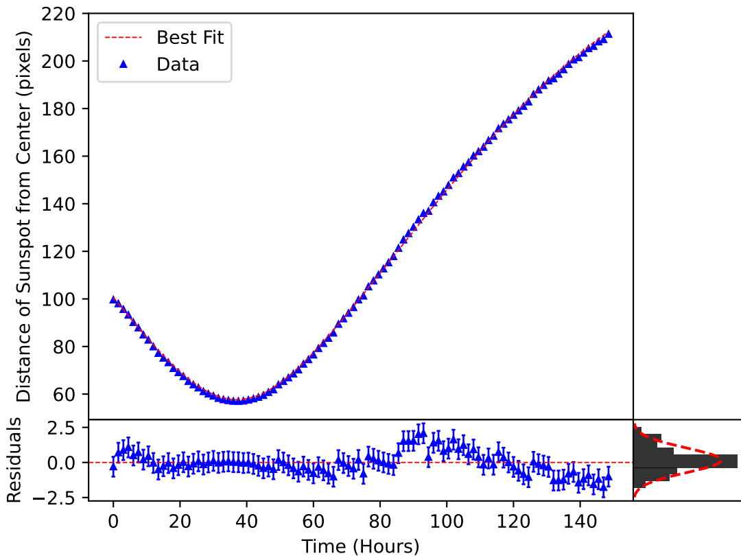
\delta_m(\omega, t) Plotted over the Motion of Sunspot 3664
