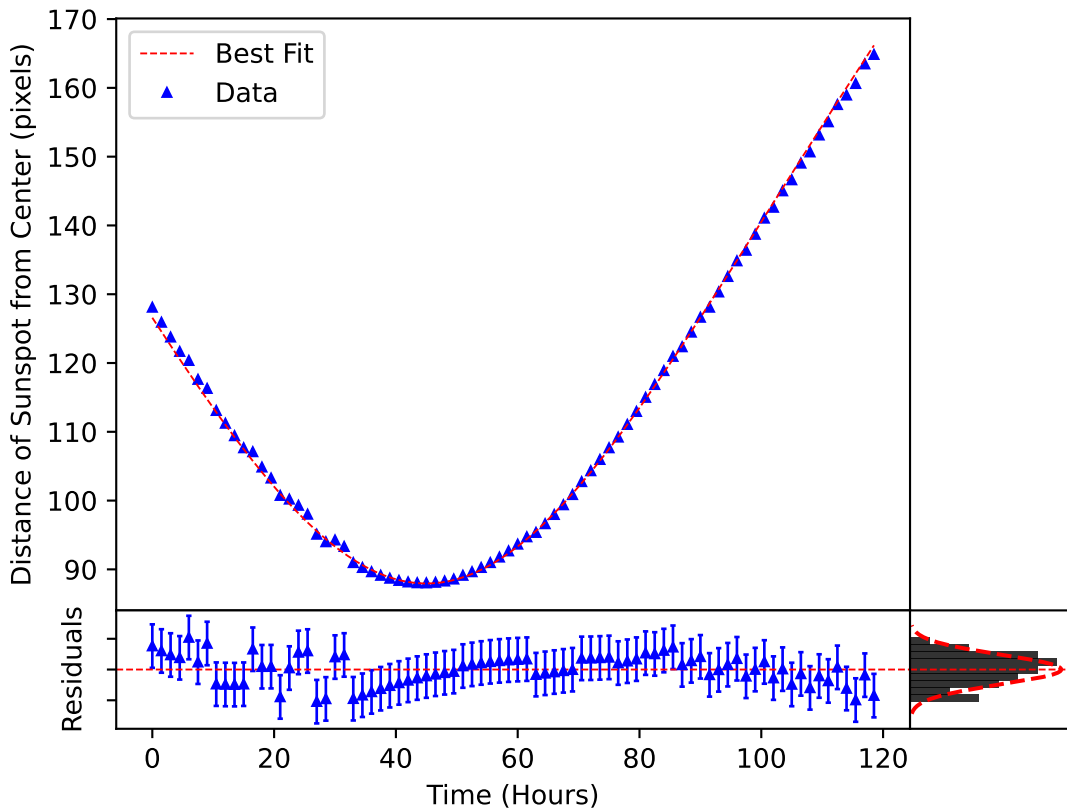
\delta_m(\omega, t) Plotted over the Motion of Sunspot 3698
