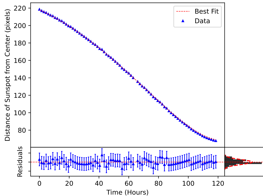
\delta_m(\omega, t) Plotted over the Motion of Sunspot 3702
