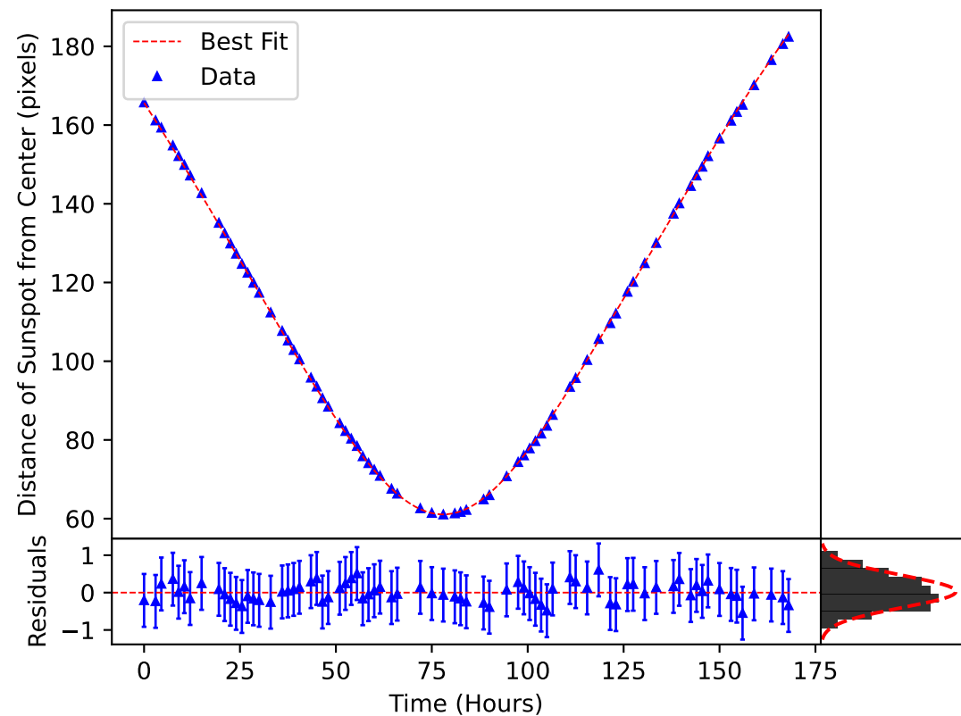
\delta_m(\omega, t) Plotted over the Motion of Sunspot 3581
