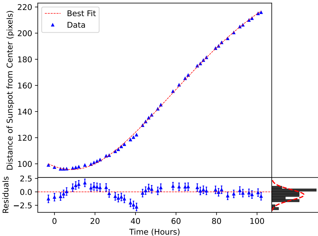
\delta_m(\omega, t) Plotted over the Motion of Sunspot 3621
