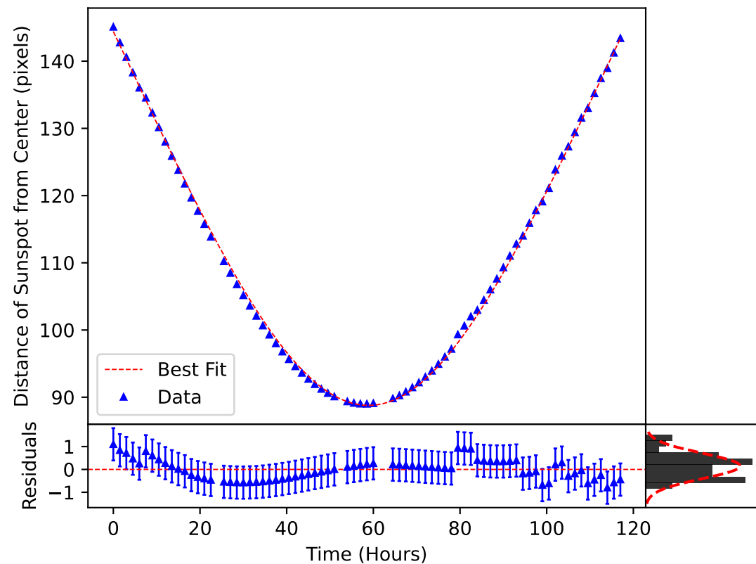
\delta_m(\omega, t) Plotted over the Motion of Sunspot 3655
