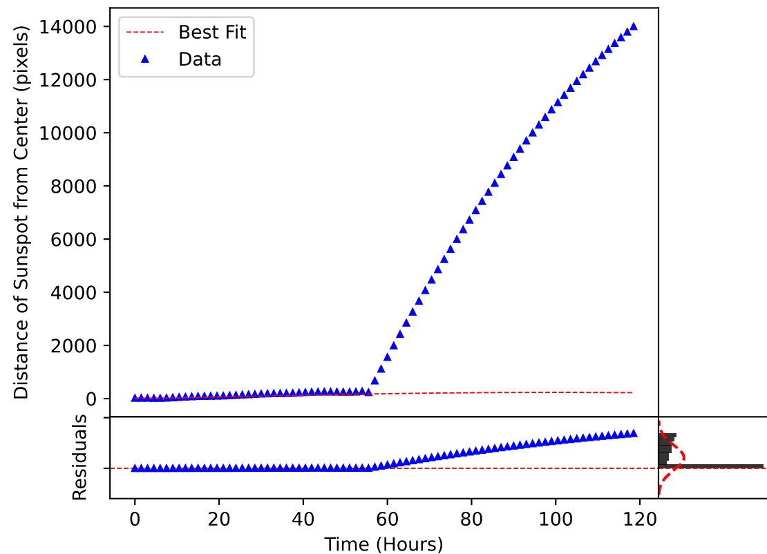
\delta_m(\omega, t) Plotted over the Motion of Sunspot 3699
