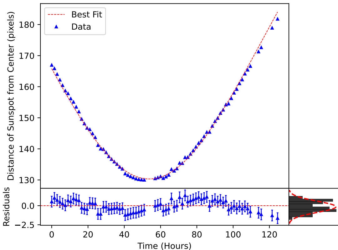
\delta_m(\omega, t) Plotted over the Motion of Sunspot 3662
