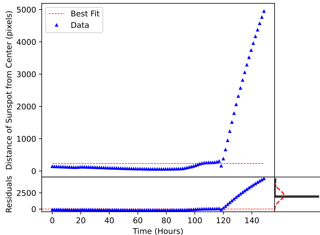
\delta_m(\omega, t) Plotted over the Motion of Sunspot 3669
