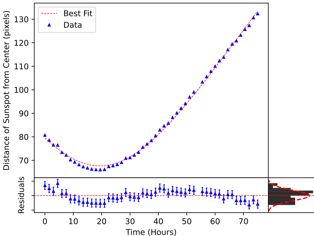
\delta_m(\omega, t) Plotted over the Motion of Sunspot 3676
