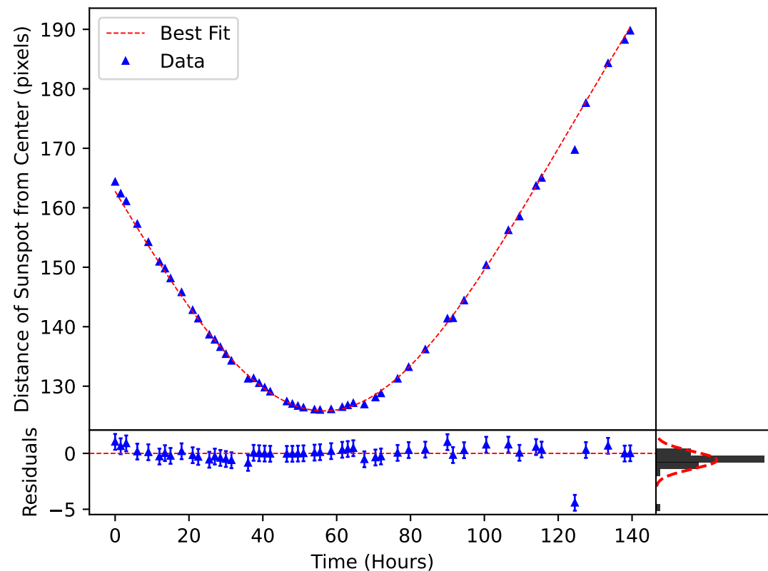
\delta_m(\omega, t) Plotted over the Motion of Sunspot 3639
