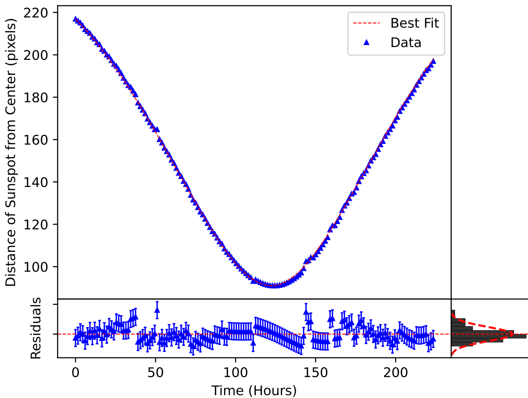
\delta_m(\omega, t) Plotted over the Motion of Sunspot 3721
