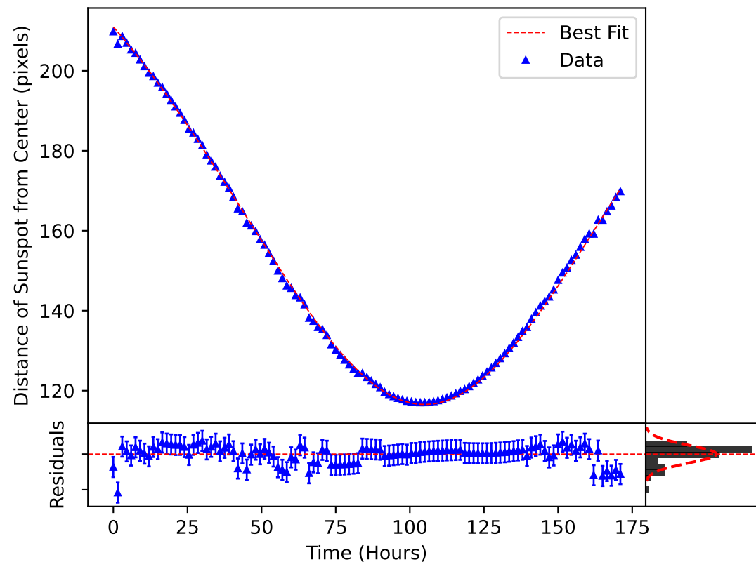
\delta_m(\omega, t) Plotted over the Motion of Sunspot 3728
