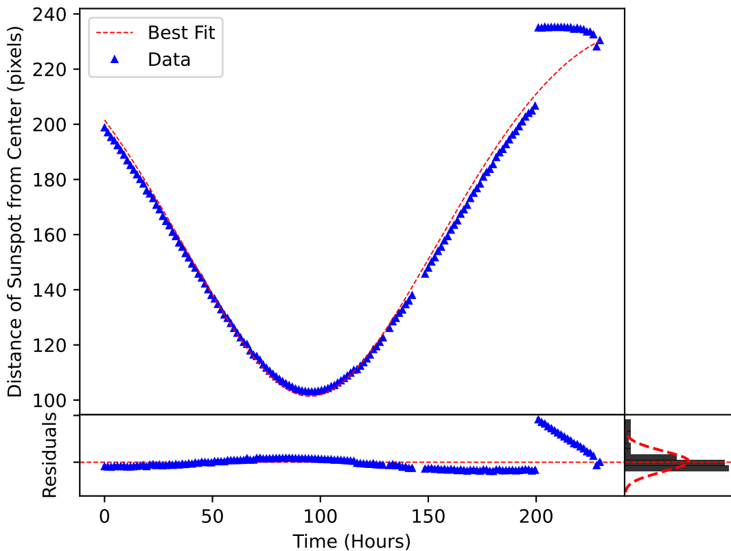
\delta_m(\omega, t) Plotted over the Motion of Sunspot 2767
