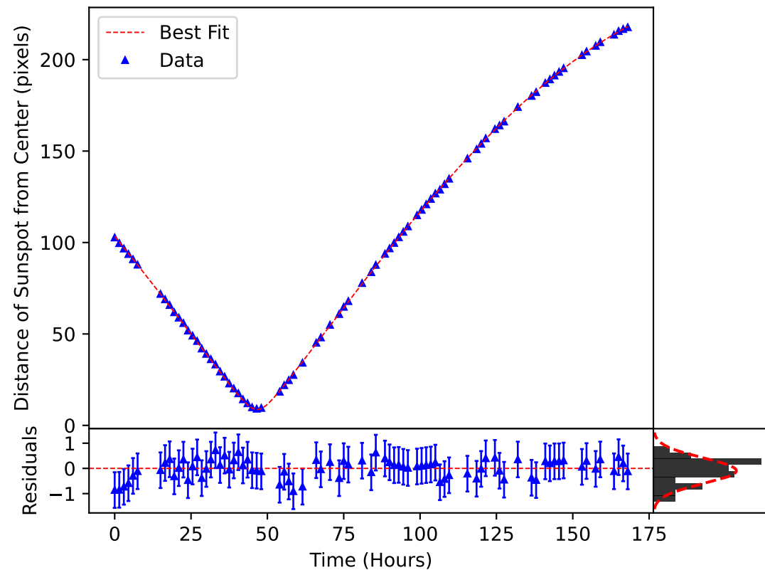
\delta_m(\omega, t) Plotted over the Motion of Sunspot 3633
