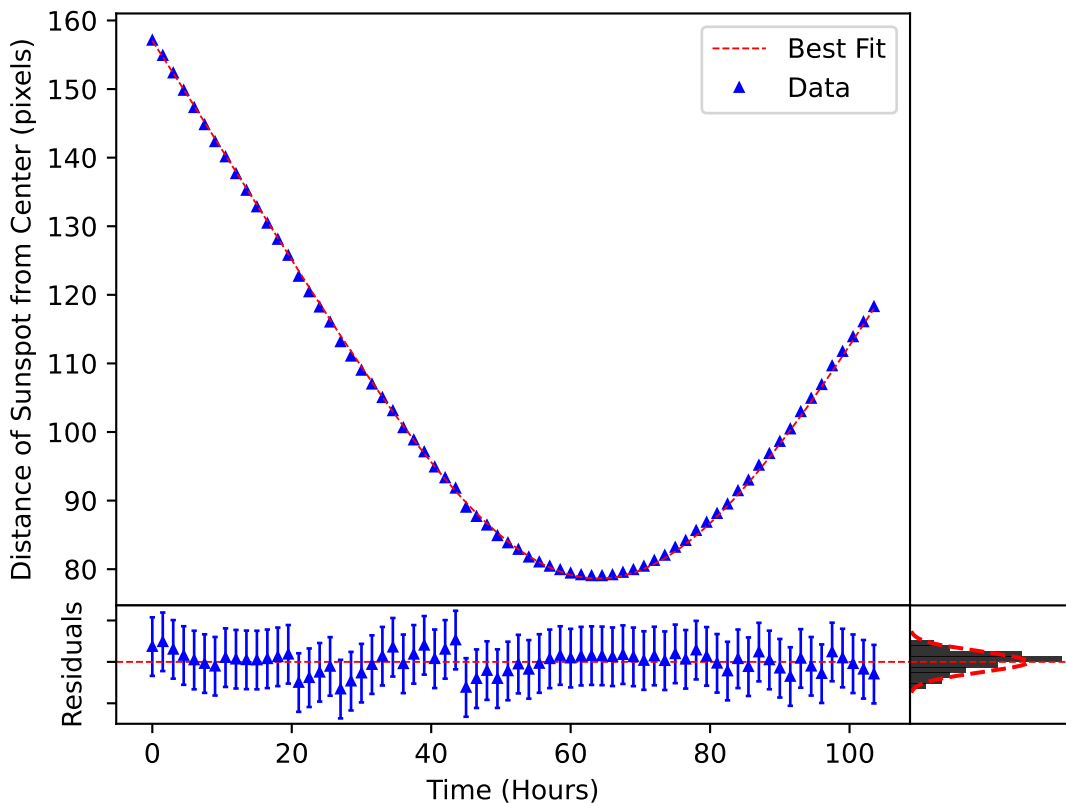
\delta_m(\omega, t) Plotted over the Motion of Sunspot 3723
