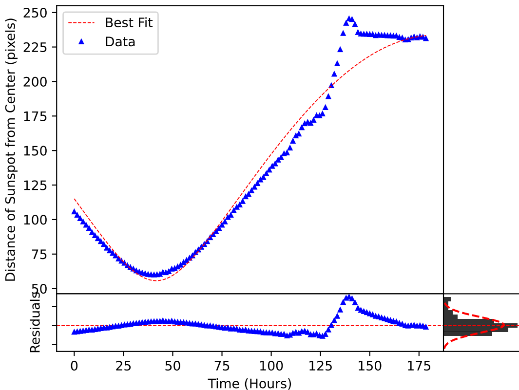
\delta_m(\omega, t) Plotted over the Motion of Sunspot 3707
