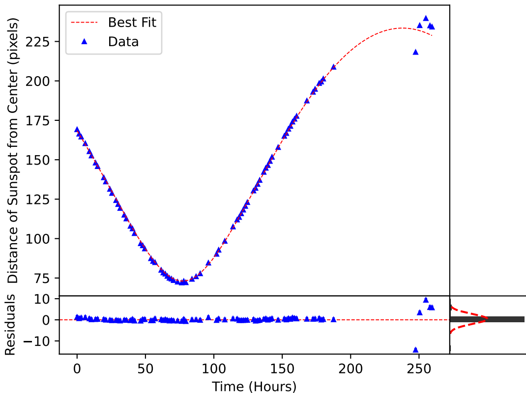
\delta_m(\omega, t) Plotted over the Motion of Sunspot 3719
