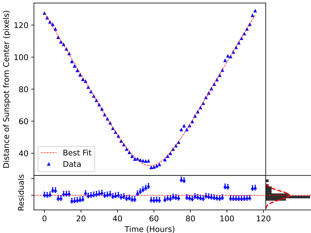
\delta_m(\omega, t) Plotted over the Motion of Sunspot 3703.2
