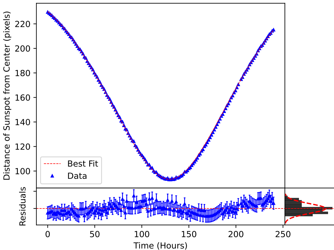
\delta_m(\omega, t) Plotted over the Motion of Sunspot 2790
