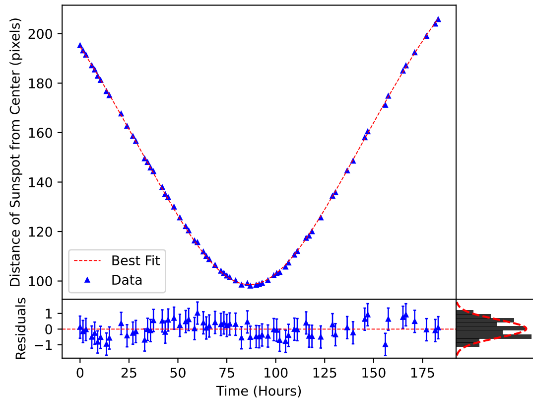
\delta_m(\omega, t) Plotted over the Motion of Sunspot 3619
