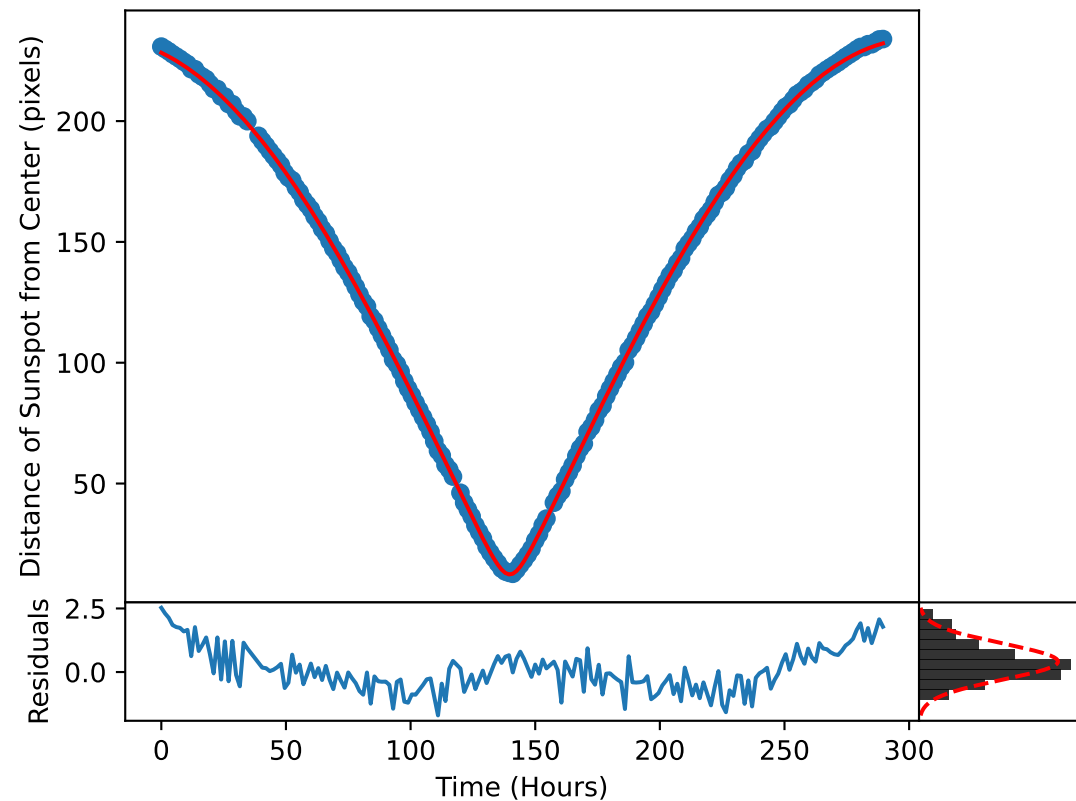
\delta_m(\omega, t) Plotted over the Motion of Sunspot 4225
