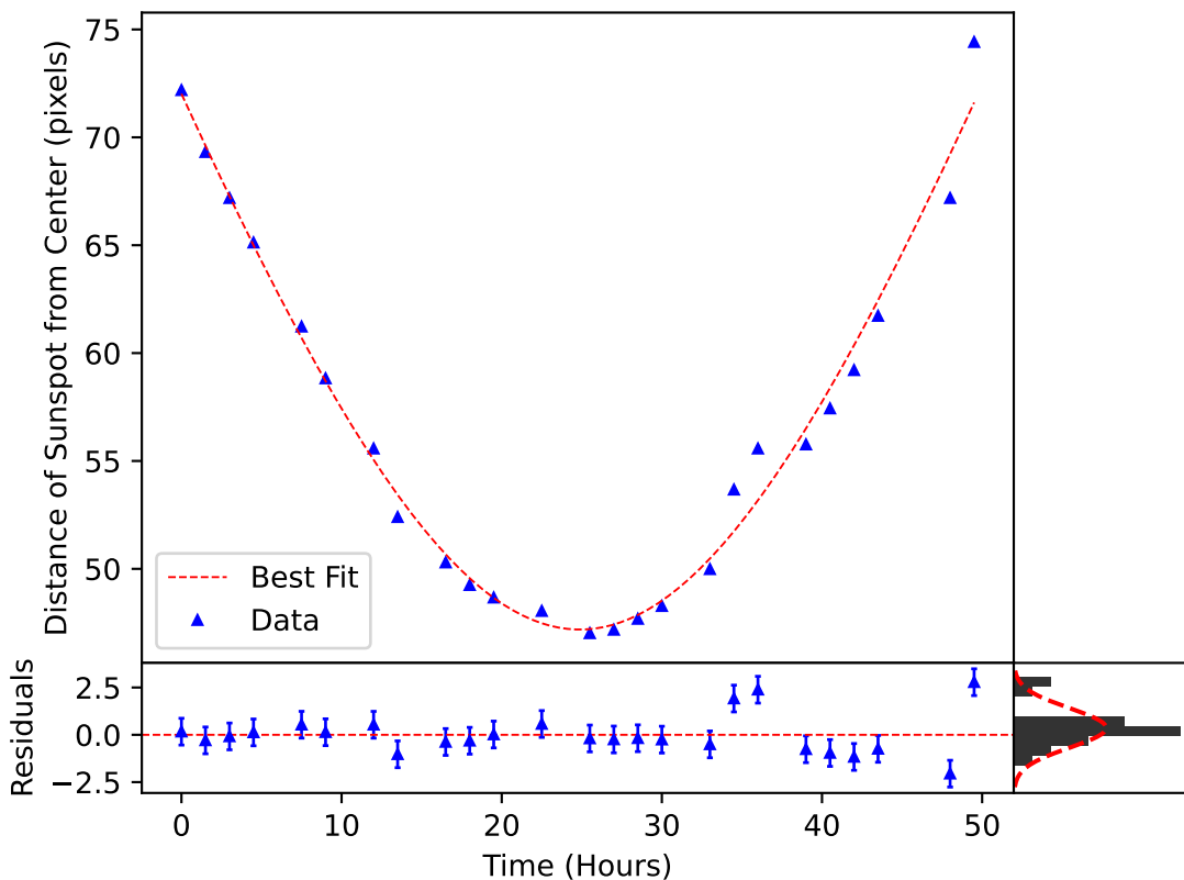
\delta_m(\omega, t) Plotted over the Motion of Sunspot 3600
