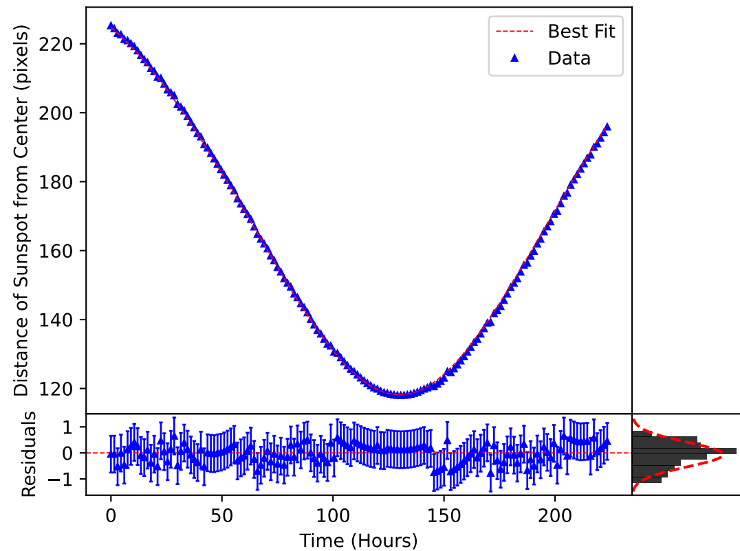
\delta_m(\omega, t) Plotted over the Motion of Sunspot 3667
