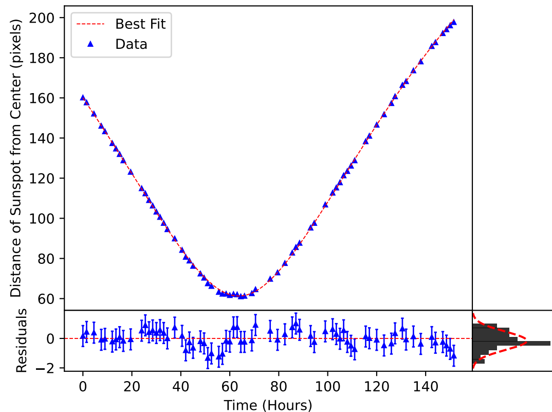
\delta_m(\omega, t) Plotted over the Motion of Sunspot 3583
