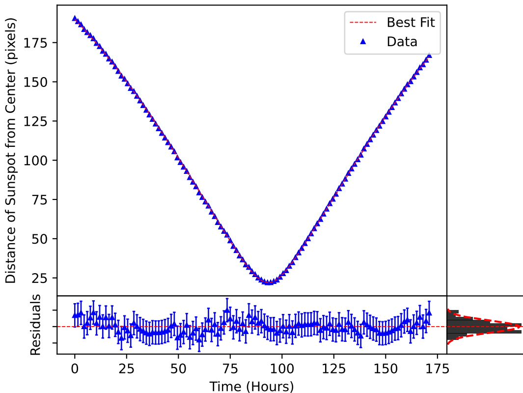
\delta_m(\omega, t) Plotted over the Motion of Sunspot 3729
