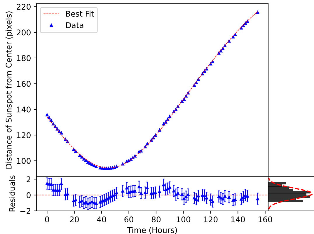
\delta_m(\omega, t) Plotted over the Motion of Sunspot 3602
