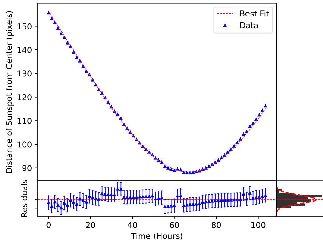
\delta_m(\omega, t) Plotted over the Motion of Sunspot 3708
