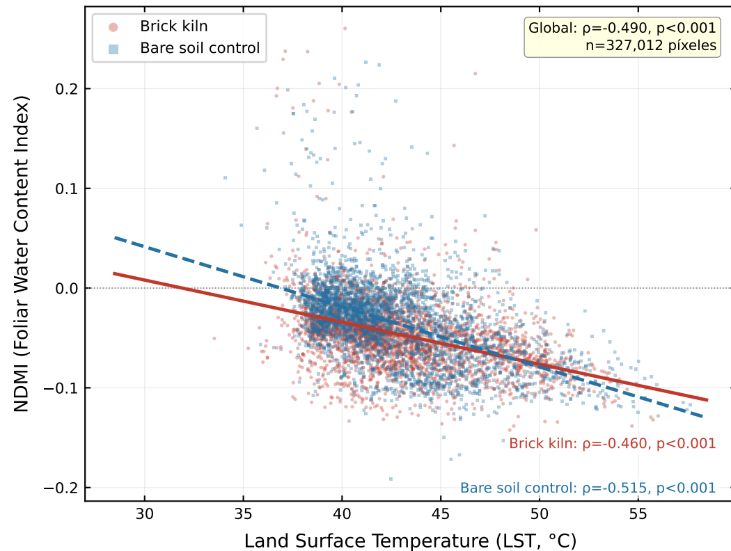
(a) LST vs NDMI — All years combined (2024-2026)
