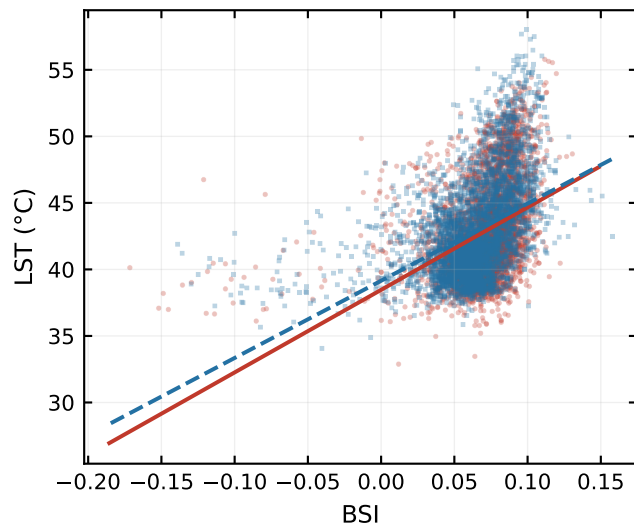
(b) LST vs BSI
