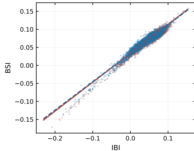
(f) BSI vs IBI
