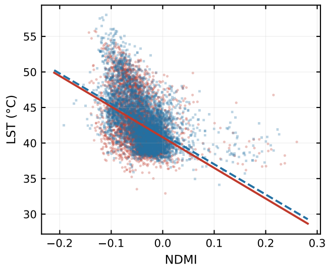
(a) LST vs NDMI
