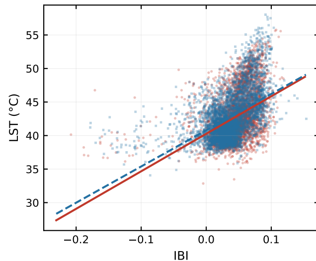
(c) LST vs IBI
