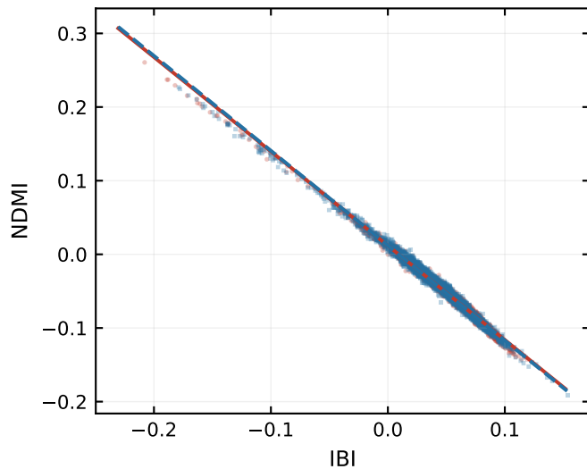
(e) NDMI vs IBI
