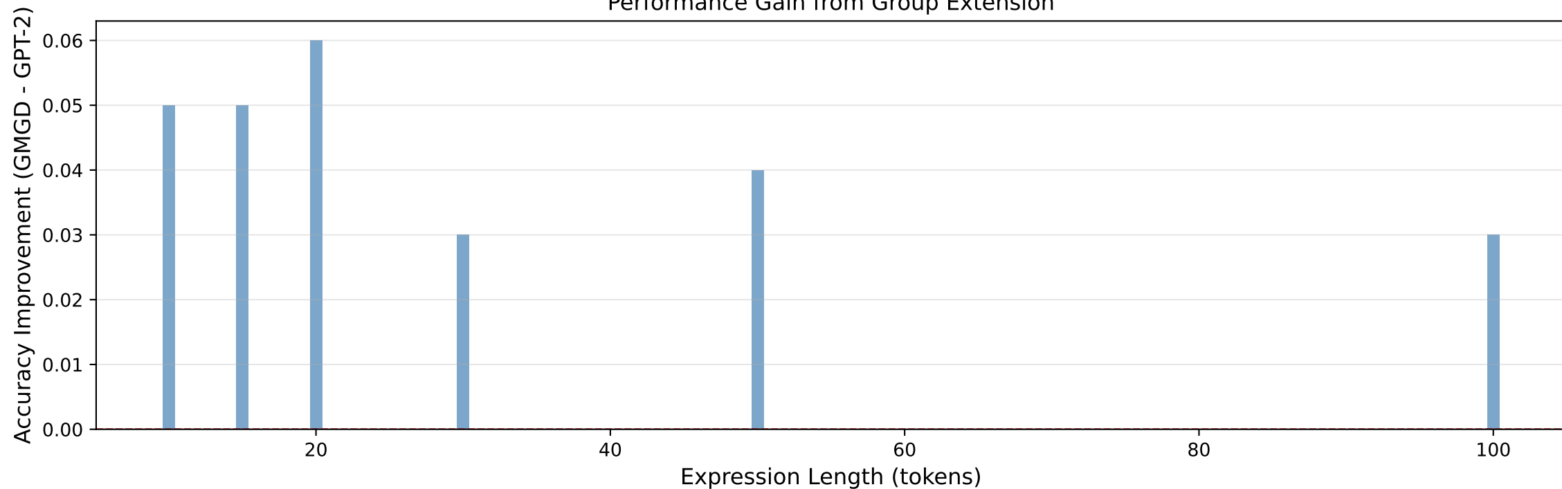
Performance Gain from Group Extension
