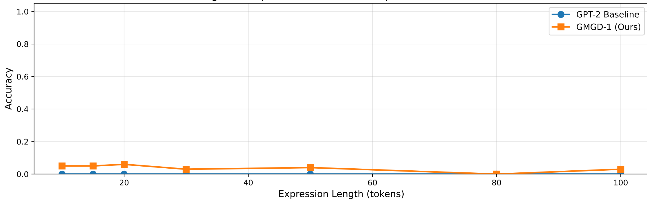
Performance Gain from Group Extension
