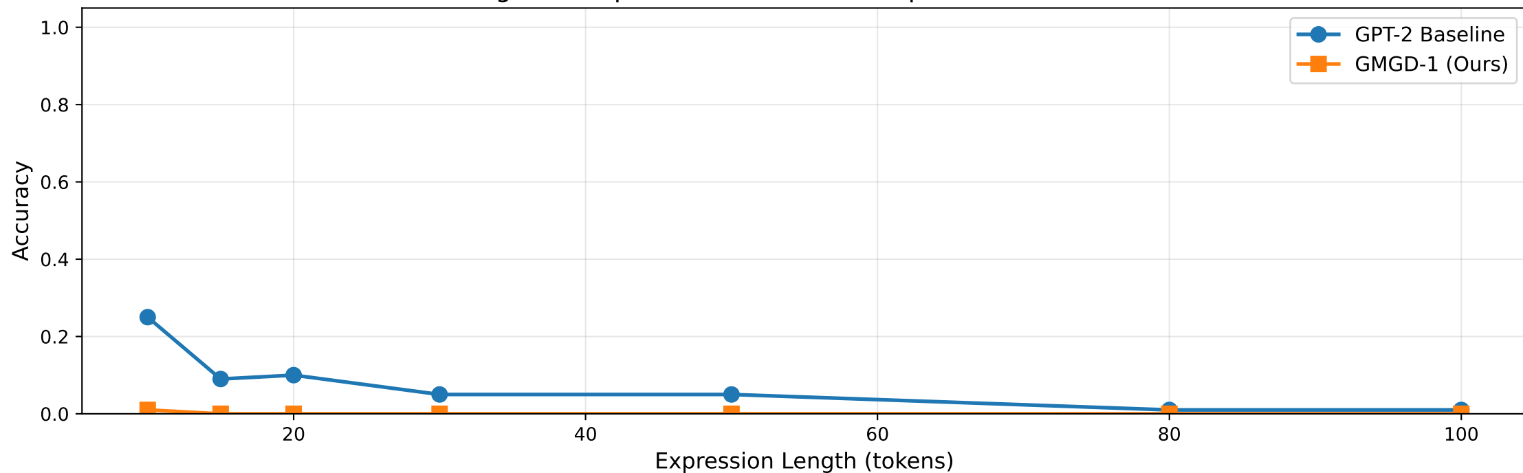
Length Extrapolation: Arithmetic Expression Evaluation
