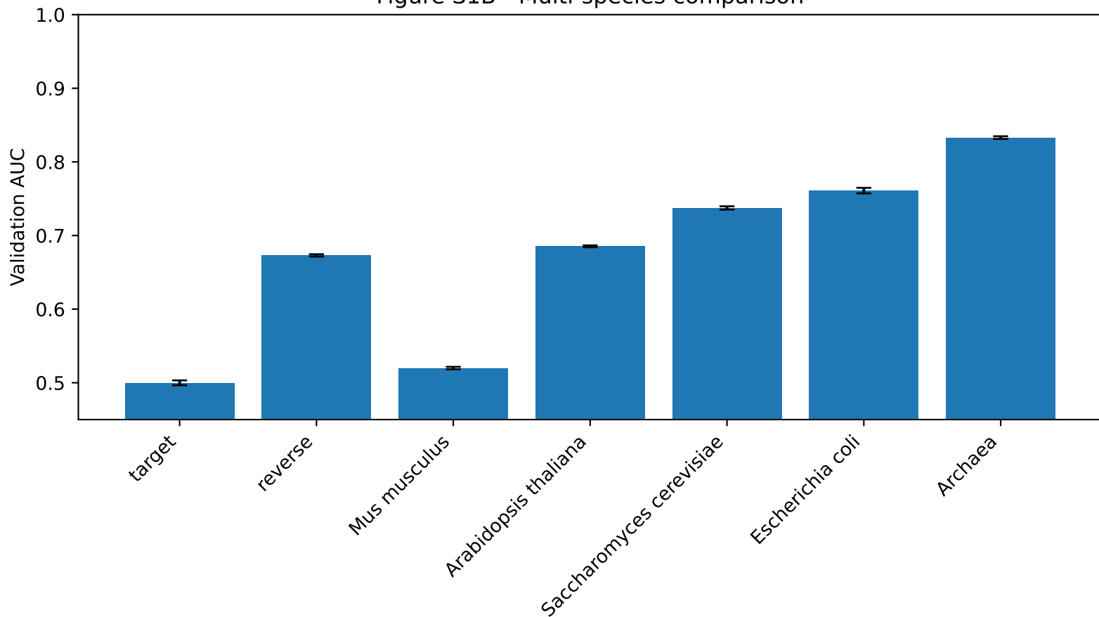
Figure S1B - Multi-species comparison
