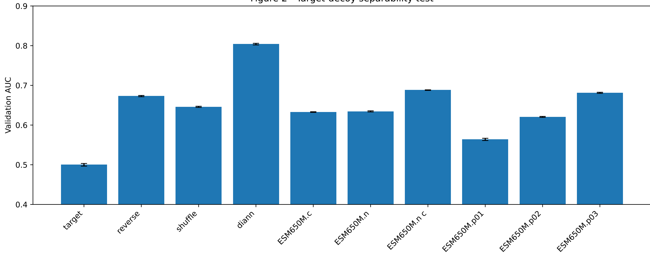
Figure 2 - Target-decoy separability test
