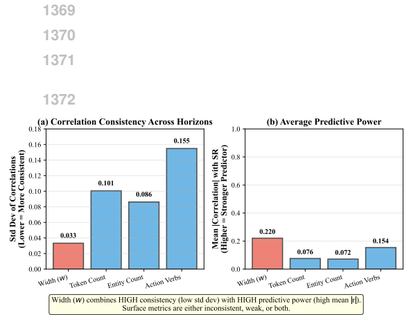
Figure 14: Consistency comparison between instruction width and other linguistic heuristics.
