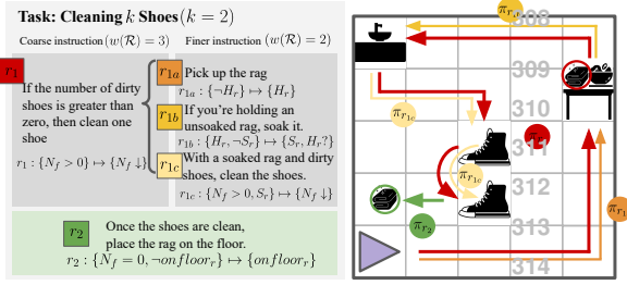
Figure 1: (Left) Factoring r_1 into r_{1a}-r_{1c} reduces latent planning complexity via explicit action guidance. (Right) Fine instructions segment the long-horizon coarse trajectory ( \pi_{r_1} , red).
