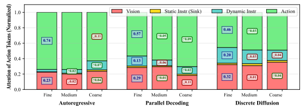
Figure 15: Attention from action tokens. Self-attention dominates, followed by vision; No clear trend across granularity levels.
