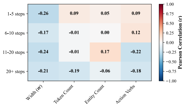
Figure 13: Correlation heatmap between instruction width and other linguistic heuristics.
