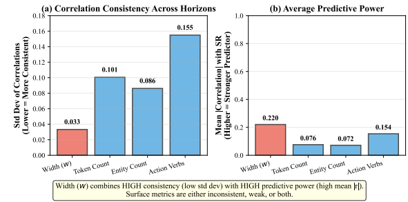
Figure 14: Consistency comparison between instruction width and other linguistic heuristics.
