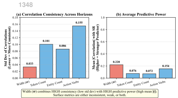
Figure 14: Consistency comparison between instruction width and other linguistic heuristics.
