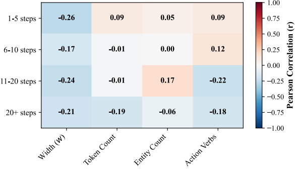
Figure 13: Correlation heatmap between instruction width and other linguistic heuristics.
