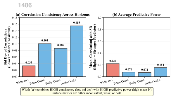
Figure 13: Consistency comparison between instruction width and other linguistic heuristics.
