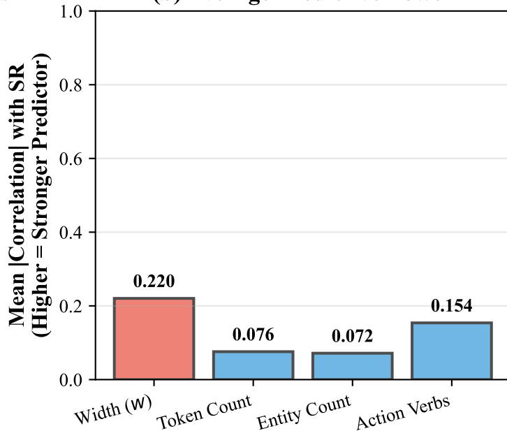
(b) Average Predictive Power
