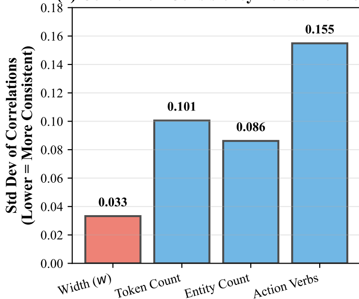
(a) Correlation Consistency Across Horizons
