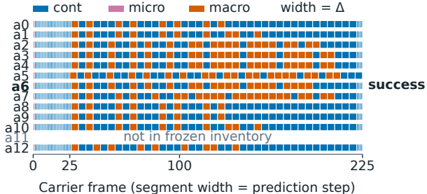
(a) Requests chosen while imagining each launch
