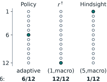
(b) Rank of each launch by predicted cost
