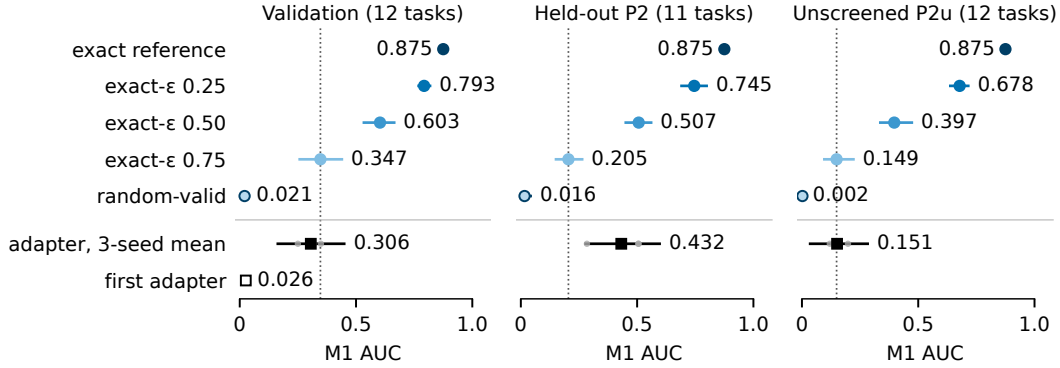
Figure 2: M1 solve-versus-budget AUC with task-clustered 95% intervals on the validation panel, the held-out panel P2, and the unscreened panel P2u, for the five ladder arms and the three-seed adapter mean (per-seed points faint). Ladder rungs read the privileged heap head.
