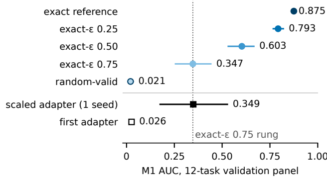
Figure 2: M1 solve-versus-budget AUC on the 12-task validation panel, with task-clustered 95% intervals. Ladder rungs read the privileged heap head. The scaled adapter (single seed) sits at the exact- \epsilon 0.75 rung on point estimates.
