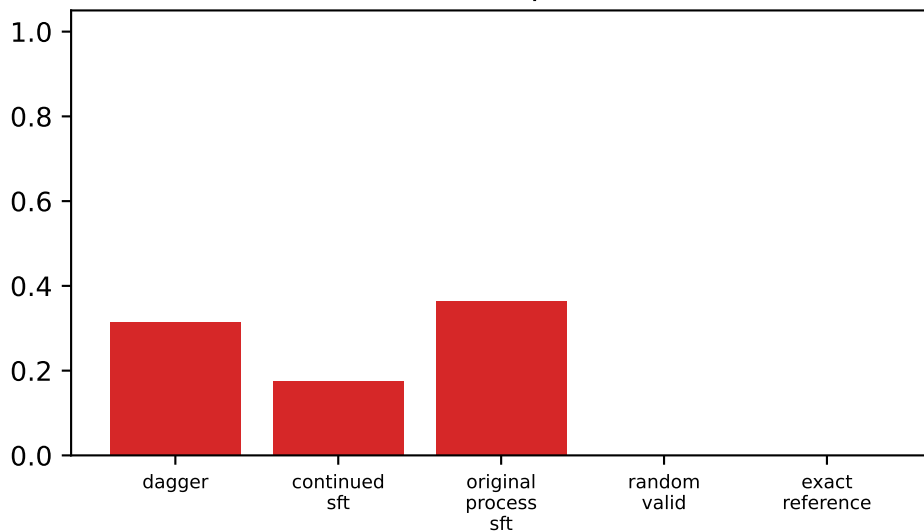
Unseen invalid-operation rate
