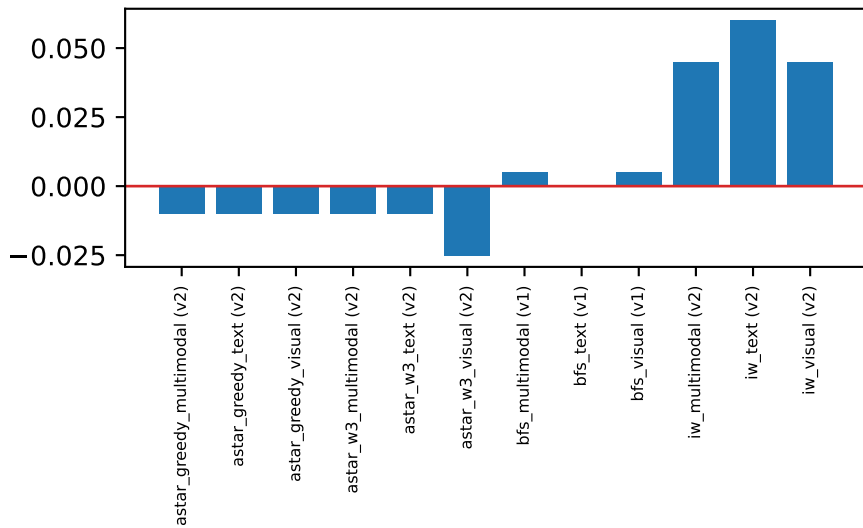
folio (base 0.600)
