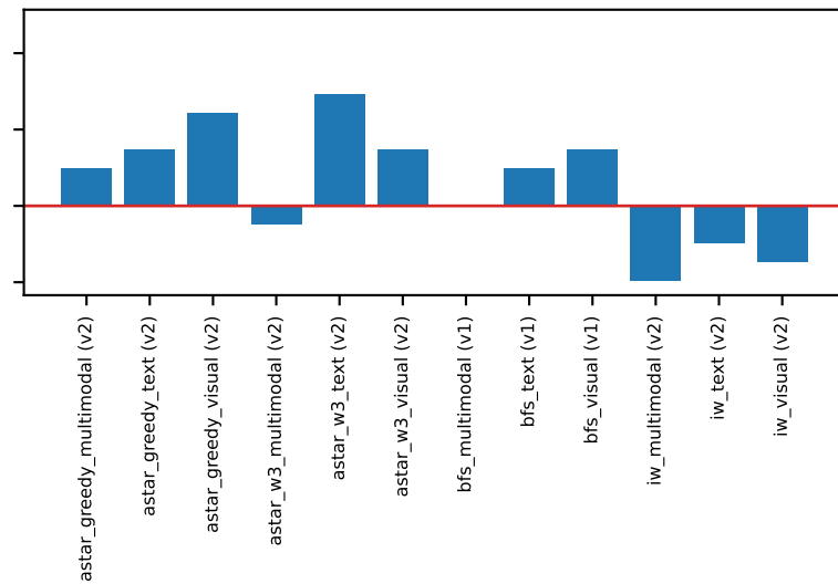
humaneval (base 0.780)
