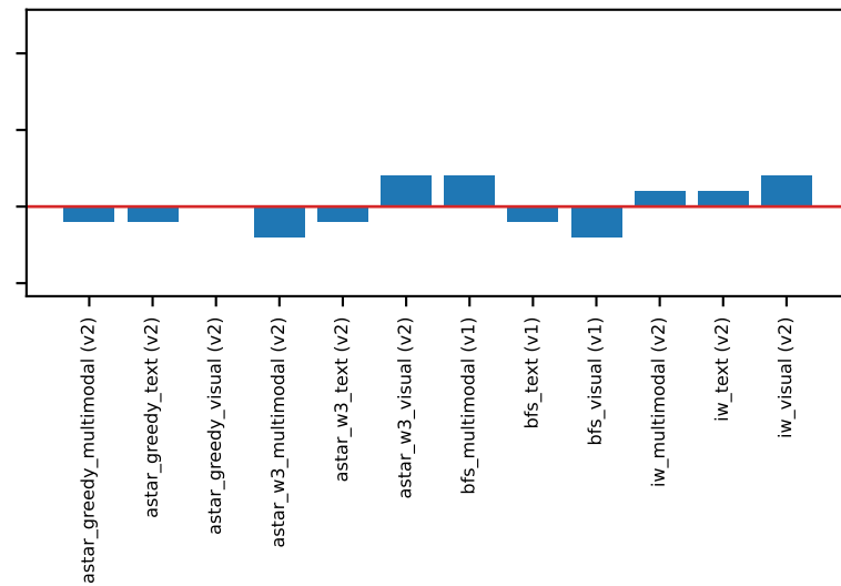
gsm8k (base 0.955)
