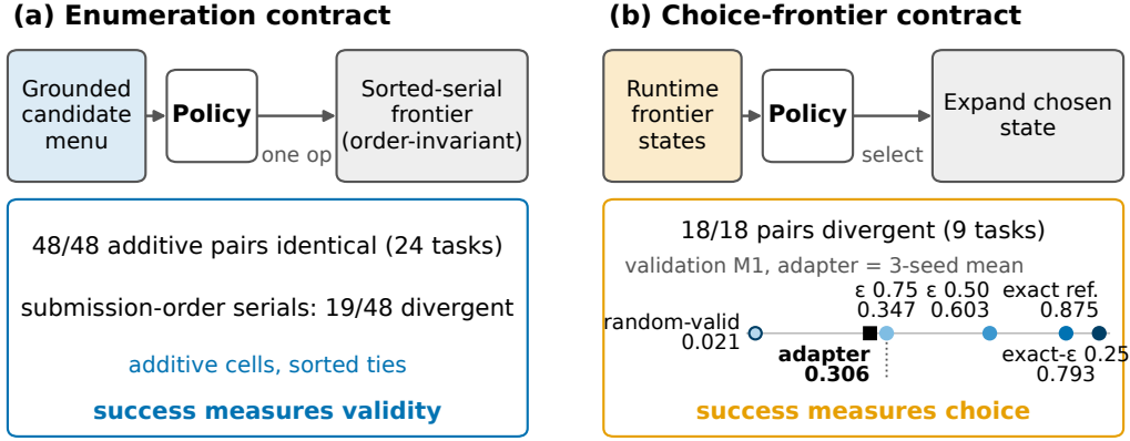
Figure 1: Validate before score. Random-valid success measures choice only on an interface where its decisions can diverge from the exact reference’s, and the measure must order privileged reference-derived selectors before it scores any policy. (a) Under the enumeration contract, random-valid makes the exact reference’s decisions on 48/48 additive pairs, and 19/48 pairs diverge when ties break in submission order. (b) Under the choice-frontier contract, 18/18 pairs on the reused 9-task panel diverge. On the validation panel, M1 falls from 0.875 for the exact reference, a value fixed by construction, through the exact- \epsilon rungs, which randomize a fraction \epsilon of reference decisions, to 0.021 for random-valid (point estimates, with intervals in Figure 2). The adapter’s three-seed mean is 0.306. Success therefore measures validity in the additive cells of (a) under sorted tie-breaking and choice in (b), and the rungs read privileged information. The BFS and BFWs cells of (a) and submission-order ties register choice (Section 5.1).
