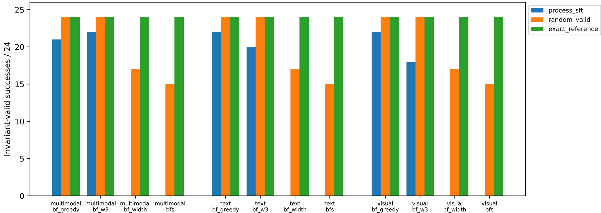
Expanded baseline: 24 problems x 4 algorithms x 3 modalities, one training seed
