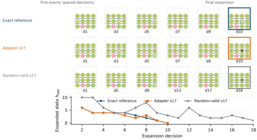
Figure 7: On a solved validation task, the adapter follows the reference to the goal. In this rule-selected weighted-A* episode, the seed-17 adapter agrees with the reference on 7/9 comparable decisions, and both reach the goal at decision 10, while random-valid exhausts its decision cap at 18. Rows show expanded scenes, and the plot traces their h_{add} after the first expansion. The example is illustrative, not an efficacy estimate.
