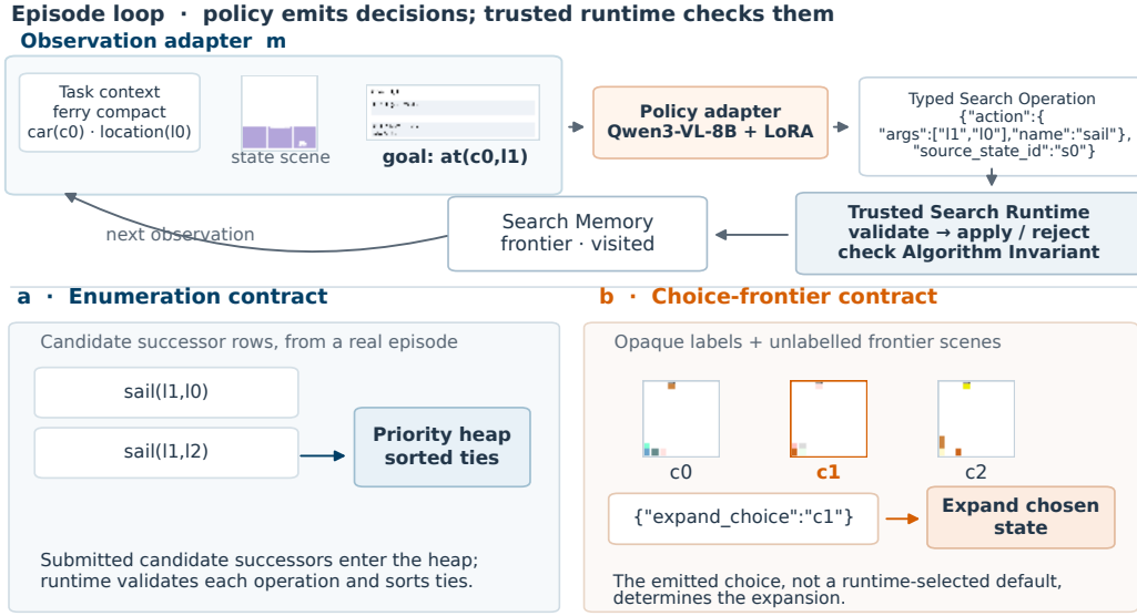
Figure 2: The policy emits typed decisions, and the runtime owns the checks and Search Memory. The runtime validates, applies, or rejects each emitted operation without repair (top). (a) Under enumeration, submitted candidates enter a priority heap that sorts ties. (b) Under choice-frontier, the policy’s choice of an opaque label determines the expanded state.
