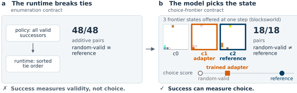
Figure 1: Success reflects choices only if they change the search. (a) On additive tasks, runtime tie-breaking makes random-valid (uniform valid choices) reproduce exact search. (b) When the model picks the state to expand (one illustrative blocksworld step), random-valid and exact search diverge, and a trained adapter scores between them.
