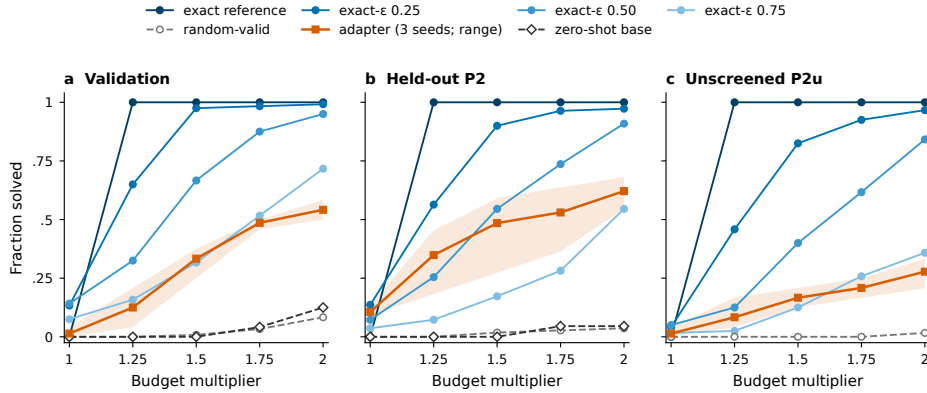
Figure 5: Solved fraction against decision budget. On all three panels the privileged rungs fall in order between the reference and random-valid, and the trained adapter’s area exceeds random-valid’s. Panels are validation, held-out (P2), and unscreened (P2u, descriptive), and the zero-shot base appears where measured. The adapter band is its three-seed range, not a confidence interval. Areas under these curves are M1, and the privileged rungs test only their own reference–random axis.
