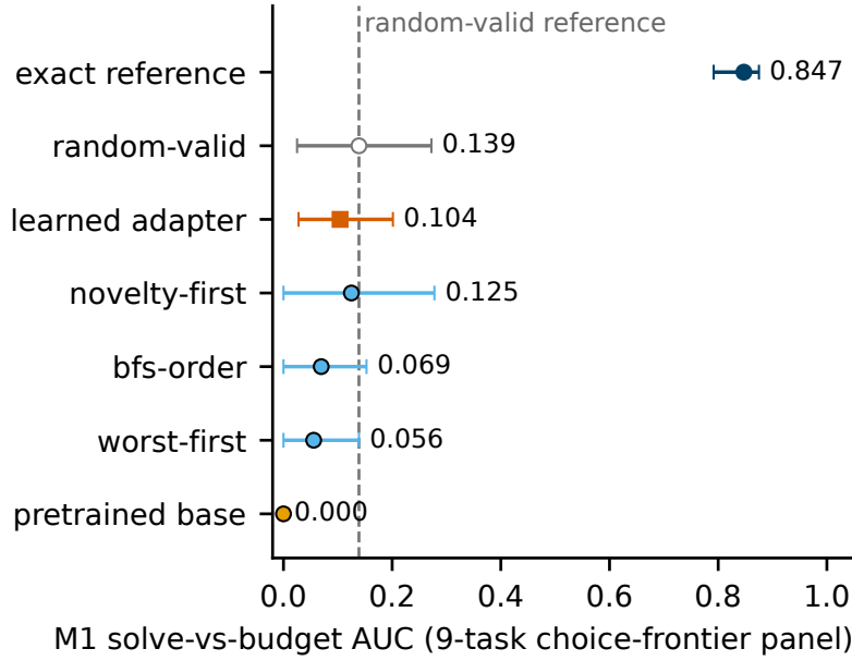
Figure 4: Only the exact reference stands apart on M1 (solve-versus-budget AUC at multipliers 1 to 2) on the frozen 9-task choice-frontier panel. The intervals of all non-exact arms overlap, and the Holm family licenses no ordering. Exact reference .847, random-valid uniform-choice reference .139, learned adapter .104 [.028, .201], novelty-first .125, bfs-order .069, worst-first .056, pretrained base 0. Under the enumeration contract, by contrast, the BFS/BFWS random-valid rows (15/24 and 17/24 versus exact 24/24) already registered choice.
