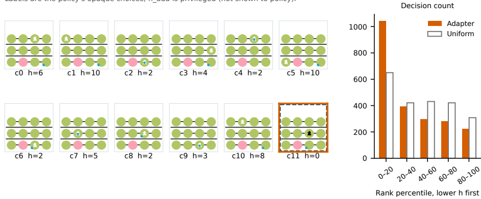
Figure 8: The adapter picks the reference's state at the episode's largest menu and prefers low- h_{add} states overall. At decision 10 of Figure 7, the adapter and the privileged reference both select c_{11} from 12 choices. The policy sees only opaque labels and scenes, not the heuristic values or the reference pick. The histogram describes the adapter's heuristic ranks across validation decisions against uniform choice on the same menus and is not an efficacy estimate.
