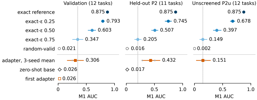
Figure 3: M1 orders the privileged rungs on all three panels. Points give M1, the area under the solve-versus-budget curve, with task-clustered 95% intervals, and faint points give the adapter’s three seeds. Only on the held-out panel (P2) does the adapter’s interval lie entirely right of the dotted \epsilon=0.75 line. The rungs read privileged information, so the ladder validates the measurement, not a policy. The unscreened ladder (P2u) is descriptive.
