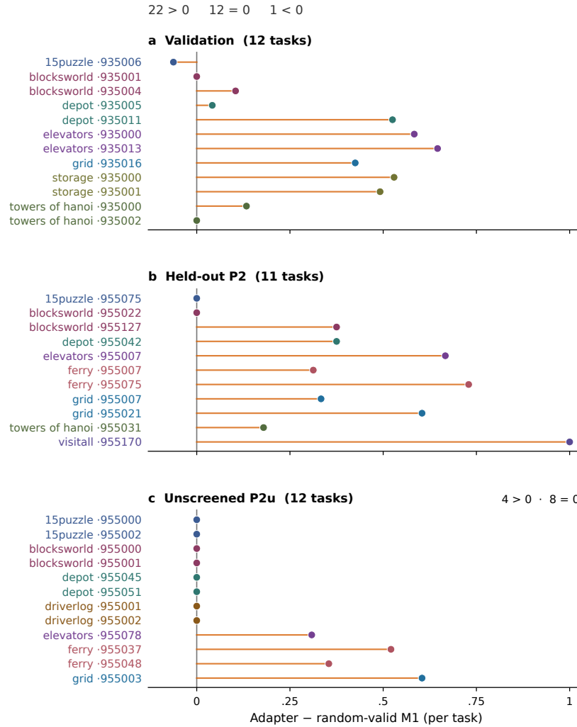
Figure 6: Descriptive task-level choice-frontier gains. Most tasks gain, and the unscreened panel’s improvement is concentrated on four tasks. Each point is the three-seed adapter mean minus random-valid M1, averaged across the two additive algorithms for a task, and colours identify domains. These points are not task-level significance tests.
