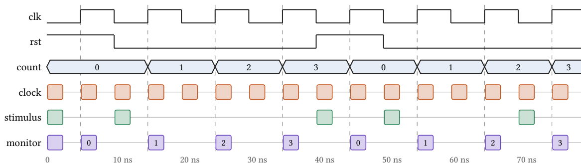
Figure 5: CounterTest with three processes, simulated. The upper rows are the VCD; each lower row marks the moments a process ran, between which it was suspended in an await . The monitor's marks carry the count it printed. All three share one host thread; at a shared time they run in a fixed order, so a run always reproduces.
