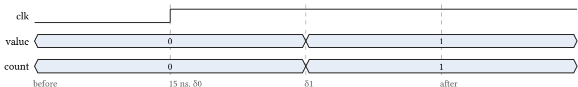
Figure 4: The clock edge at 15 ns in Counter , one column per delta cycle. The simulator confirms it: a process woken by value changing already sees the new count .
