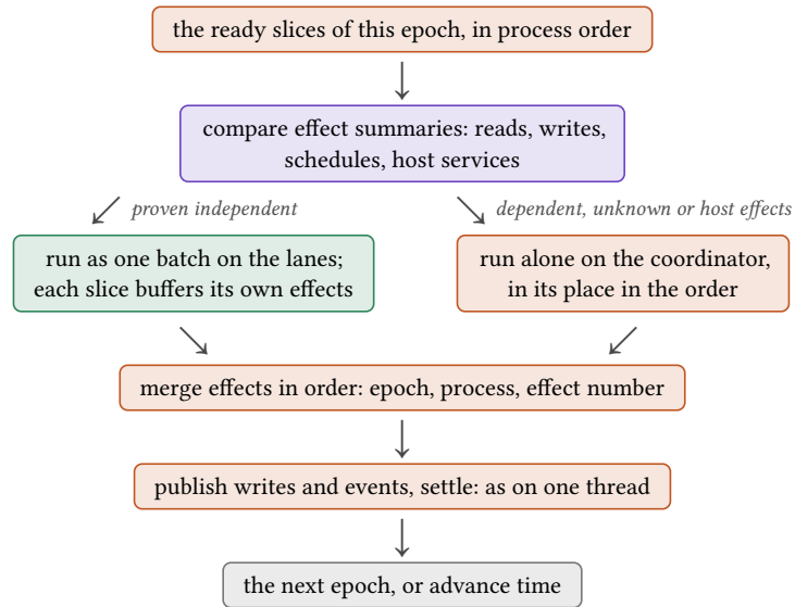
Figure 10: How the proposed runtime dispatches an epoch. Only slices proven independent reach the workers; everything else keeps its serial place. The merge and publication steps are the ones a single thread already performs.
