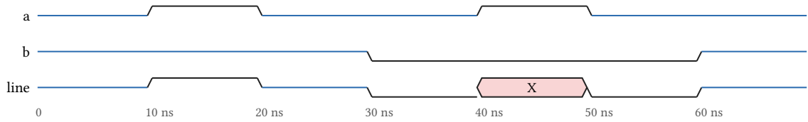
Figure 2: Two drivers of one Logic line, from the simulator's VCD. A released driver ('Z') yields to the other; when both drive, '1' against '0' resolves to the unknown 'X', and the line floats at 'Z' when neither does.
