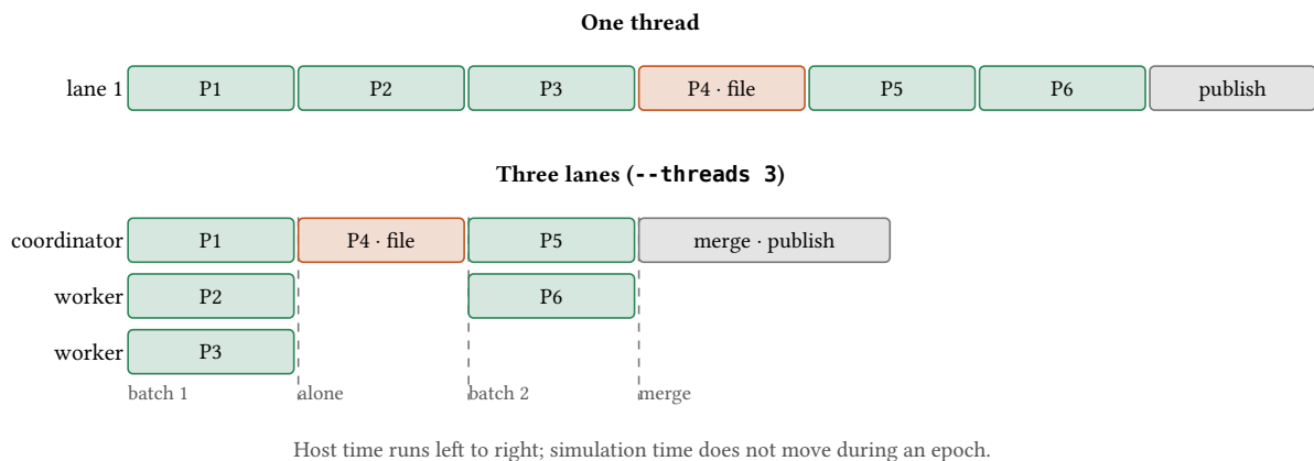
Figure 9: One epoch on one thread and on three lanes. P4 reads a file, so it runs alone, between the batches before and after it. The coordinator merges every slice's effects in process order before publishing, so both runs end in the same state.
