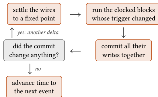
Figure 3: One delta cycle, repeated until a commit changes nothing; only then does time advance.
