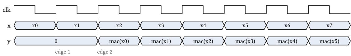
Figure 7: The intended timing of y = mac(...) with #[latched(2)] (a proposal; not simulated). Before the first result arrives, y holds its type's default.
