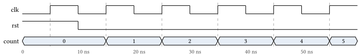
Figure 1: The first 60 ns of CounterTest , drawn from the VCD the test executable writes. The clock rises at 5 ns and every 10 ns after; the edge at 5 ns still sees reset, so the count starts at the edge at 15 ns.
