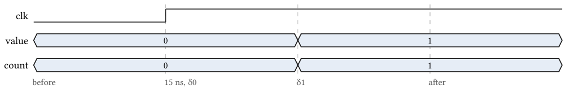
Figure 4: The clock edge at 15 ns in Counter , one column per delta cycle. The simulator confirms it: a process woken by value changing already sees the new count .
