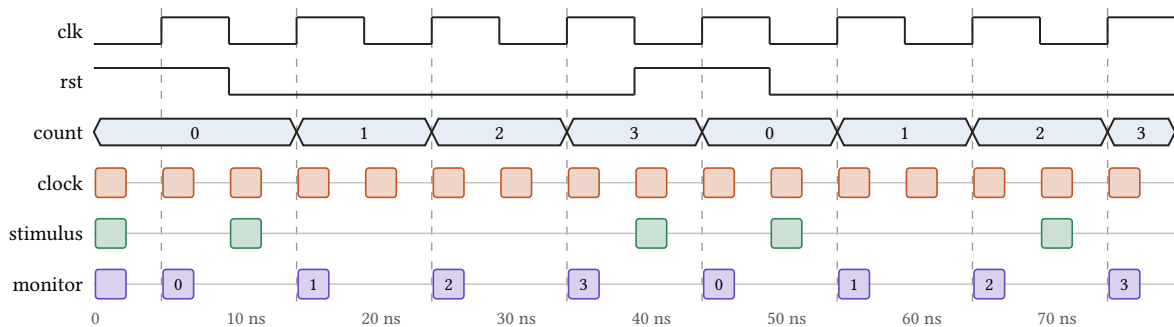
Figure 5: CounterTest with three processes, simulated. The upper rows are the VCD; each lower row marks the moments a process ran, between which it was suspended in an await . The monitor's marks carry the count it printed. All three share one host thread; at a shared time they run in a fixed order, so a run always reproduces.
