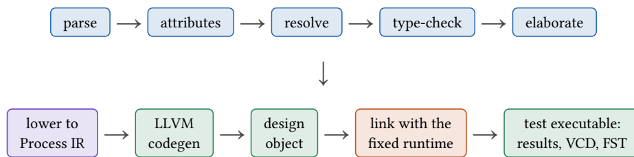
Figure 6: The pipeline. The front end produces one checked instance tree; hardware and testbench processes alike become Process IR; the native code links with a runtime that is the same for every design.
