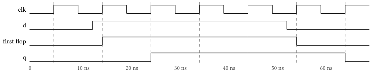
Figure 8: std::sync::Sync2 in simulation: an input that changes between clock edges (13 ns) is taken by the first flop on the next edge and reaches q one edge later, so q only ever changes on an edge of clk .
