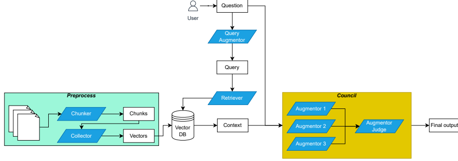
Fig. 1 Overview of the proposed RAG-based pipeline. During preprocessing, documents are segmented into chunks by the Chunker. The Collector encodes each chunk into a dense vector and indexes it in the vector database. At inference time, a user question is first reformulated by a query-enhancement model, which generates one or more retrieval queries. The Retriever performs top- k similarity search over the vector index and aggregates the retrieved passages into a supporting context. The original question and the retrieved context are then provided to the Council, i.e., an ensemble of role-specialized generative models producing candidate answers. Finally, a Judge model validates these candidates and outputs the final response.
