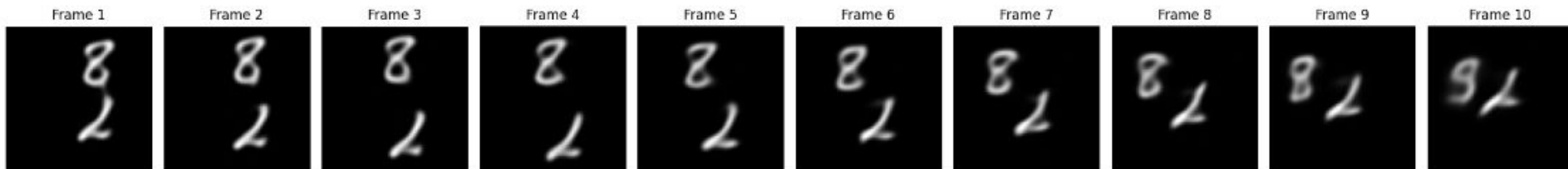
Predicted Frames
