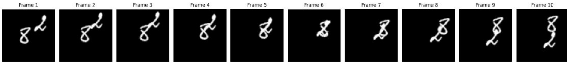
Target Frames
