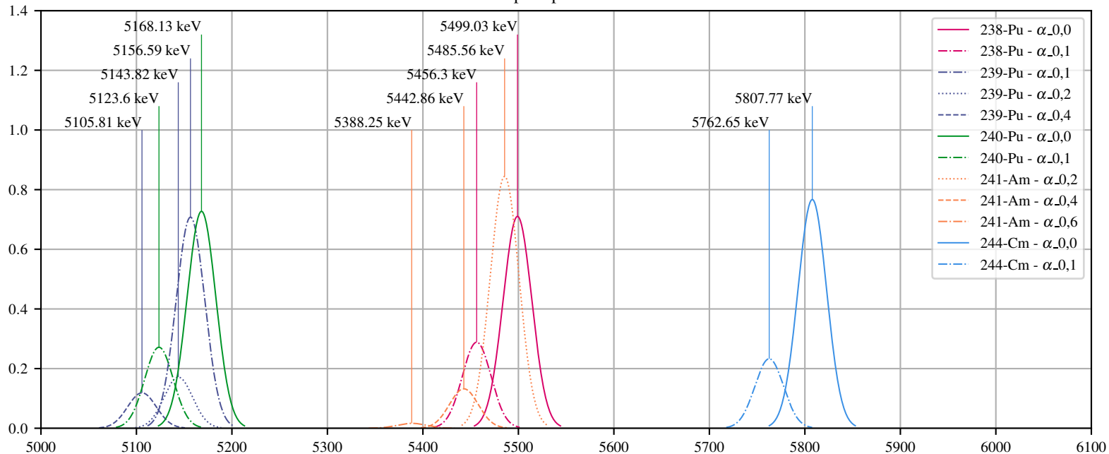
Harwell source alpha spectrum - FWHM = 15 keV
