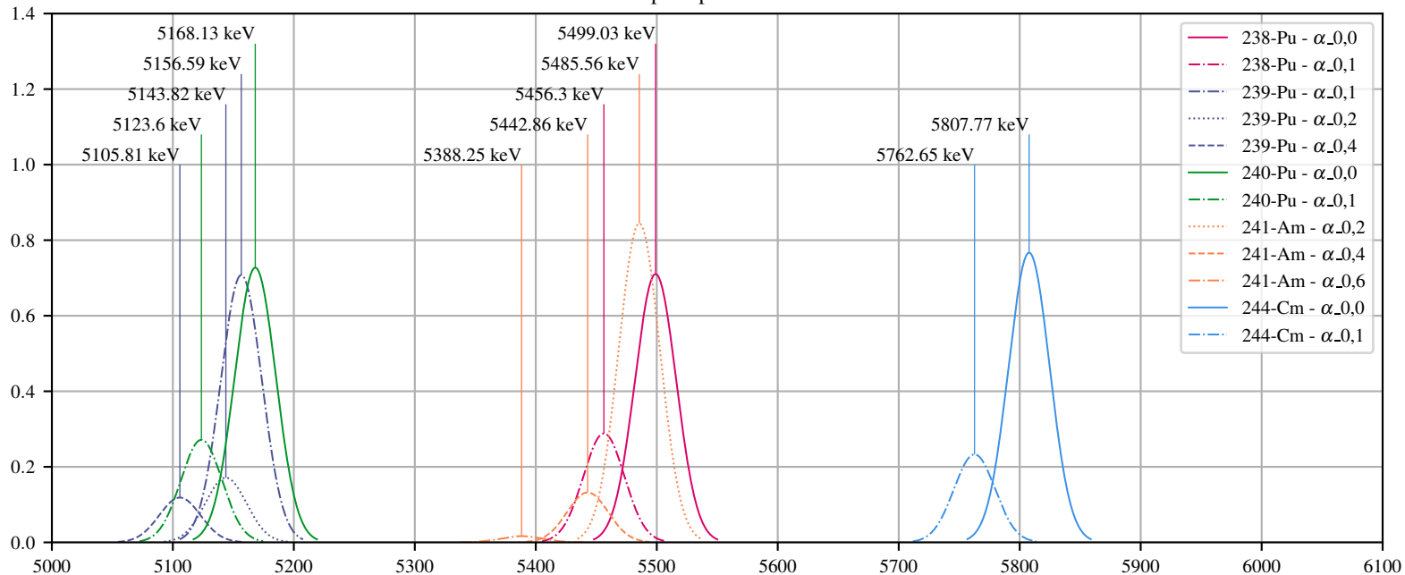
Harwell source alpha spectrum - FWHM = 17 keV
