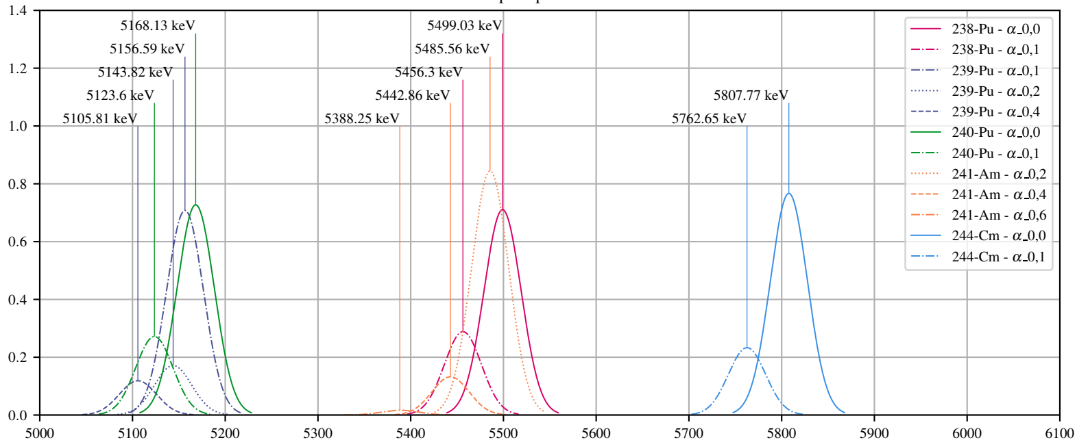
Harwell source alpha spectrum - FWHM = 20 keV
