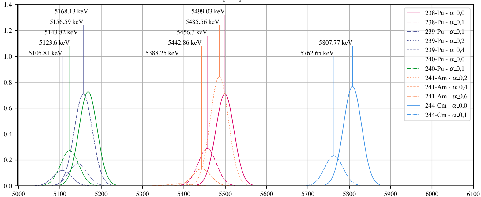
Harwell source alpha spectrum - FWHM = 22 keV
