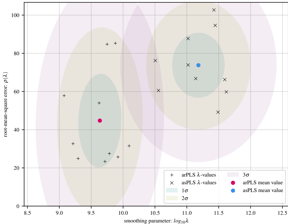
10 simulations of sine baseline with 8 Gaussians and 30 dB noise
