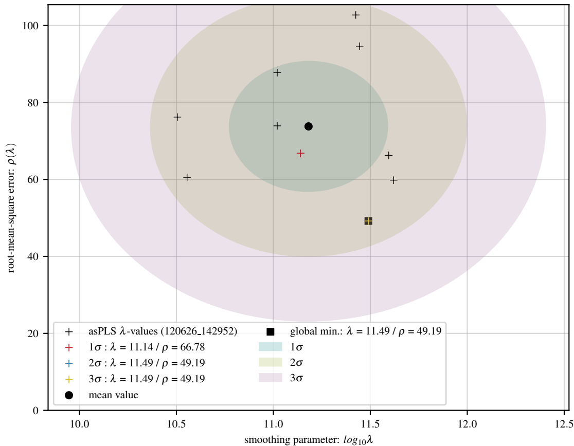
10 asPLS fits of sine baseline with 8 Gaussians and 30 dB noise
