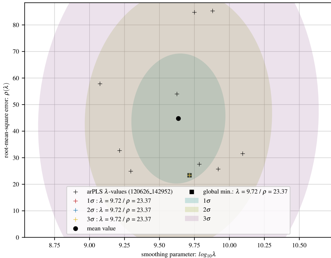
10 arPLS fits of sine baseline with 8 Gaussians and 30 dB noise
