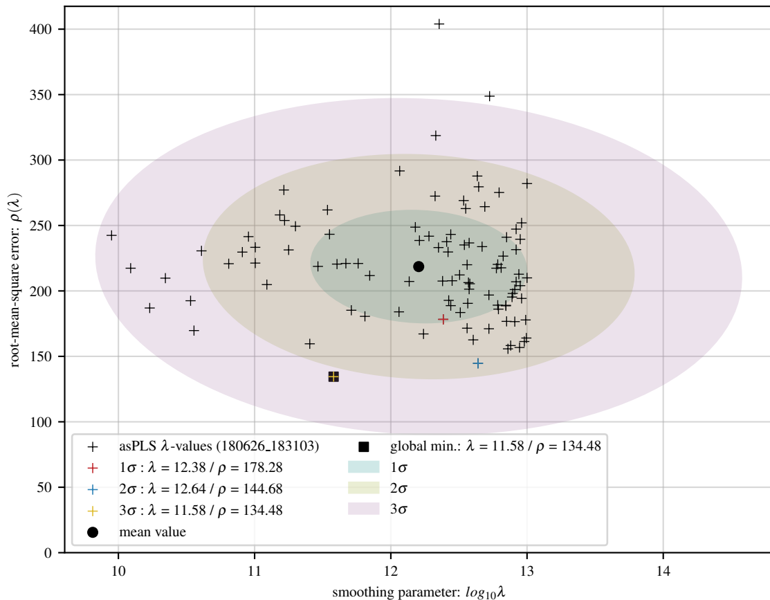
100 asPLS fits of lin baseline with 8 Gaussians and 20 dB noise
