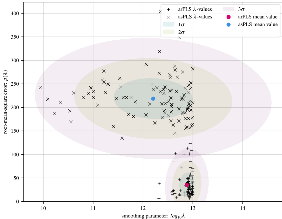
100 simulations of lin baseline with 8 Gaussians and 20 dB noise
