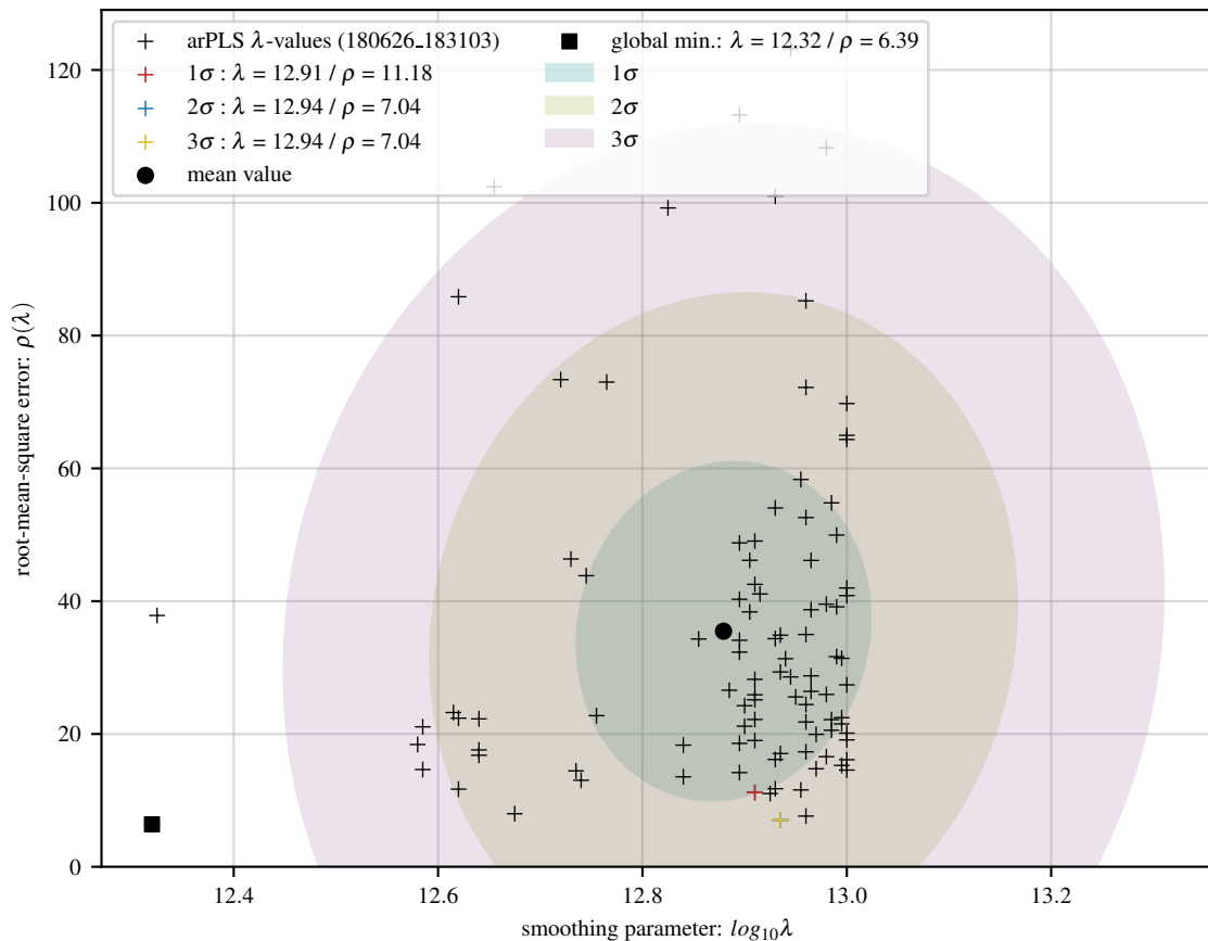
100 arPLS fits of lin baseline with 8 Gaussians and 20 dB noise
