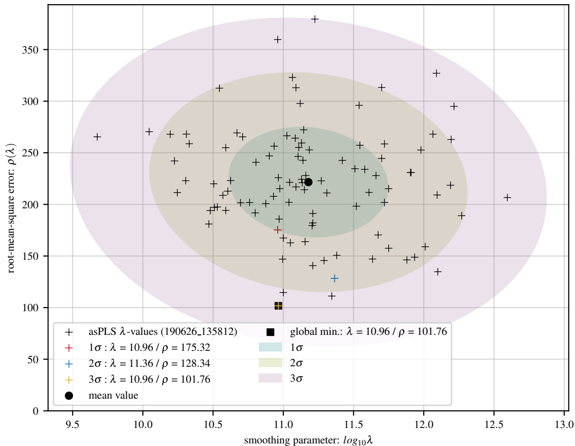
100 asPLS fits of sine baseline with 8 Gaussians and 20 dB noise
