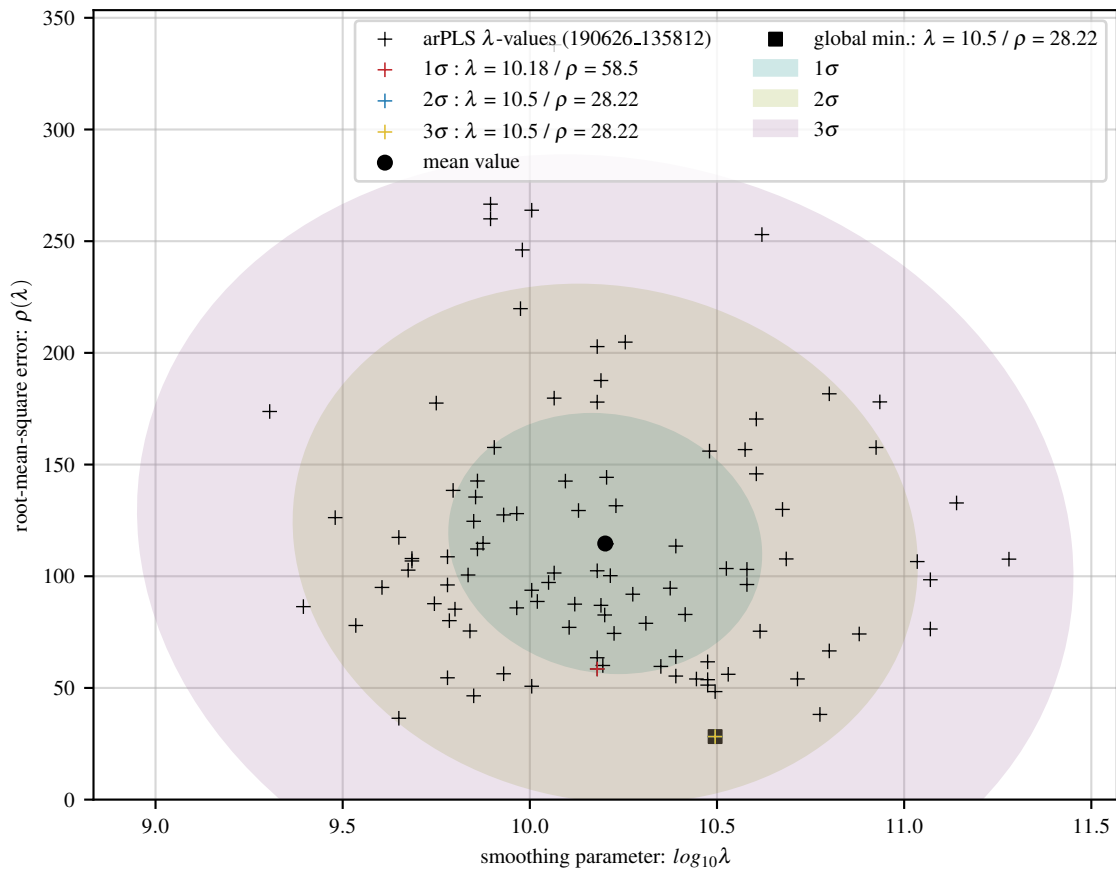
100 arPLS fits of sine baseline with 8 Gaussians and 20 dB noise
