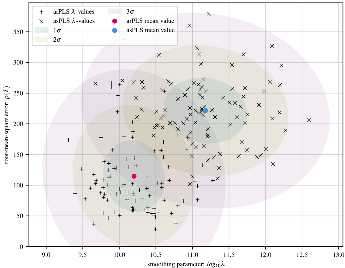
100 simulations of sine baseline with 8 Gaussians and 20 dB noise
