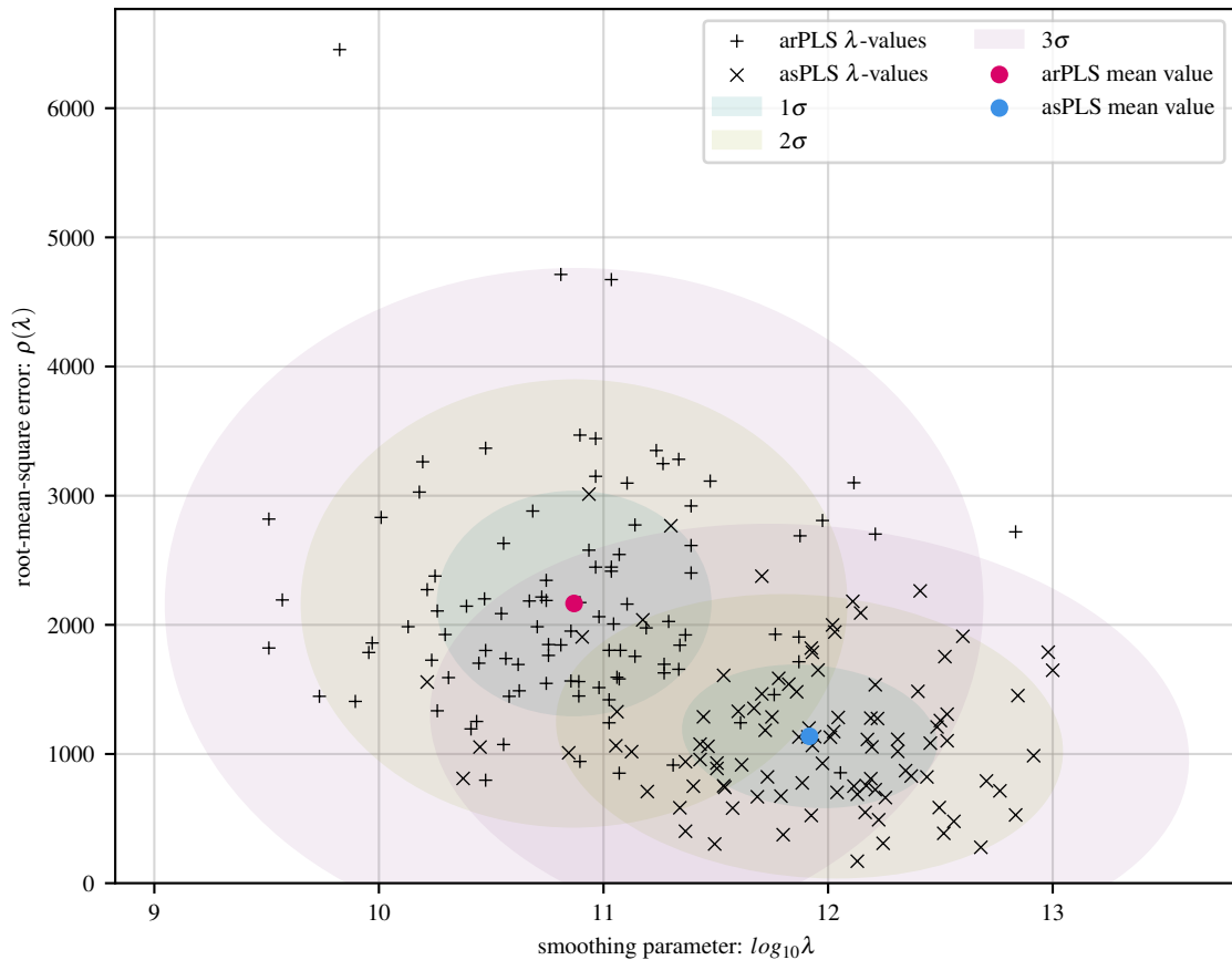
100 simulations of sine baseline with 40 Gaussians and 20 dB noise
