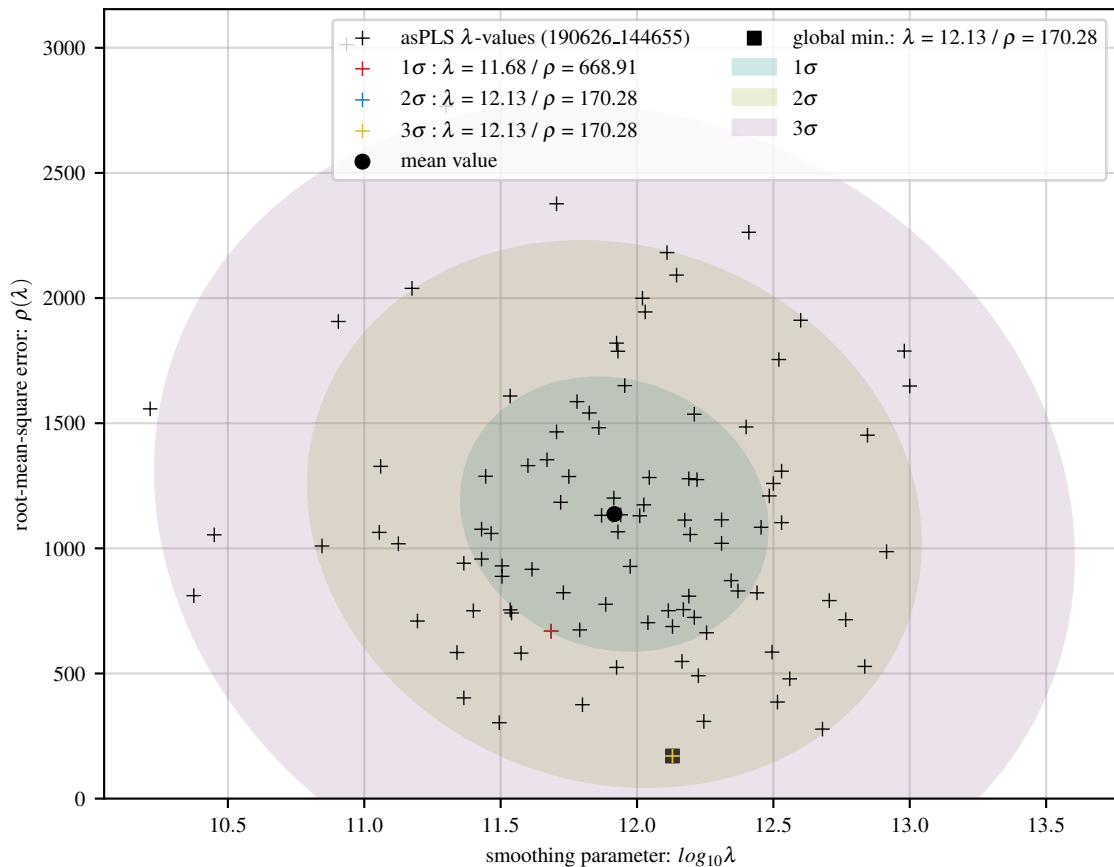
100 asPLS fits of sine baseline with 40 Gaussians and 20 dB noise
