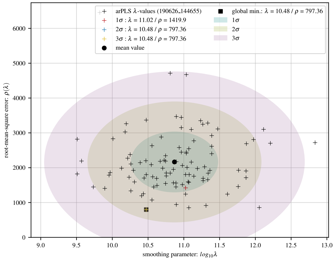
100 arPLS fits of sine baseline with 40 Gaussians and 20 dB noise
