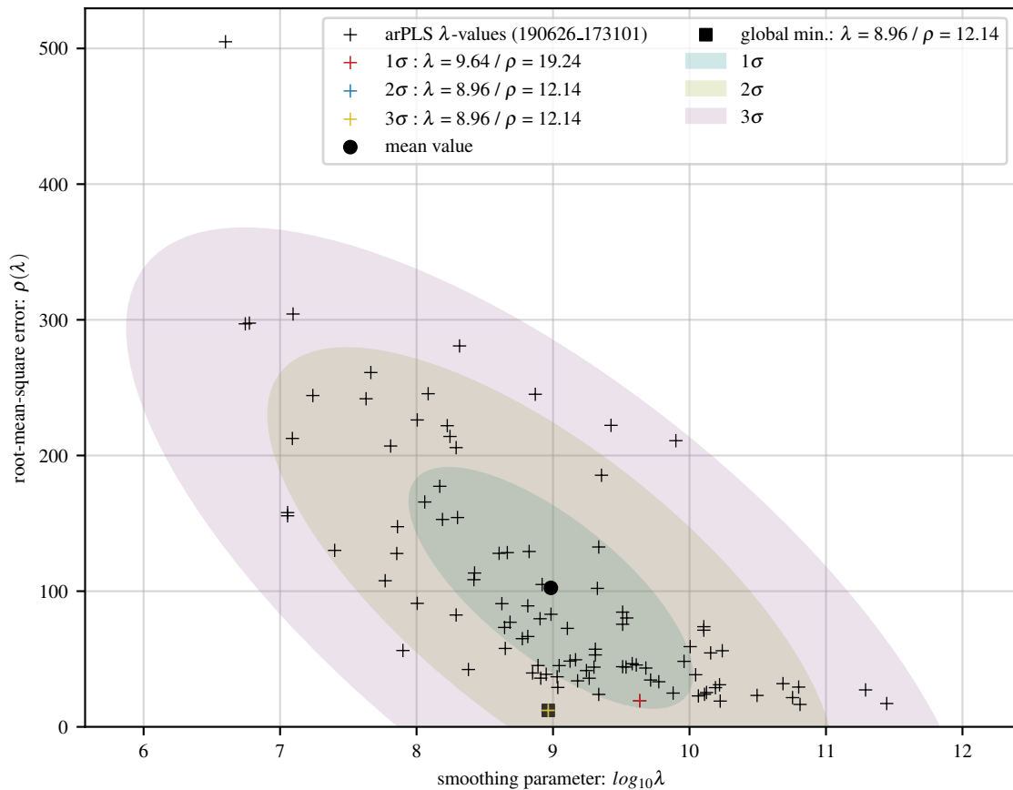
100 arPLS fits of exp baseline with 8 Gaussians and 30 dB noise
