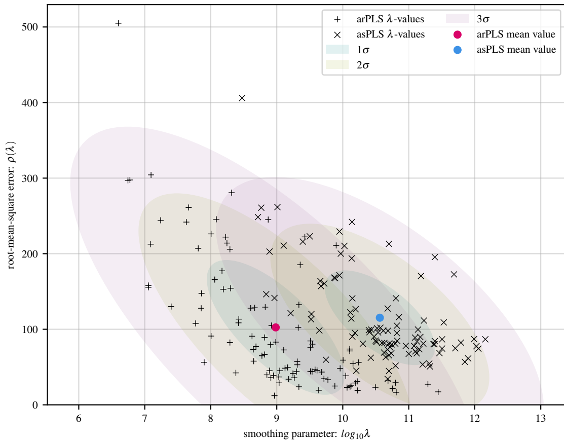
100 simulations of exp baseline with 8 Gaussians and 30 dB noise
