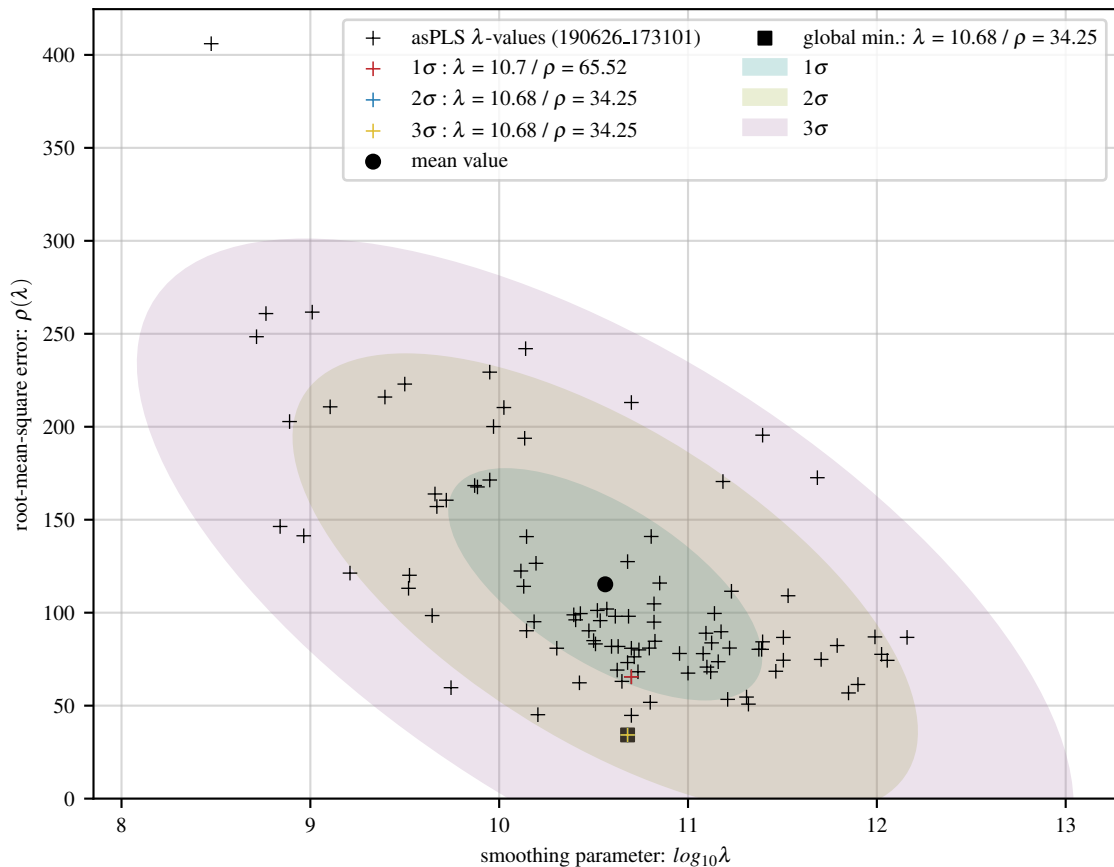
100 asPLS fits of exp baseline with 8 Gaussians and 30 dB noise
